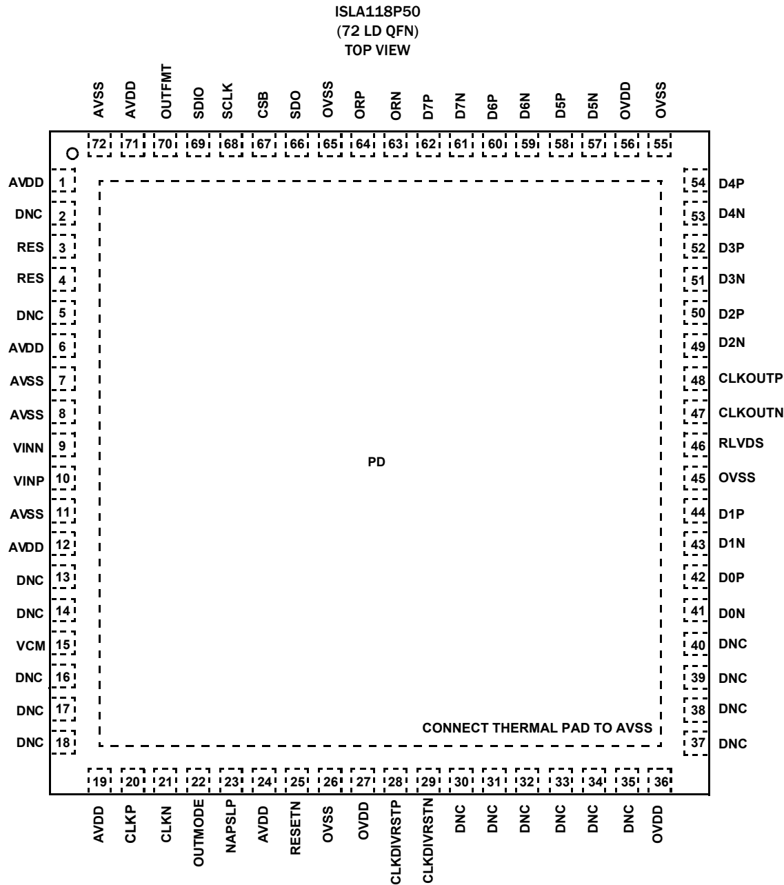
FIGURE 2. PIN CONFIGURATION
