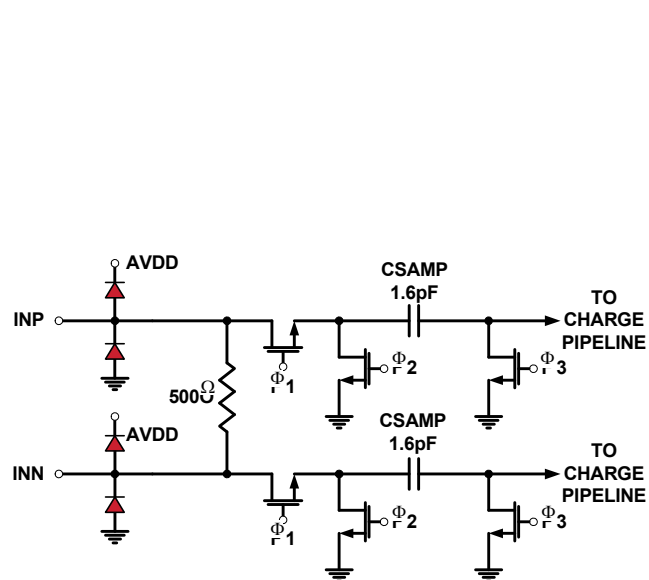
FIGURE 47. ANALOG INPUTS
