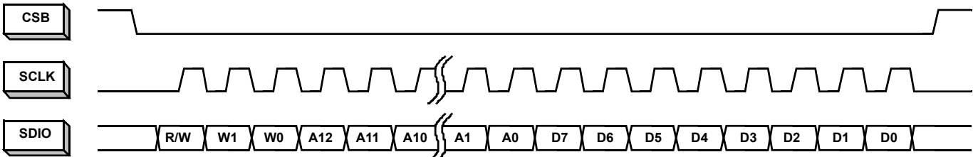
FIGURE 39. MSB-FIRST ADDRESSING
