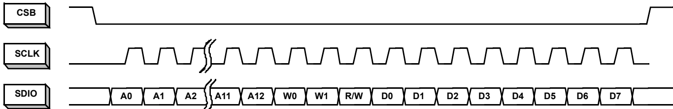
FIGURE 40. LSB-FIRST ADDRESSING
