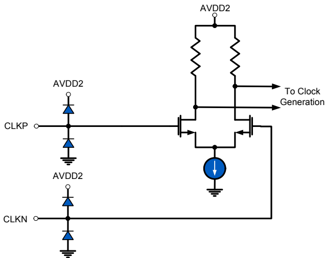
FIGURE 29. CLOCK INPUTS
