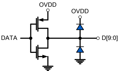
FIGURE 30. LVCMOS OUTPUT
