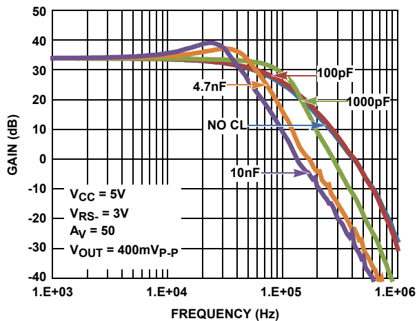
FIGURE 35. CAPACITIVE LOAD DRIVE GAIN vs FREQUENCY
