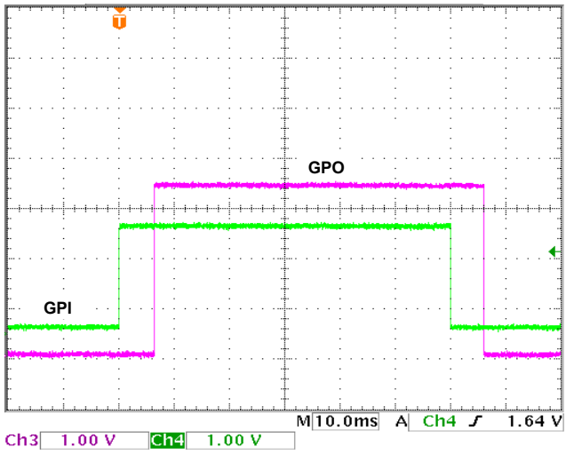
FIGURE 19. GPI TO GPO FUNCTIONALITY
