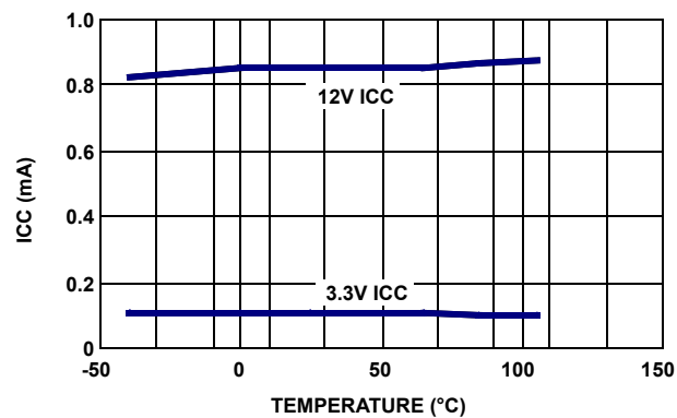
FIGURE 22. ICC CURRENT vs TEMPERATURE
