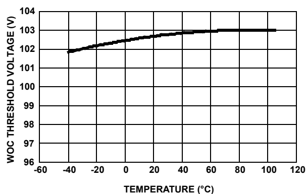
FIGURE 24. FAST TRIP THRESHOLD VOLTAGE vs TEMPERATURE
