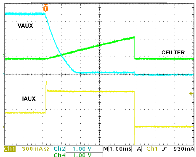
FIGURE 17. VAUX WOC REGULATION AND SHUTDOWN
