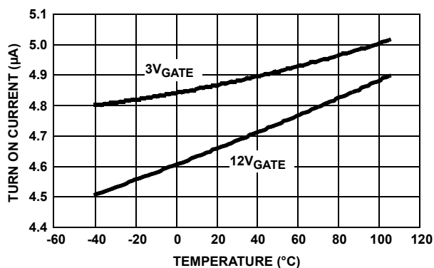
FIGURE 32. ISL6114 GATE TURN-ON CURRENT (ABS) vs TEMPERATURE
