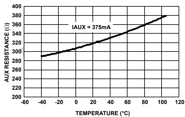
FIGURE 26. AUX r_{DS(ON)} vs TEMPERATURE
