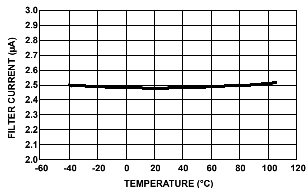
FIGURE 34. FILTER CHARGE CURRENT vs TEMPERATURE
