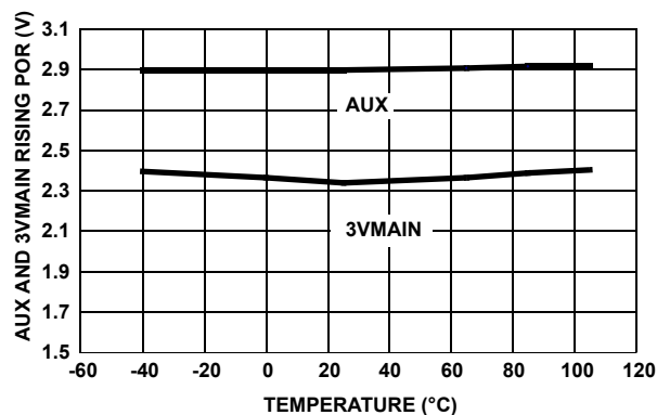
FIGURE 28. AUX AND 3VMAIN RISING POR THRESHOLD VOLTAGE vs TEMPERATURE
