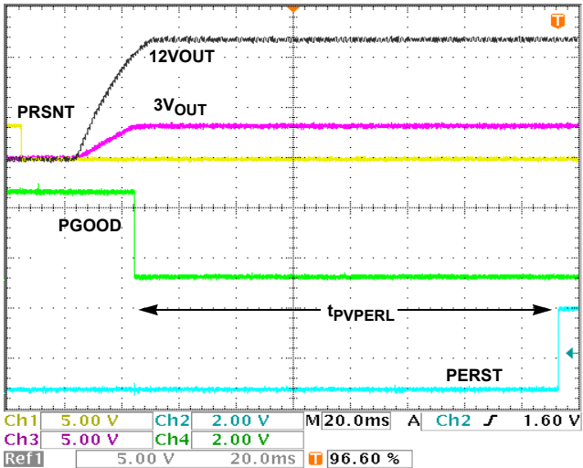
FIGURE 18. PRSNT, V_{OUT} , POWERGOOD, PERST
