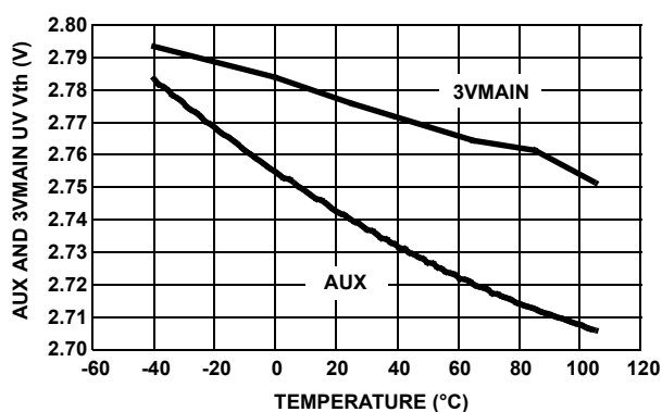
FIGURE 30. AUX AND 3VMAIN POWER GOOD THRESHOLD VOLTAGE vs TEMPERATURE
