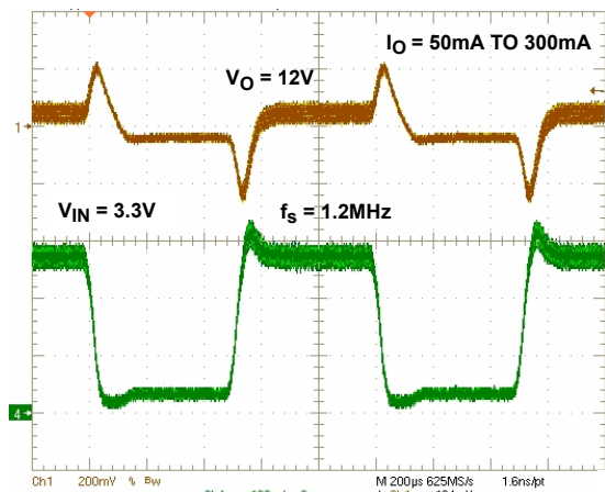
FIGURE 7. TRANSIENT RESPONSE
