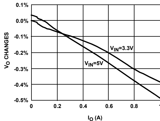
FIGURE 4. LOAD REGULATIONS
