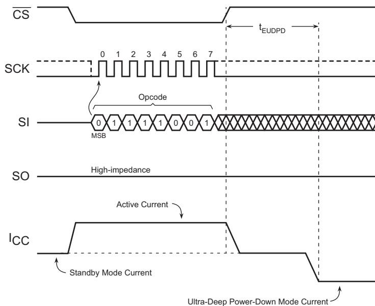
Figure 7-5. Entering Ultra-Deep Power Down State
