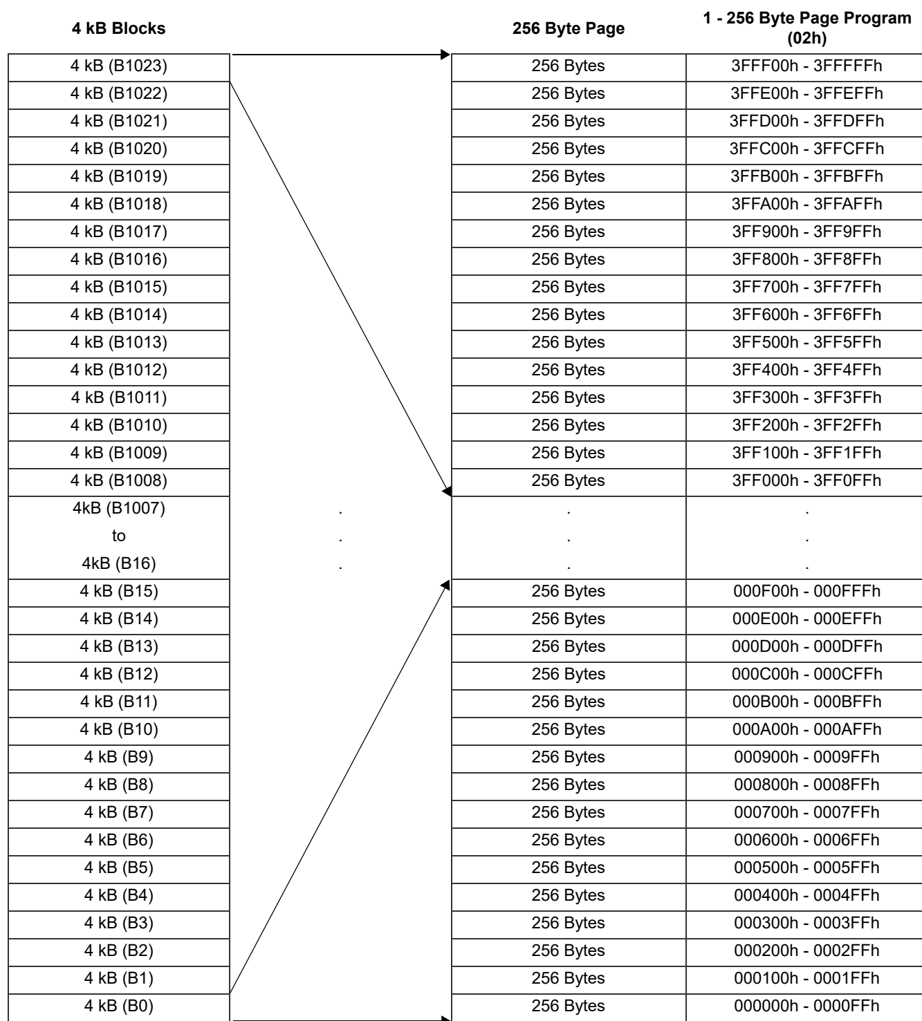
Figure 5-17. AT25FF321A Device Block Memory Map — Page Program
