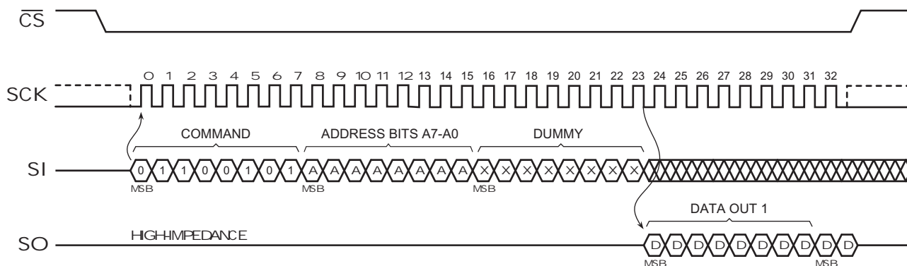
Figure 7-1. Status Register Read Operation Showing 8-bit Address Field
