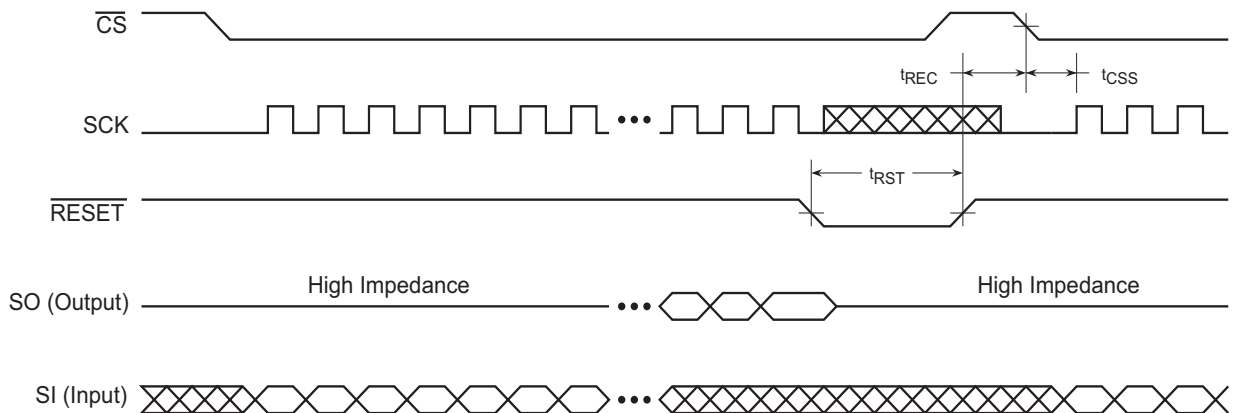
Figure 26-12. Reset Timing
