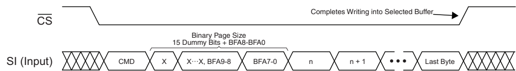
Figure 24-2. Buffer Write
