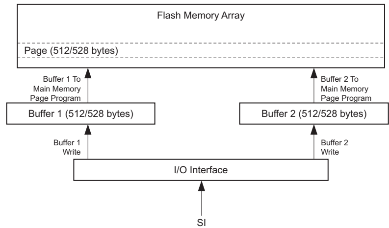
Figure 24-1. Block Diagram
