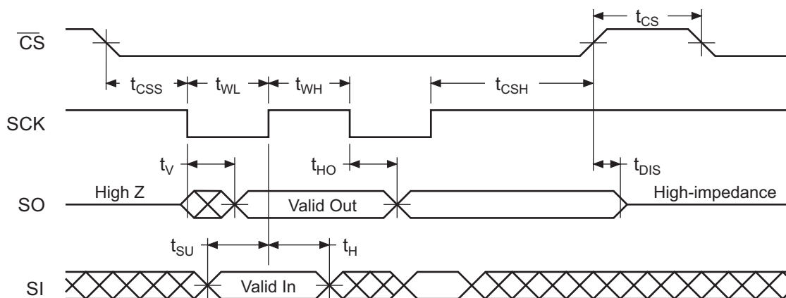
Figure 23-2. Waveform 2 = SPI Mode 3 Compatible
