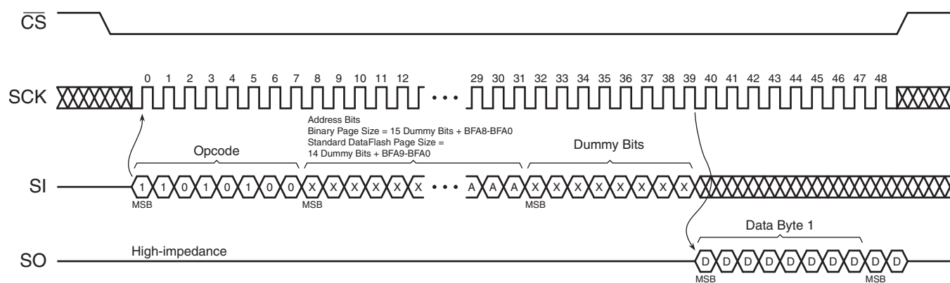
Figure 26-5. Buffer Read Timing (Opcode D4h or D6h)
