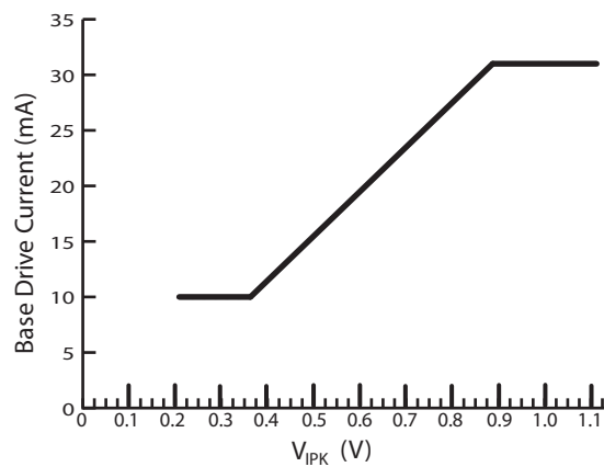
Figure 10.6: Base Drive Current vs. V_{IPK}
