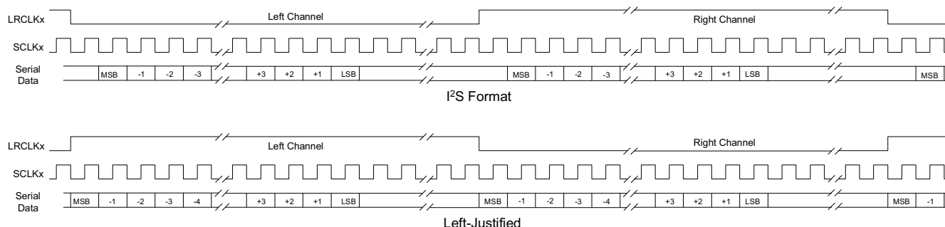
FIGURE 5. SAI PORT SUPPORTED DATA FORMATS FOR DELIVERY OF LINEAR PCM OR COMPRESSED AUDIO DATA
