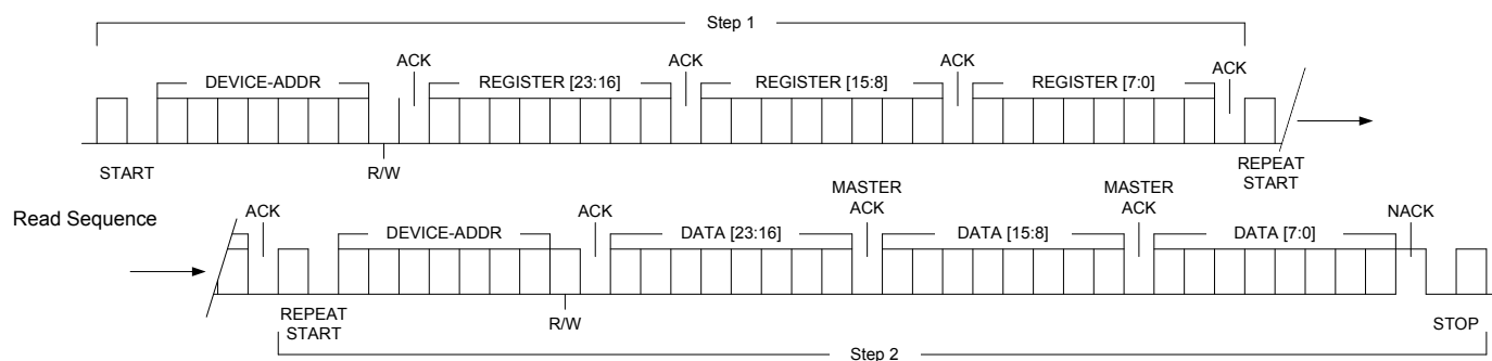
FIGURE 11. I 2 C READ SEQUENCE OPERATION
