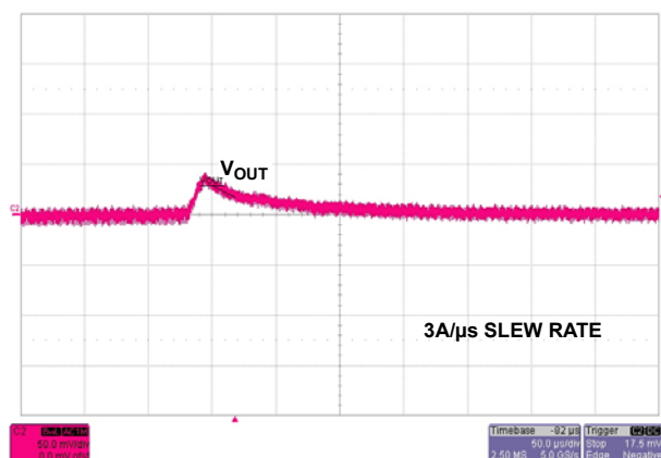
FIGURE 12. LOAD TRANSIENT (48A TO 0A STEP)
