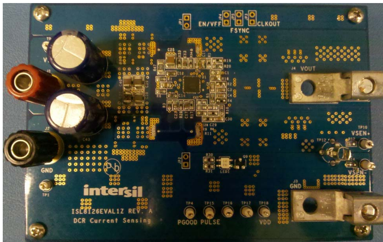
FIGURE 1. ISL8126EVAL1Z EVALUATION BOARD
