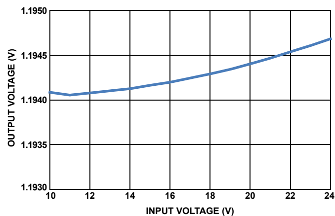
FIGURE 7. LINE REGULATION
