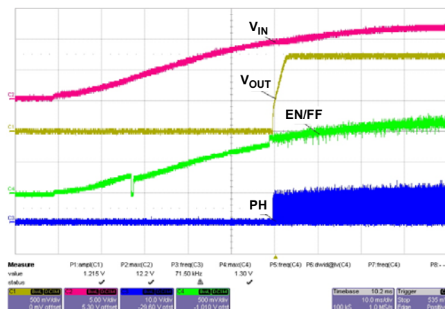
FIGURE 6. POWER-UP UNDER 50A LOAD
