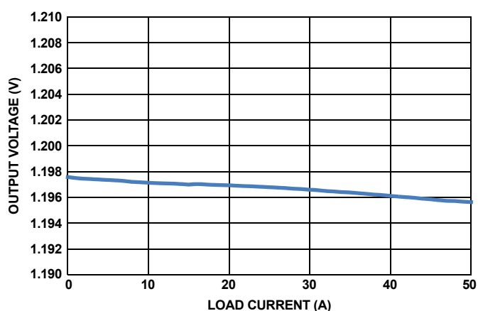
FIGURE 8. LOAD REGULATION
