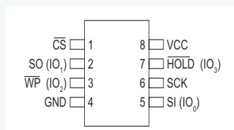
Figure 2-1. 8-SOIC (0.150" and 0.208") — Top View
