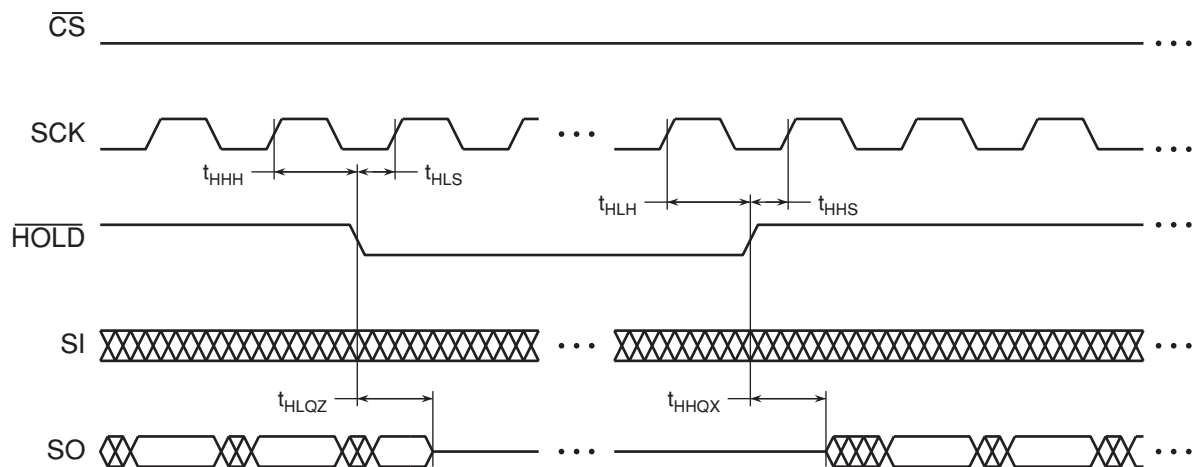
Figure 8-14. \overline{\text{HOLD}} Timing – Serial Output
