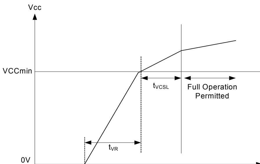
Figure 8-8. AC Timing During Device Power Up
