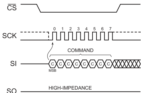
Figure 5-1. SPI Transfer — Command Only
