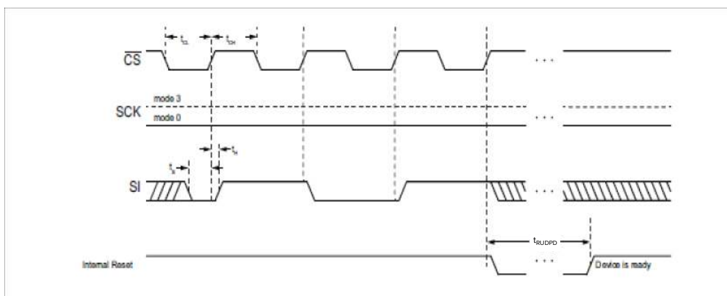
Figure 5-20. JEDEC Standard Hardware Reset
