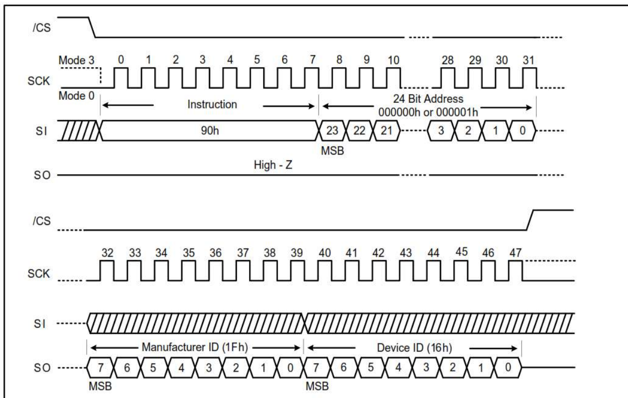
Figure 7-41. Read Manufacturer/ Device ID Instruction (SPI Mode)
