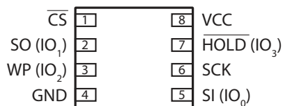
Figure 1-2. 8-UDFN (Top View)
