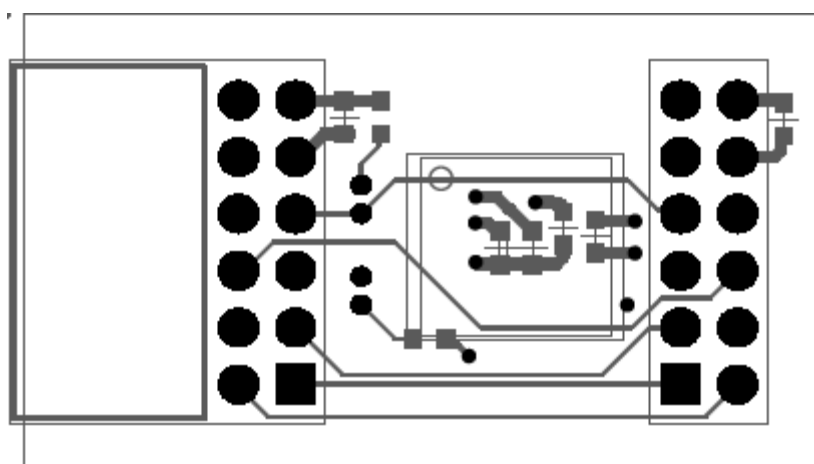
Figure 9. Copper Bottom
