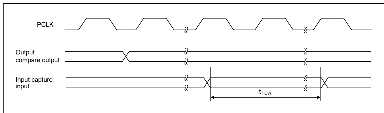
Figure 2.35 MTU Input/Output Timing
