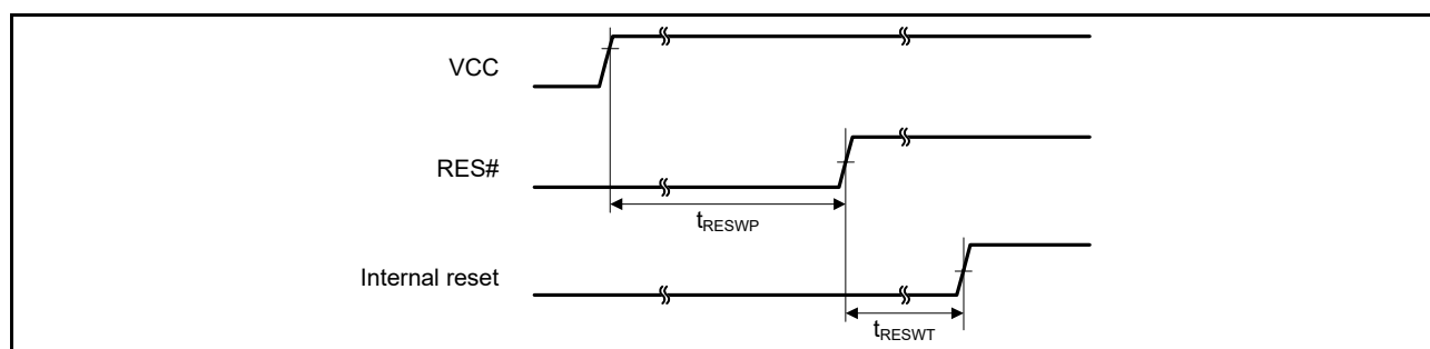
Figure 2.27 Reset Input Timing at Power-On
