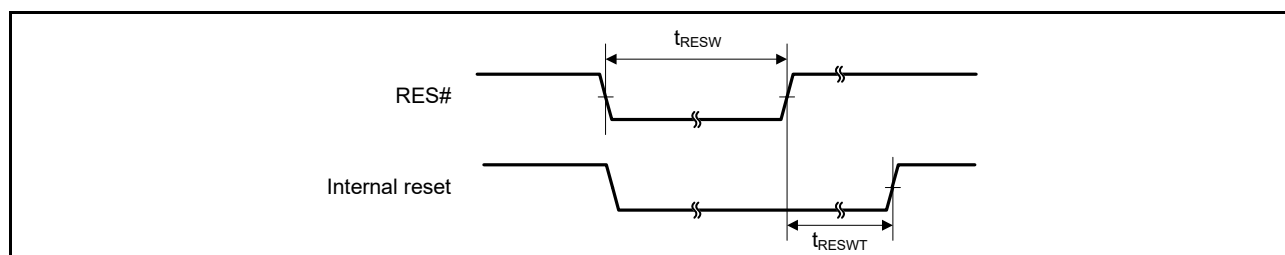
Figure 2.28 Reset Input Timing (1)
