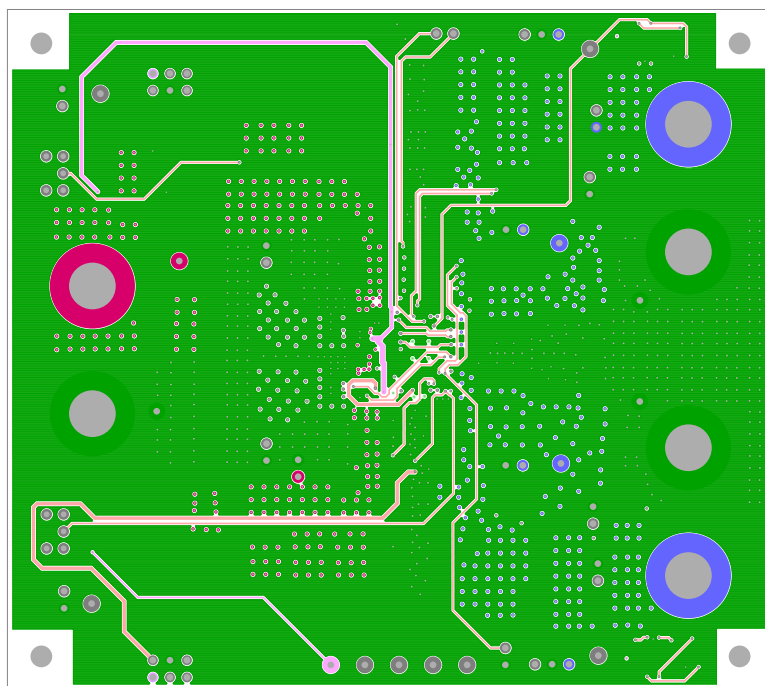
Figure 16. Layer 5
