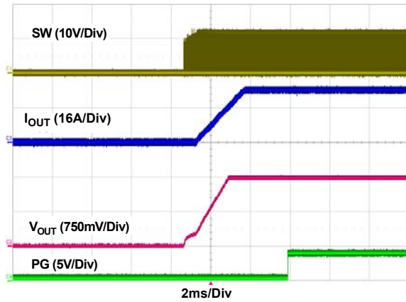
Figure 27. Single Channel Startup 12V_{IN} , 1.5V_{OUT} , 25A
