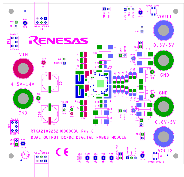
Figure 11. Silkscreen Top
