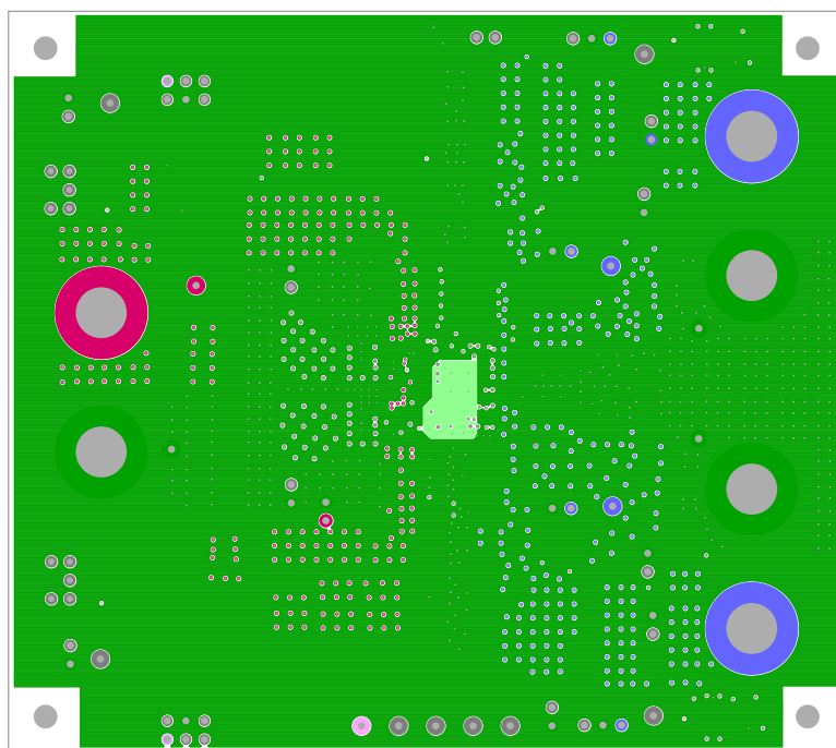
Figure 17. Layer 6
