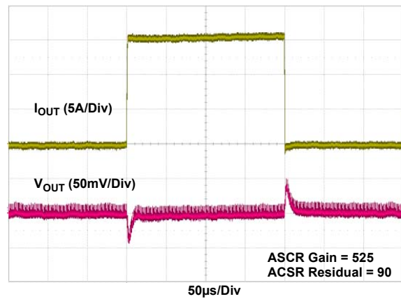
Figure 30. 0A - 15A, 12V_{IN} , 1.5V_{OUT} , 889kHz
