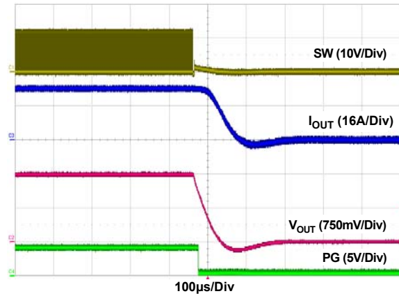
Figure 28. Single Channel Shutdown 12V_{IN} , 1.5V_{OUT} , 25A
