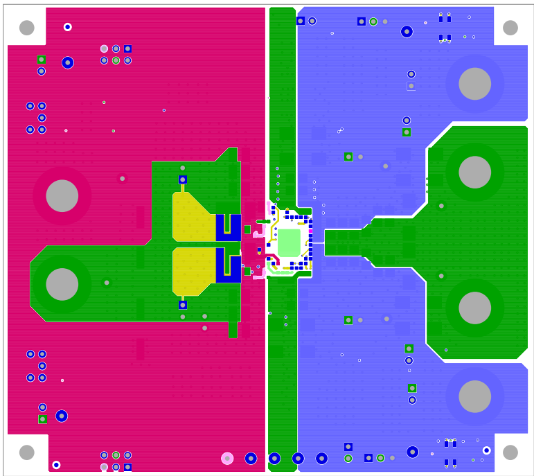
Figure 12. Top Layer
