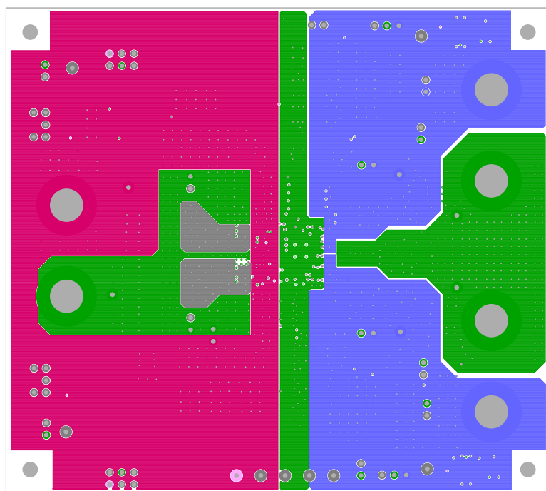
Figure 18. Layer 7
