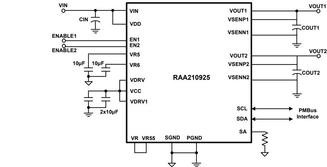
Figure 1. RTKA2109252H00000BU Block Diagram
