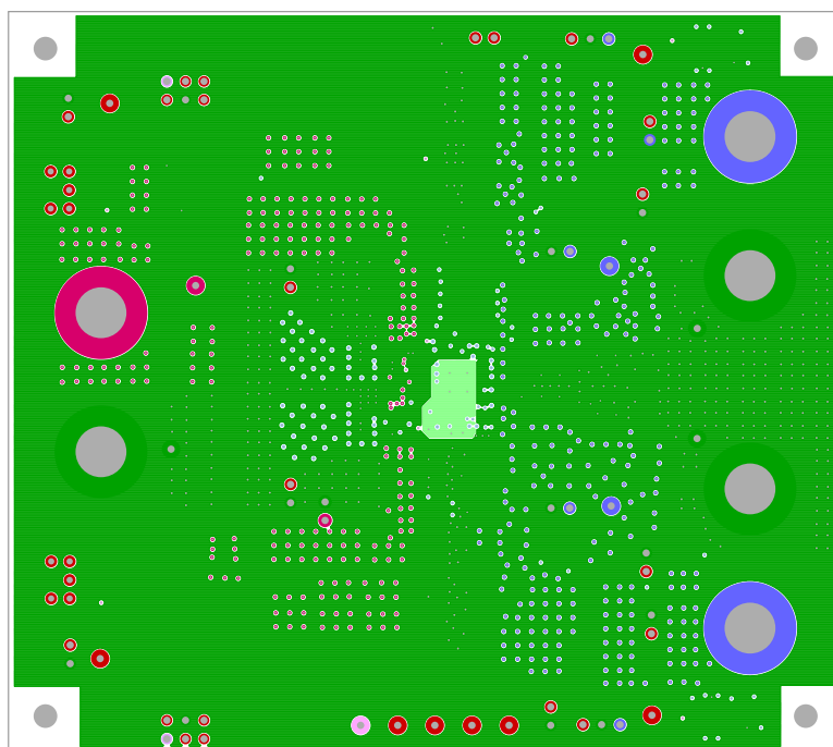
Figure 14. Layer 3
