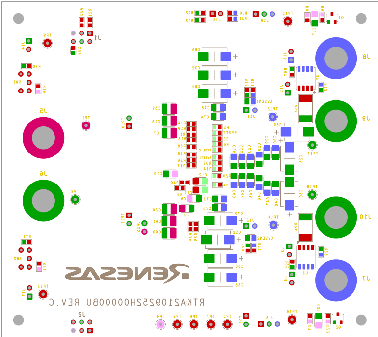
Figure 20. Silkscreen Bottom
