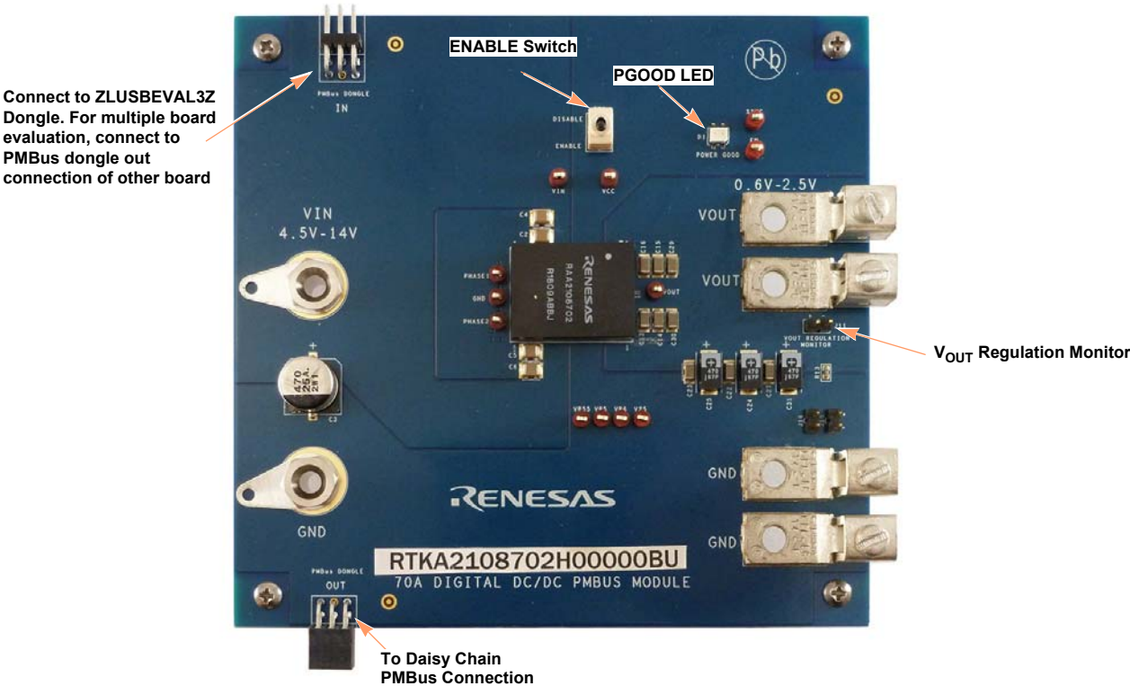
Figure 5. RTKA2108702H00000BU Evaluation Board (Top Side)
