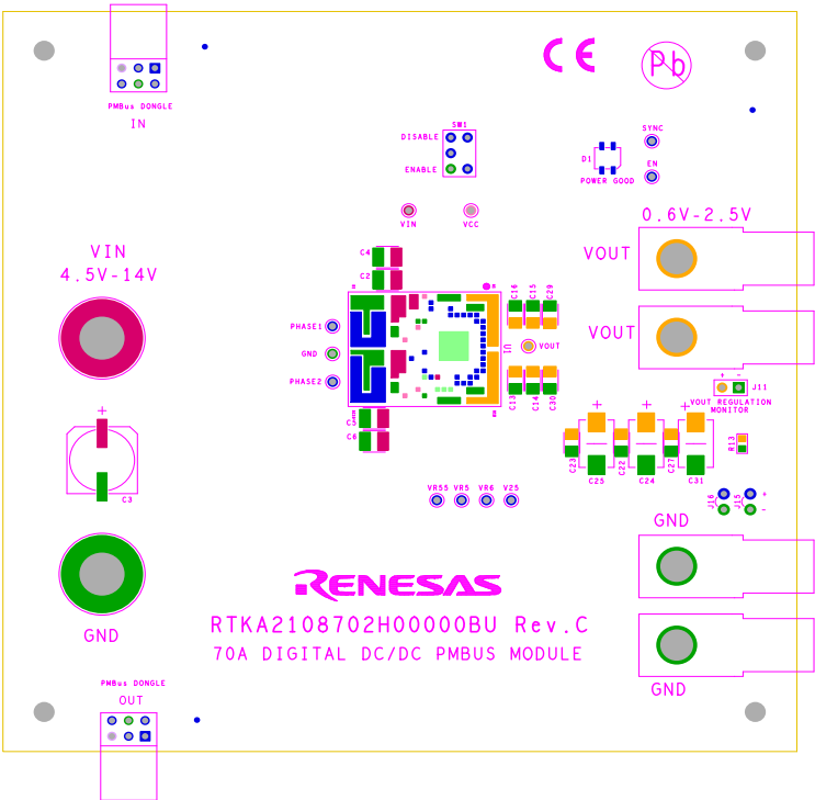
Figure 8. Silkscreen Top
