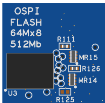
Figure 25. Octo-SPI Flash
