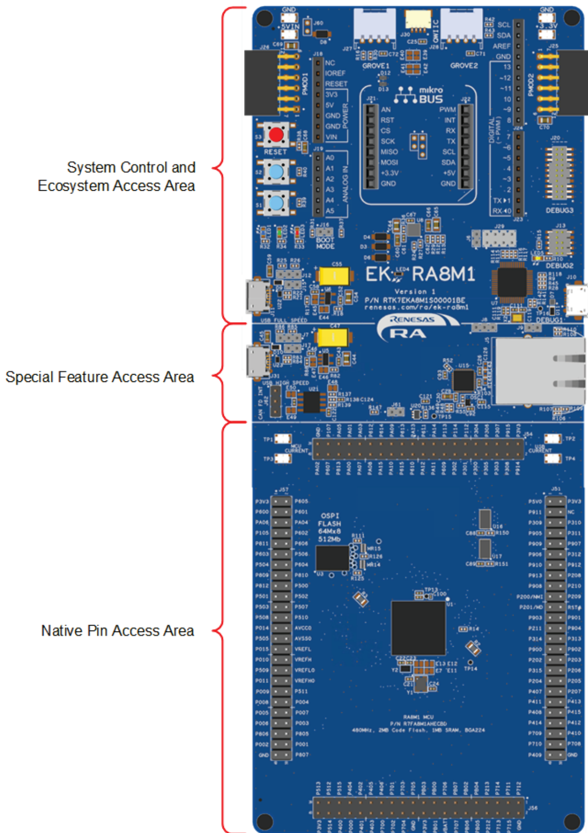
Figure 4. EK-RA8M1 Board Functional Area Definitions
