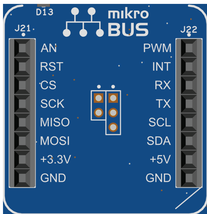
Figure 15. mikroBUS Connection
