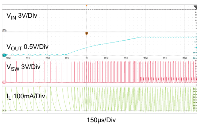
Figure 15. Recovery from Short-Circuit and startup to Full Load
