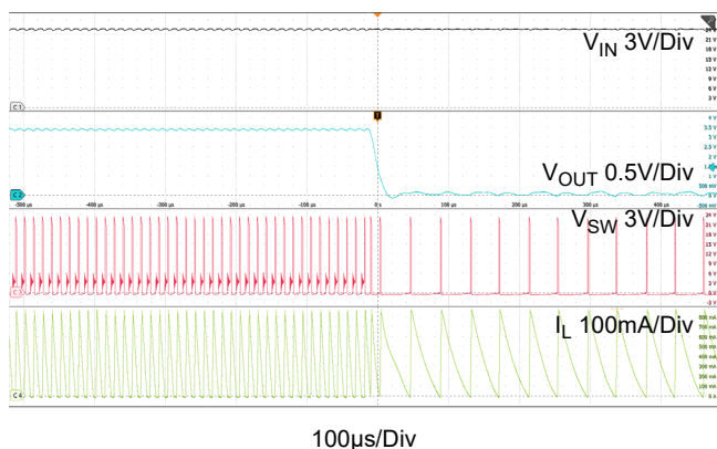
Figure 14. Short-Circuit
