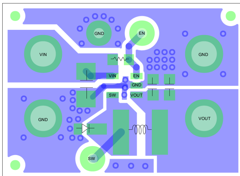
Figure 7. Top Layer
