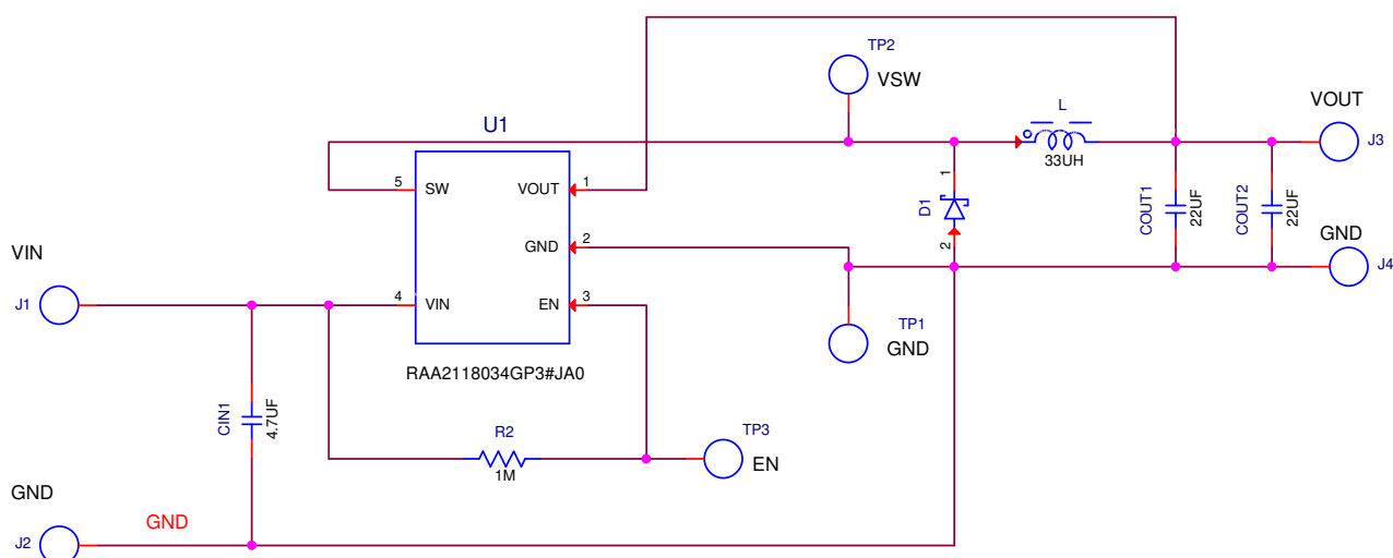
Figure 5. RTKA211803DE0000BU Schematic
