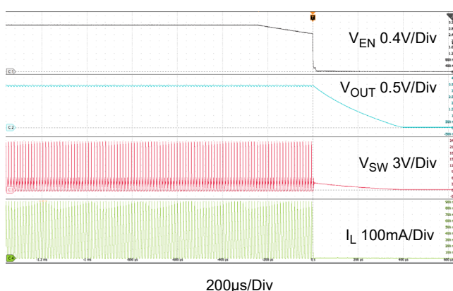
Figure 13. Shutdown through EN
