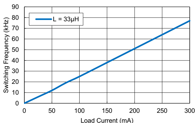
Figure 3. Switching Frequency ( V_{IN} = 24V ) vs. Load Current
