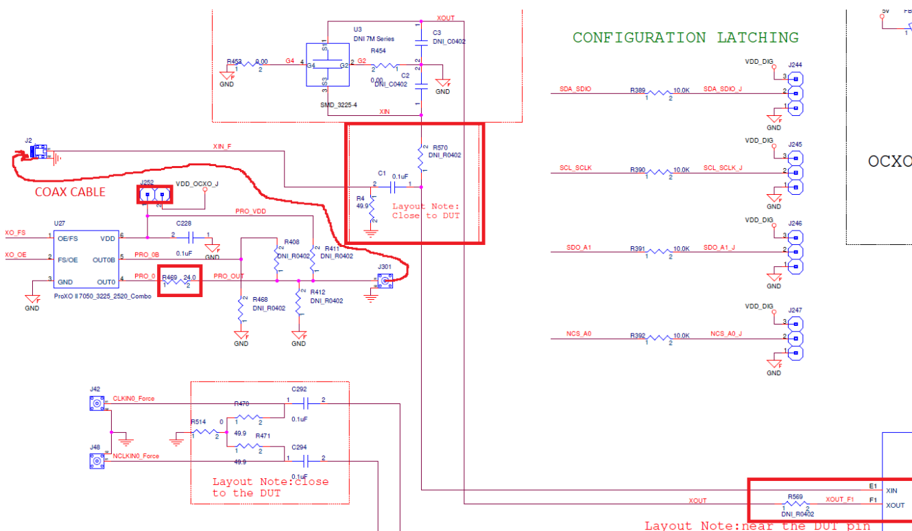
5. Set the DIP switch SW1 S7 and S8 to pull the XO output enable pin high or low depending on the XO datasheet. 6. If the XO is a differential output driver, check the termination requirement of the XO. The spare footprint can be used for LVPECL, LVDS, HCSL drivers. In most cases, only one side of the differential driver is required to overdrive the XIN.
