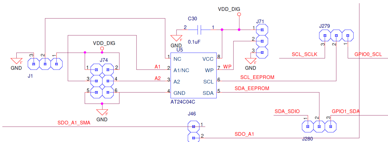
Figure 21. EEPROM Schematic
