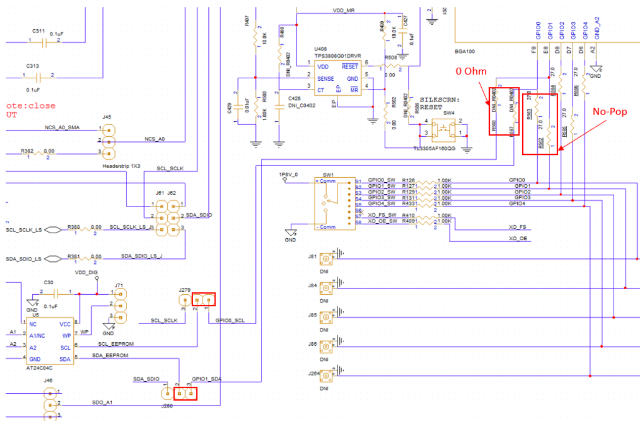
Figure 23. EEPROM Connection Jumpers for RC38312A GPIO
