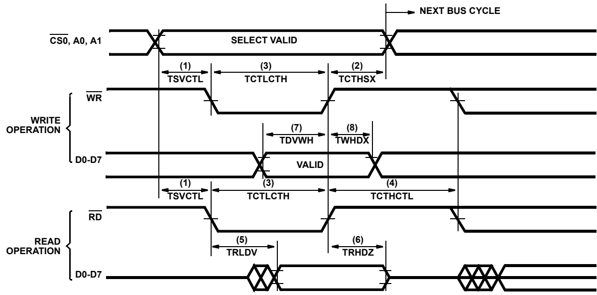
FIGURE 14. BUS OPERATION
