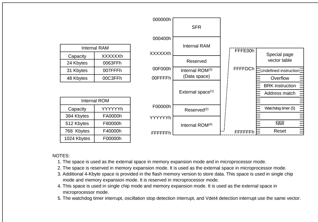
Figure 3.1 Memory Map
