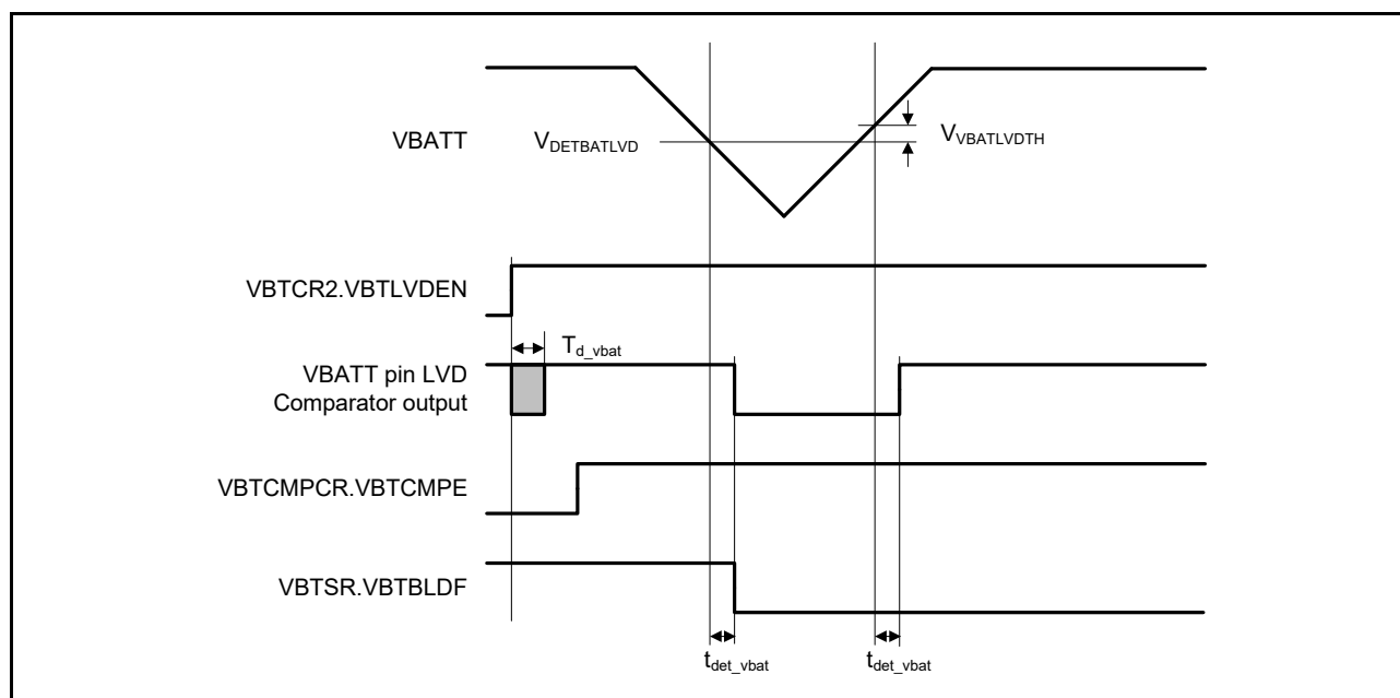
Figure 2.80 \text{VBATT} pin voltage detection circuit timing
