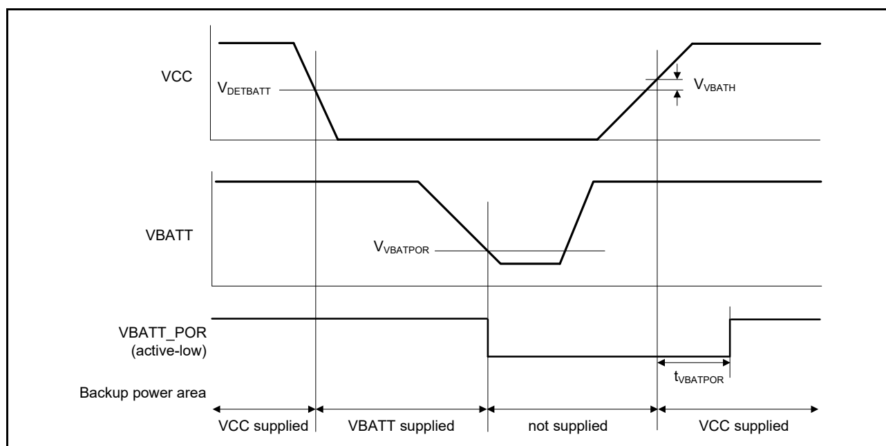
Figure 2.79 \text{VBATT\_POR} reset timing
