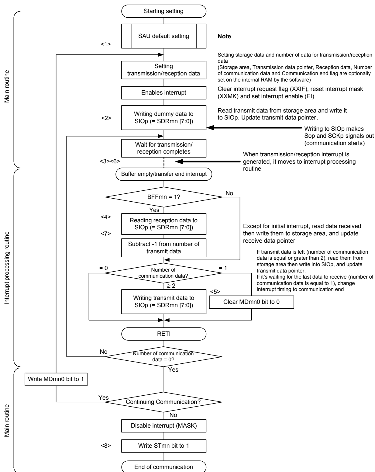
Figure 14 - 47 Flowchart of Master Transmission/Reception (in Continuous Transmission/Reception Mode)
