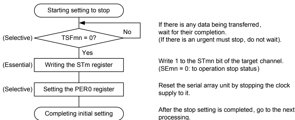
Figure 14 - 83 Procedure for Stopping UART Reception
