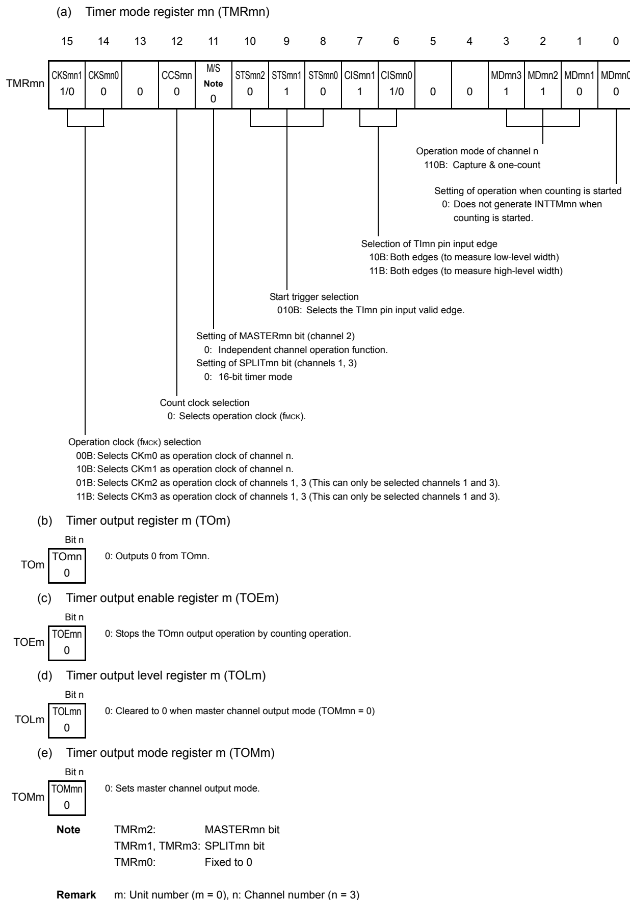
Figure 7 - 57 Example of Set Contents of Registers to Measure Input Signal High-/Low-Level Width
