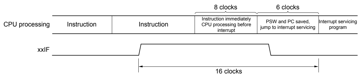
Figure 19 - 12 Interrupt Request Acknowledgment Timing (Maximum Time)
