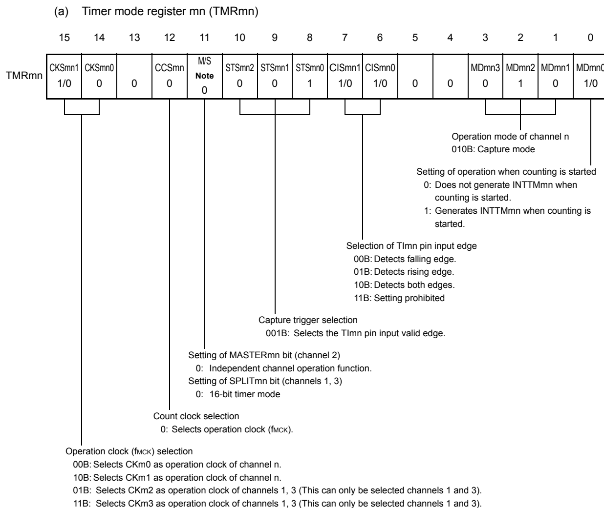
Figure 7 - 53 Example of Set Contents of Registers to Measure Input Pulse Interval
