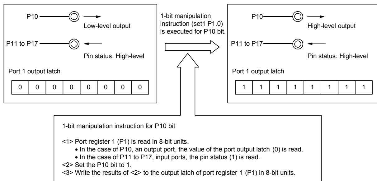
Figure 5 - 9 Bit Manipulation Instruction (P10)
