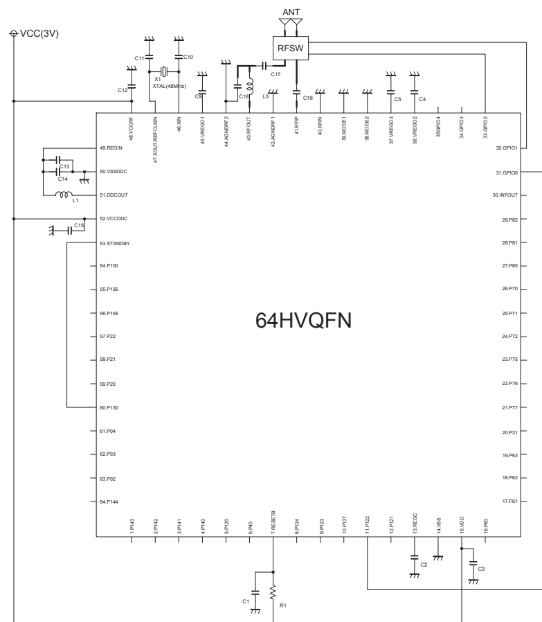
Figure 2 - 4 RL78/G1H (64-pin) Peripheral Circuits' Connection Diagram (with ANT5W)
