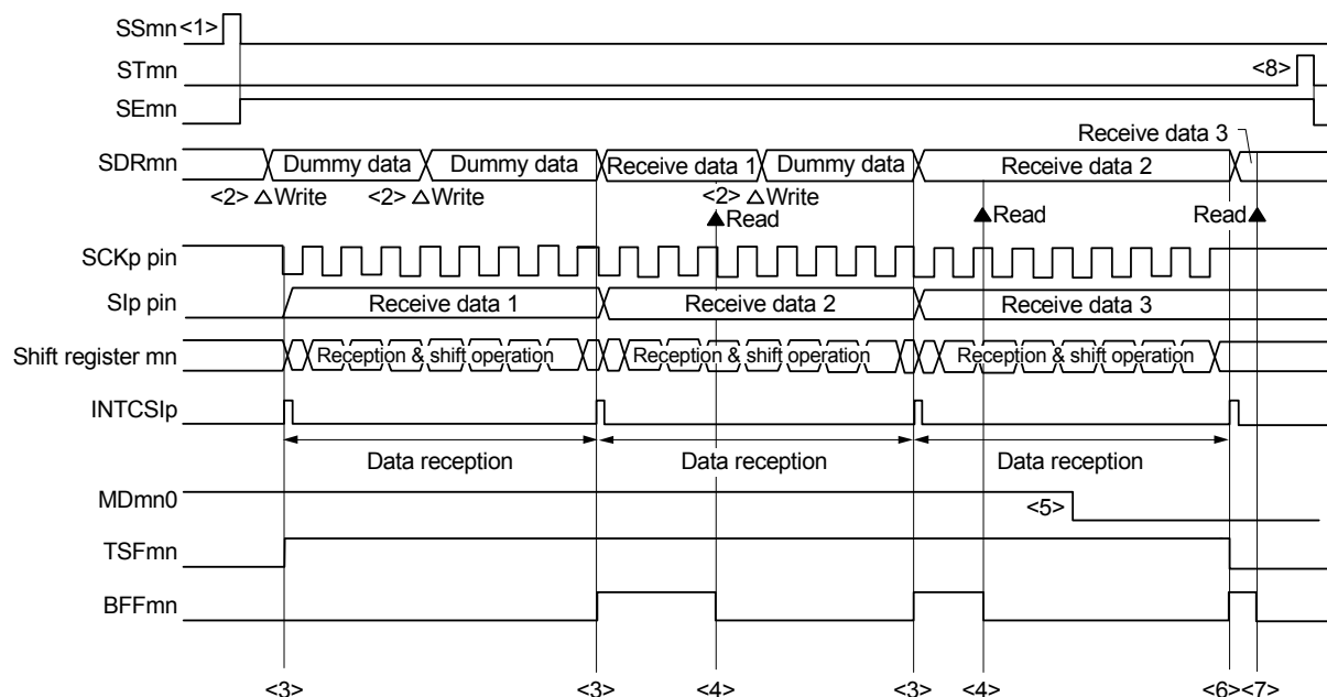
Figure 14 - 38 Timing Chart of Master Reception (in Continuous Reception Mode)
