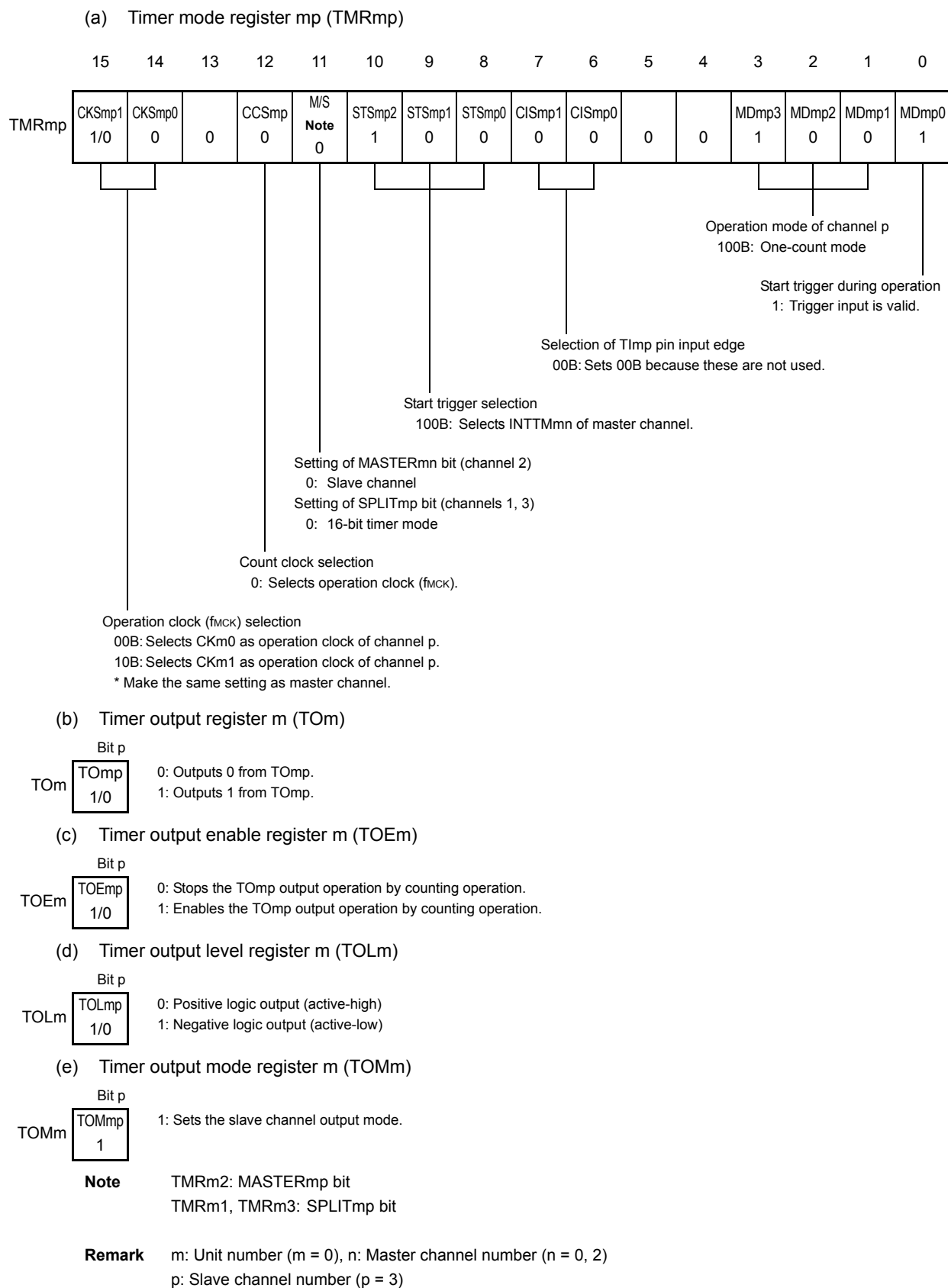
Figure 7 - 66 Example of Set Contents of Registers When PWM Function (Slave Channel) Is Used
