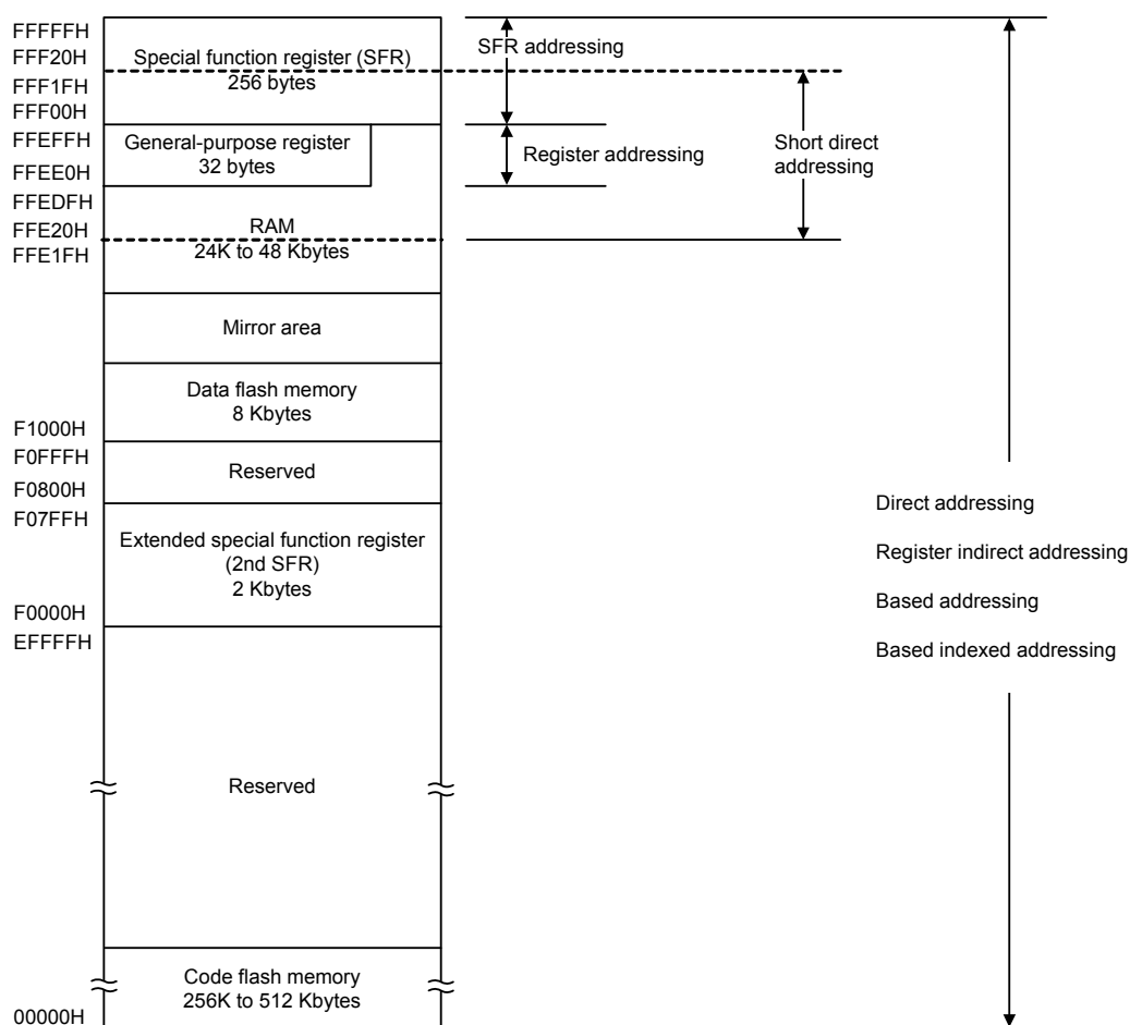
Figure 4 - 5 Correspondence Between Data Memory and Addressing
