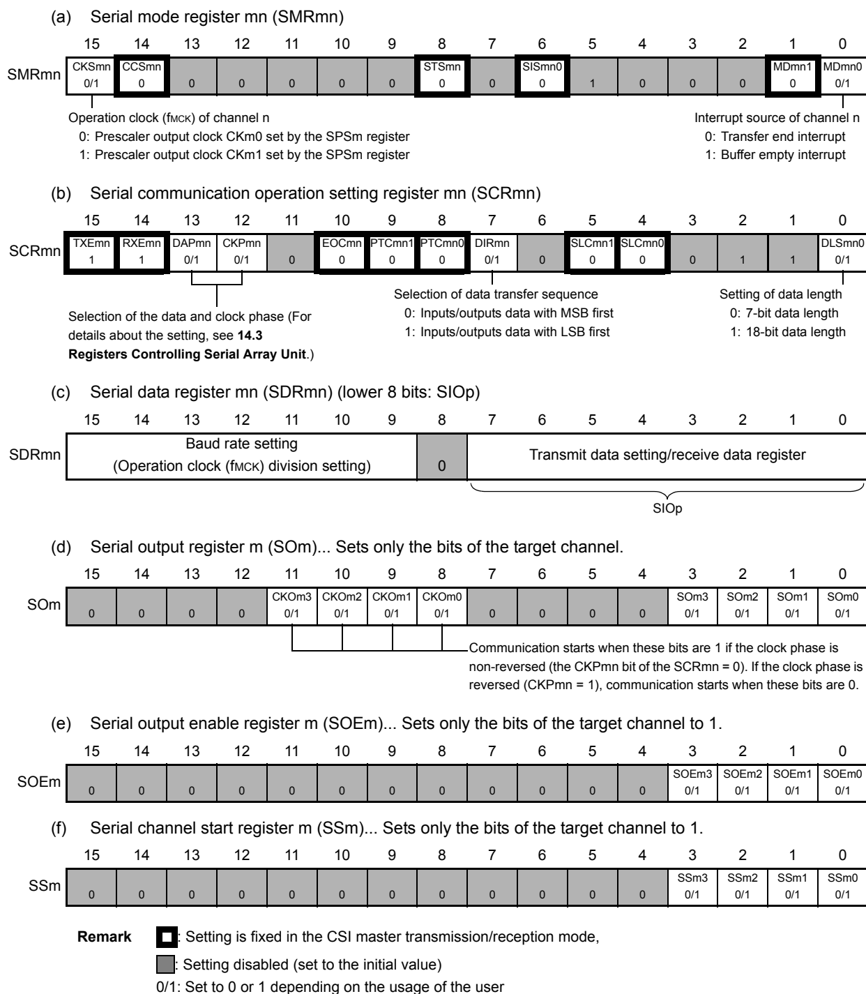
Figure 14 - 40 Example of Contents of Registers for Master Transmission/Reception of 3-Wire Serial I/O (CSIp)
