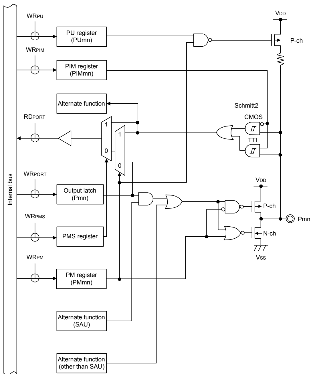
Figure 3 - 10 Pin Block Diagram of Pin Type 8-1-3
