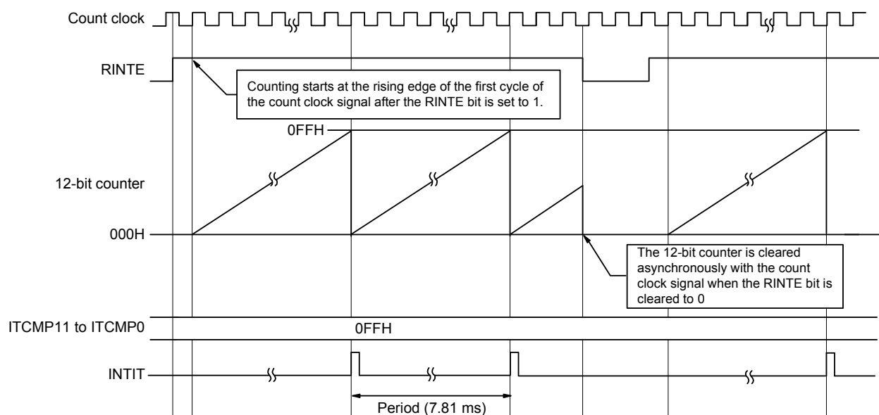
Figure 10 - 5 12-bit Interval Timer Operation Timing (ITCMP11 to ITCMP0 = 0FFH, count clock: f_{\text{sub}} = 32.768 \text{ kHz} )
