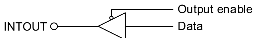
Figure 3 - 16 Pin Block Diagram of Pin INTOUT
