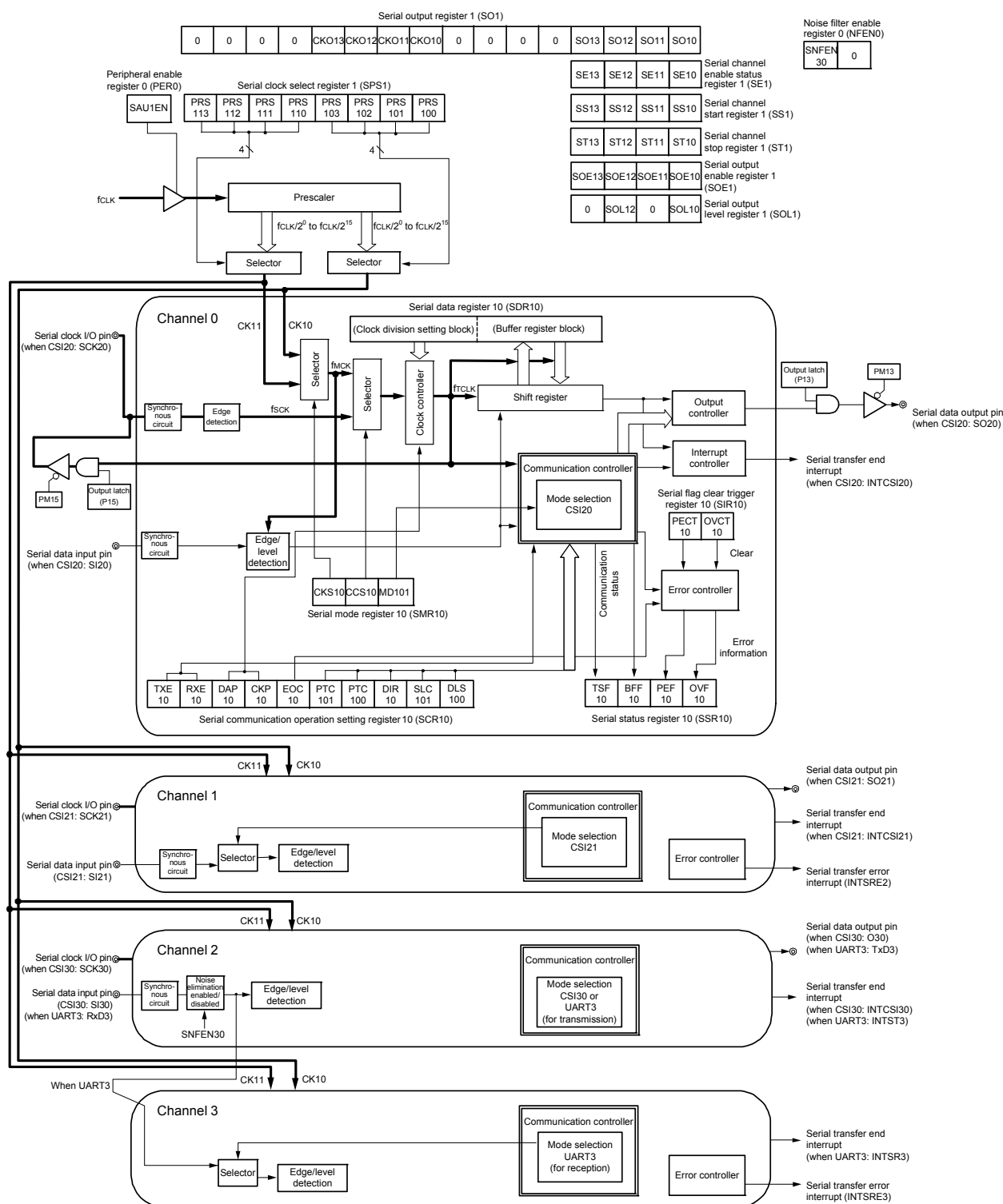
Figure 14 - 2 Block Diagram of Serial Array Unit 1
