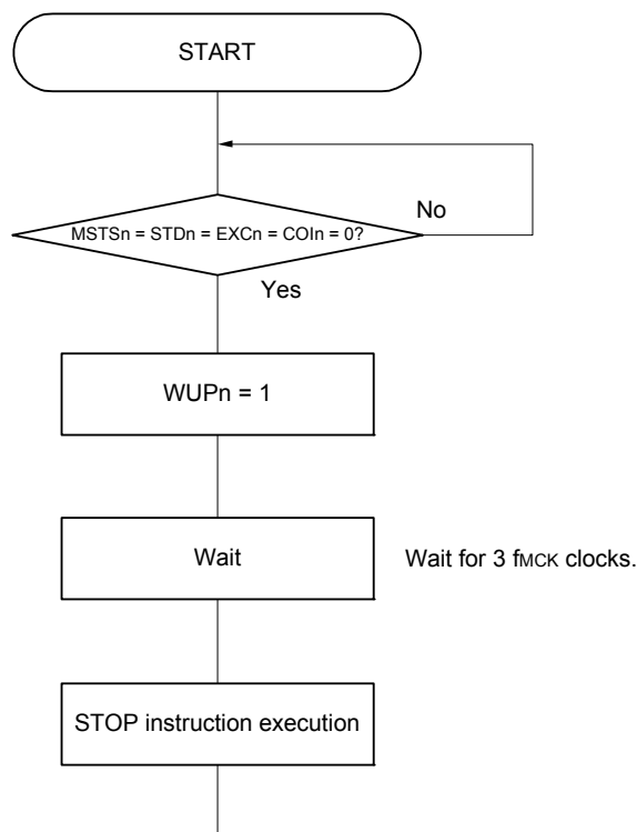
Figure 15 - 28 Flow When Setting WUPn = 1
