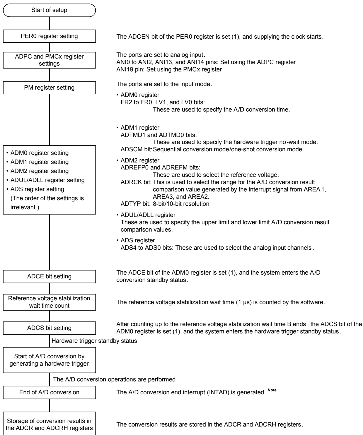
Figure 13 - 25 Setting up Hardware Trigger No-Wait Mode
