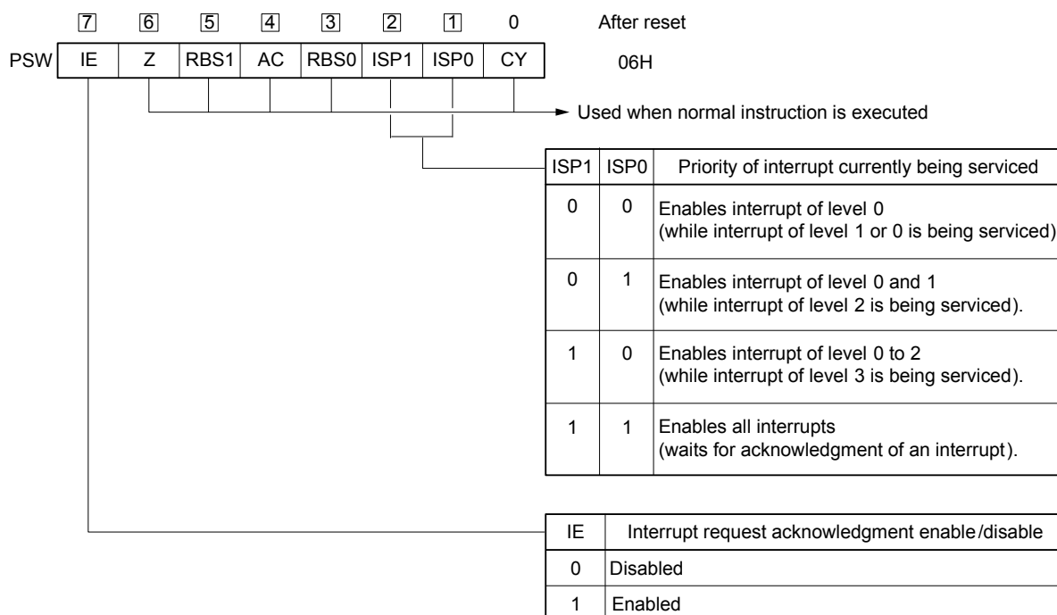
Figure 19 - 9 Configuration of Program Status Word
