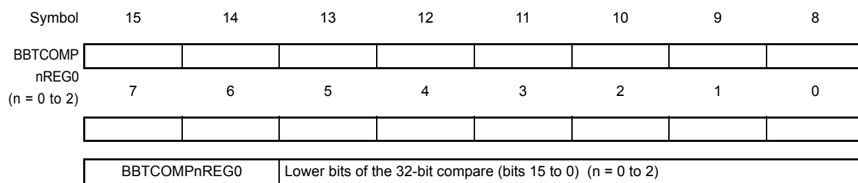
Figure 18 - 30 Timer Compare Register 1 (BBTCOMP0REG1 to BBTCOMP2REG1) Format
