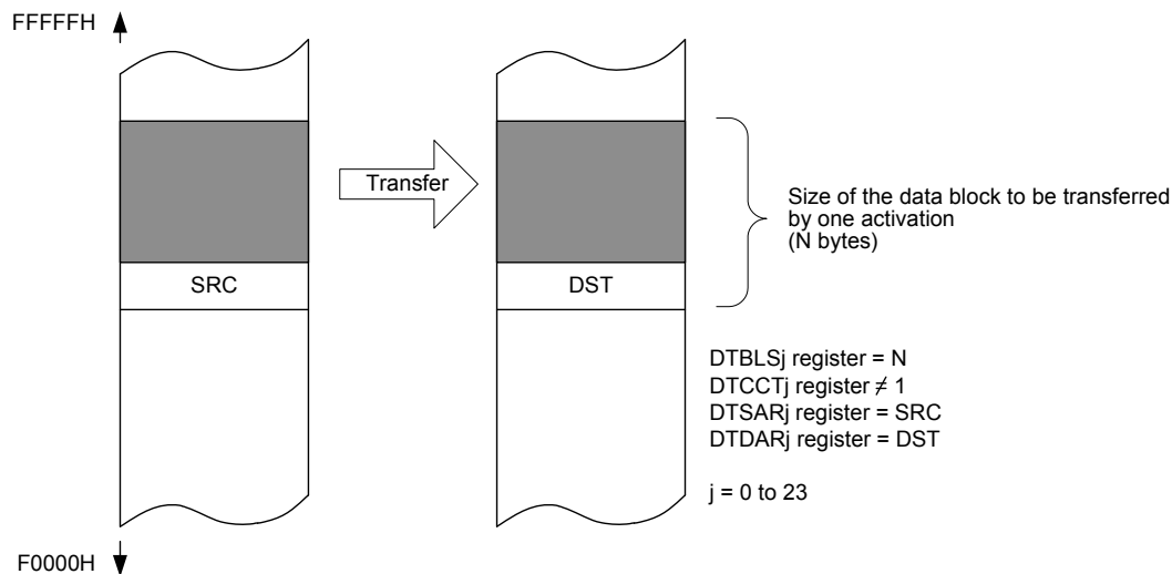
Figure 16 - 16 Data Transfers in Repeat Mode
