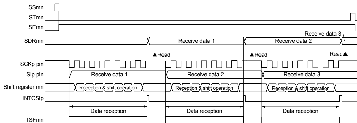
Figure 14 - 60 Timing Chart of Slave Reception (in Single-Reception Mode)
