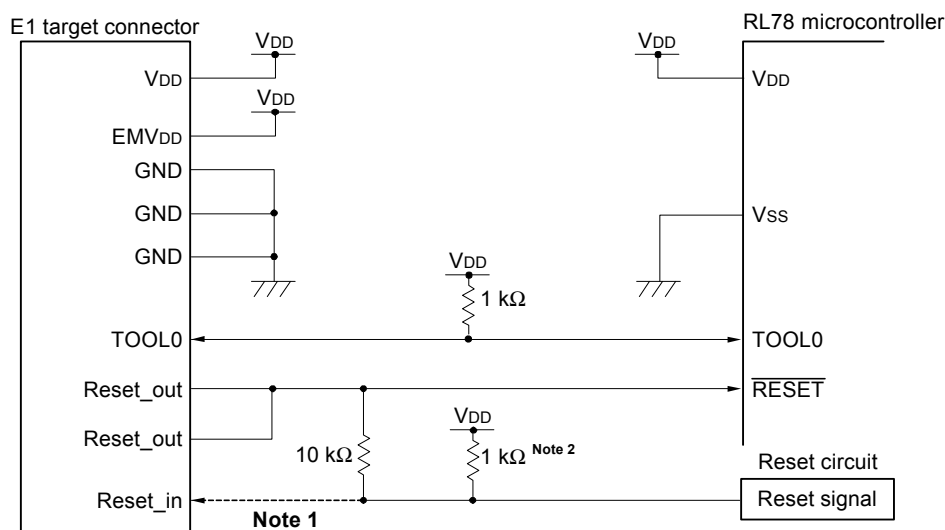
Figure 28 - 1 Connection Example of E1 On-chip Debugging Emulator
