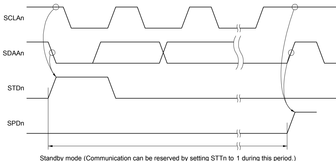
Figure 15 - 32 Timing for Accepting Communication Reservations
