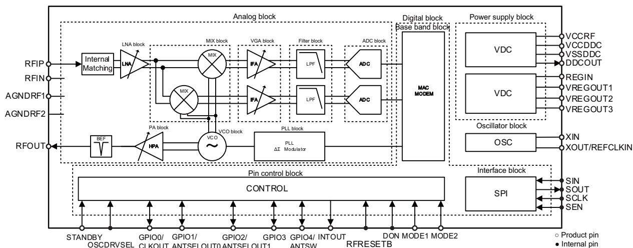
Figure 18 - 1 RF Transceiver Block Diagram
