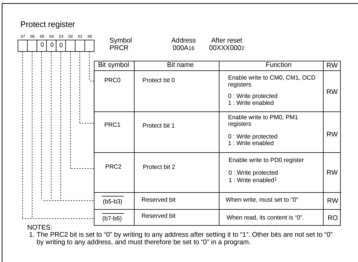
Figure 7.1 PRCR Register
