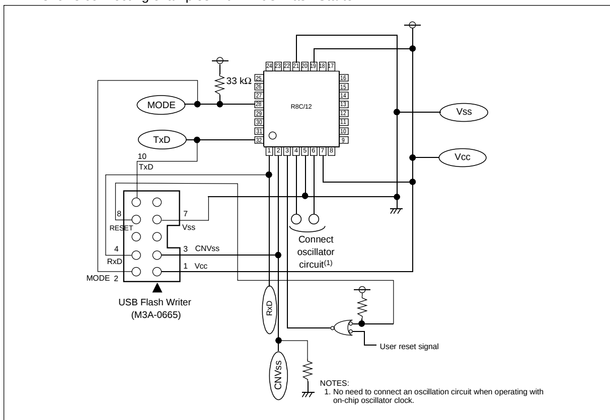
Appendix figure 2.1 Connecting examples with USB Flash Writer (M3A-0665)
