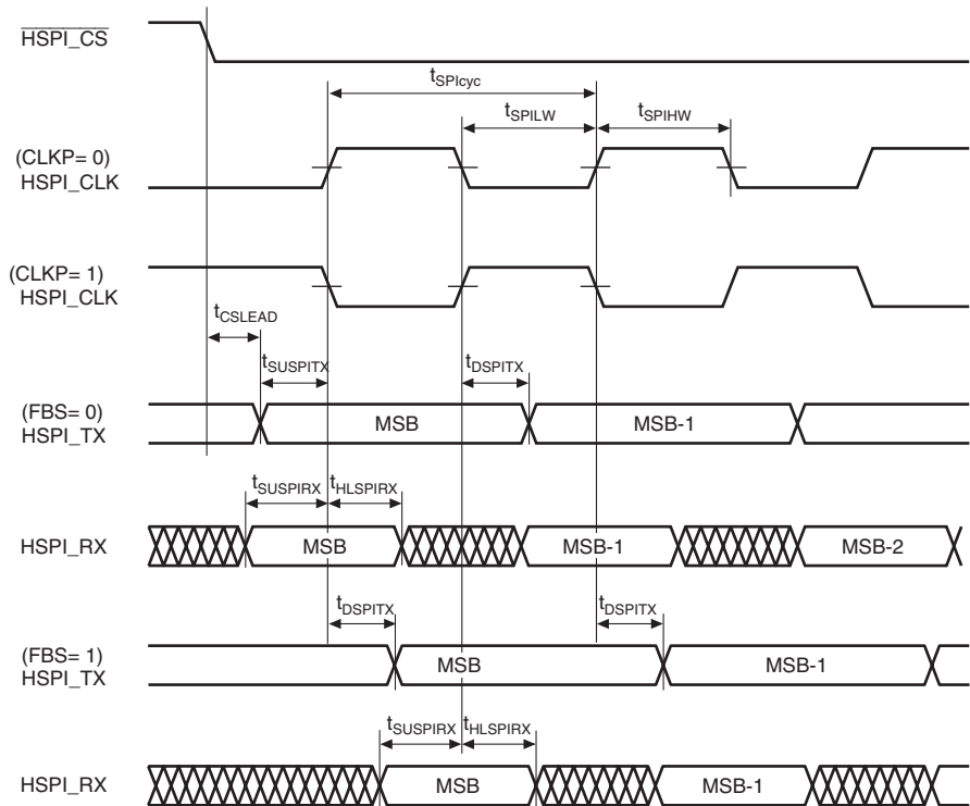
Figure 33.64 HSPI Data Output/Input Timing
