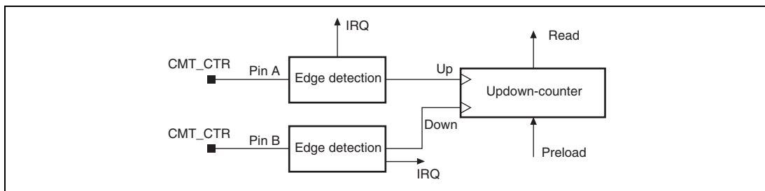
Figure 16.8 Updown-Counter Mode
