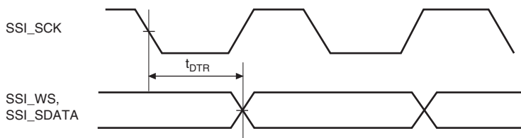
Figure 33.85 SSI Transmit Timing
