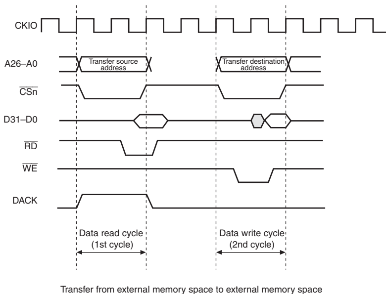
Figure 11.9 Example of Transfer Timing in Dual Address Mode
