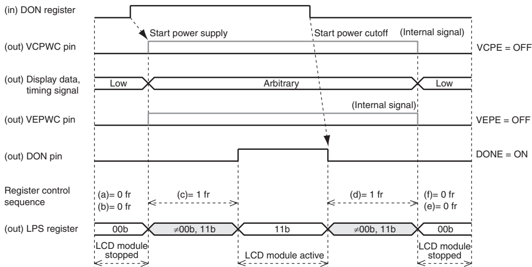
Figure 30.5 Power-Supply Control Sequence and States of the LCD Module
