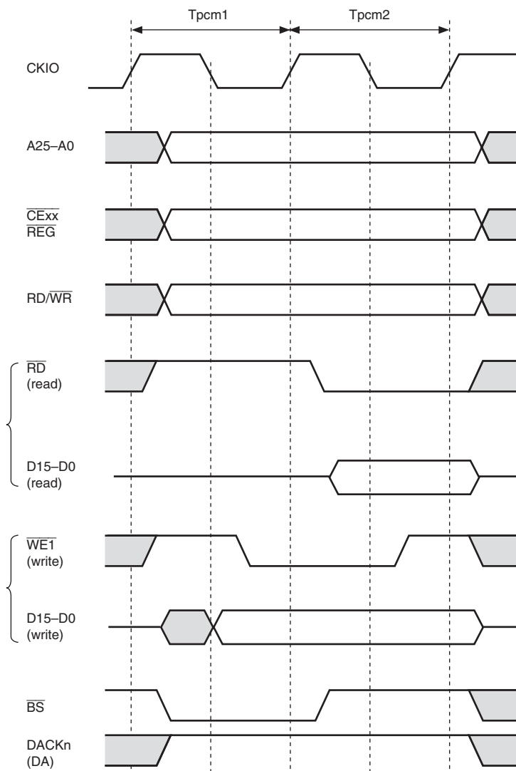
Figure 10.37 Basic Timing for PCMCIA Memory Card Interface
