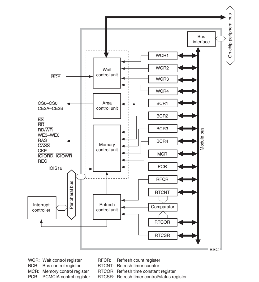
Figure 10.1 Block Diagram of BSC
