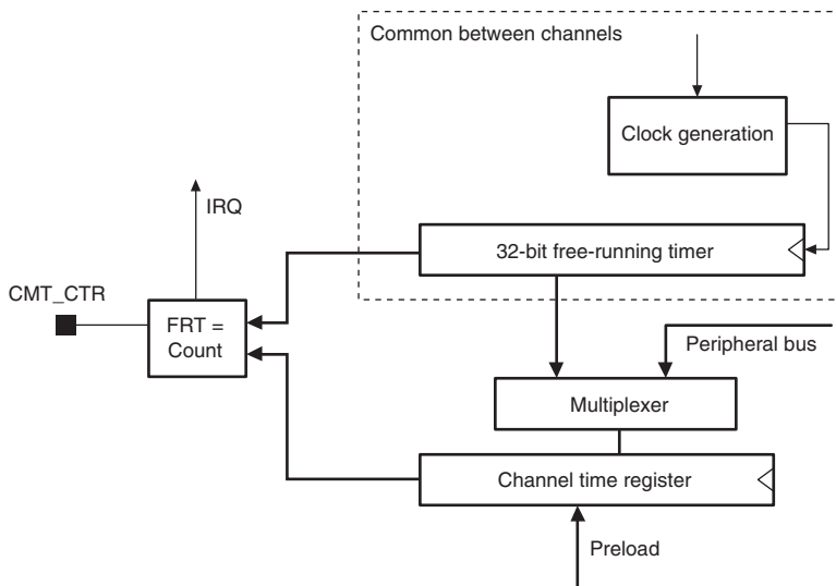
Figure 16.5 32-Bit Timer Mode: Output Compare
