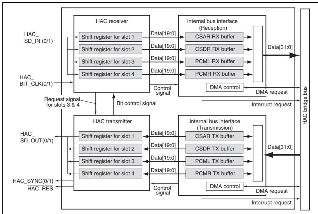
Figure 25.1 Block Diagram
