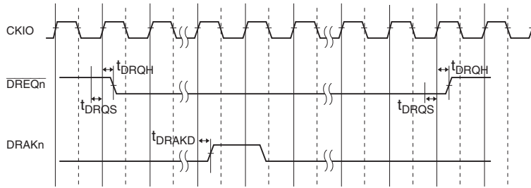
Figure 33.50 \overline{\text{DREQ}} /DRAK Timing
