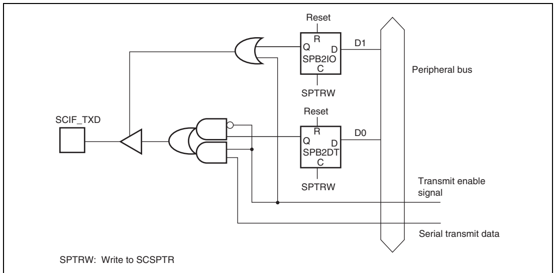
Figure 17.5 SCIF_TXD Pin
