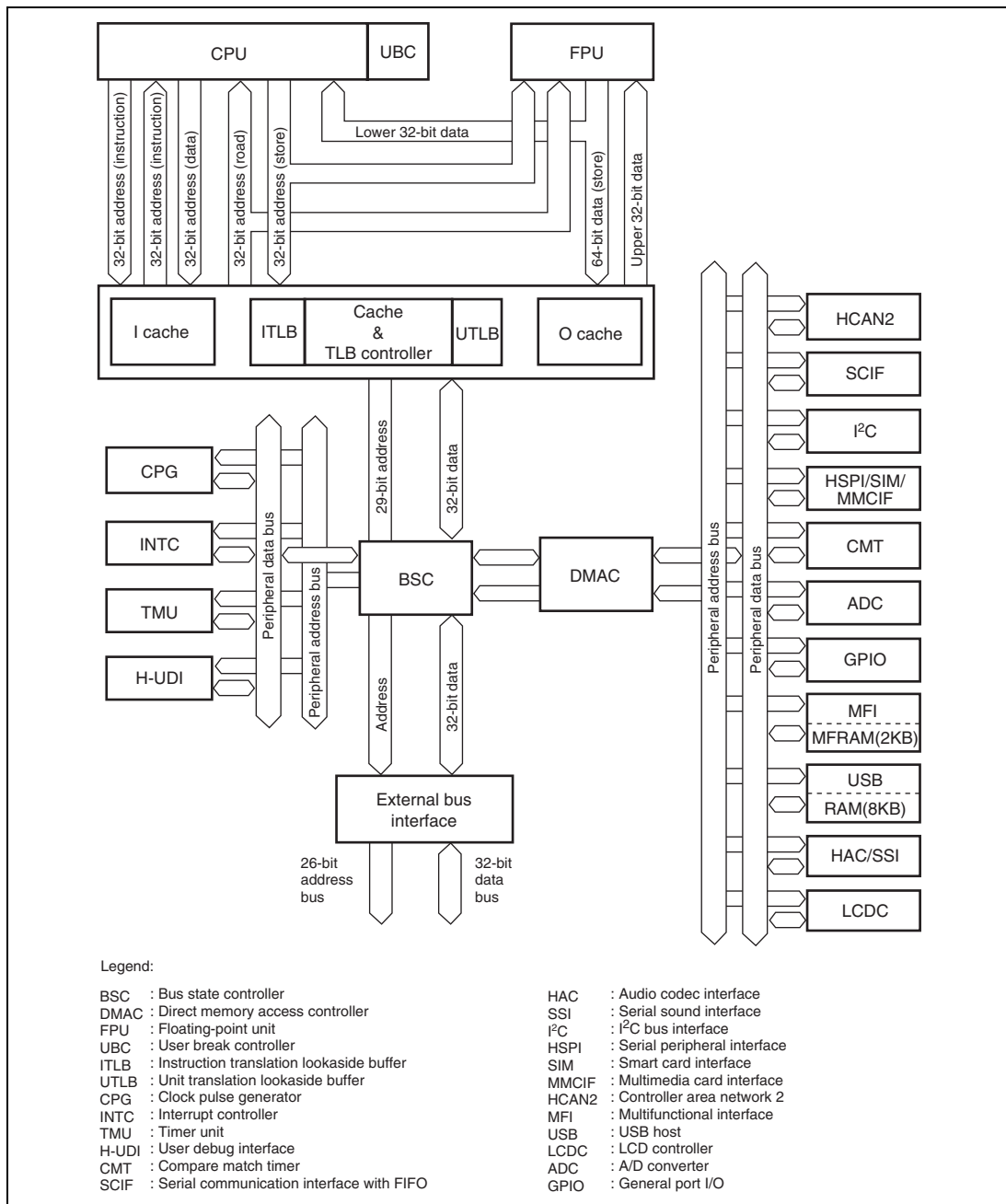
Figure 1.1 SH7760 Block Diagram
