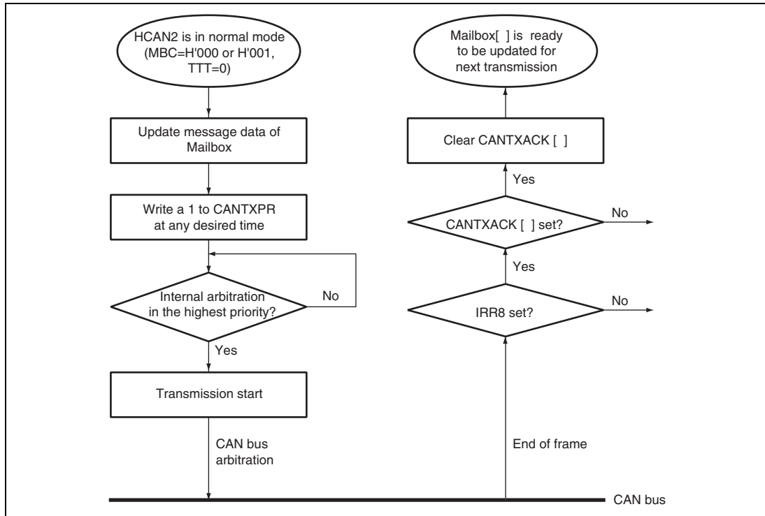
Figure 22.6 Transmission Request
