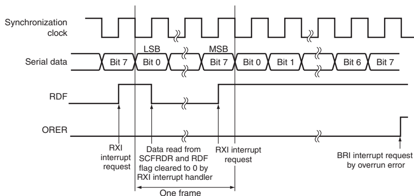
Figure 17.20 Sample SCIF Reception Operation in Synchronous Mode
