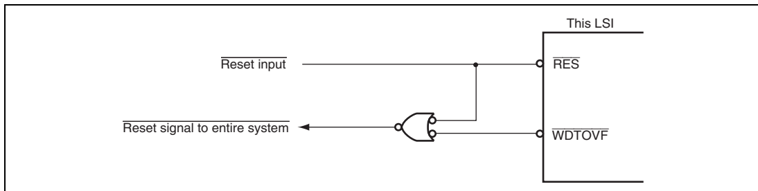
Figure 15.6 Circuit for System Reset by \overline{\text{WDTOVF}} Signal (Example)
