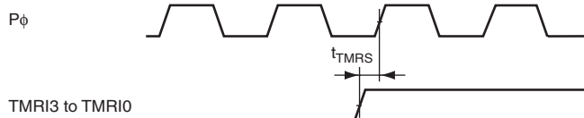
Figure 26.31 8-Bit Timer Reset Input Timing
