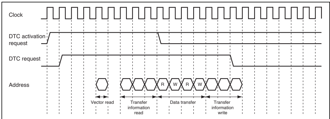
Figure 10.12 DTC Operation Timing (Example of Short Address Mode in Block Transfer Mode with Block Size of 2)
