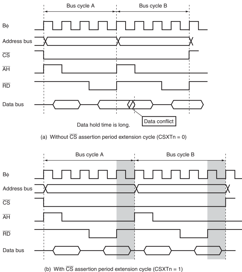
Figure 8.35 Consecutive Read Accesses to Same Area (Address/Data Multiplexed I/O Space)
