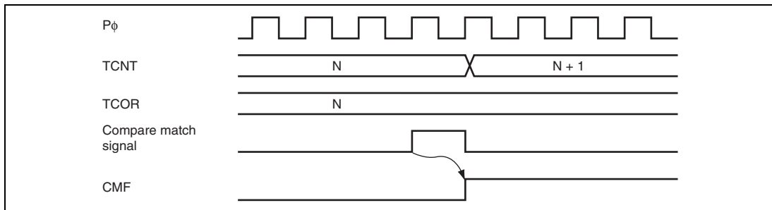
Figure 14.9 Timing of CMF Setting at Compare Match
