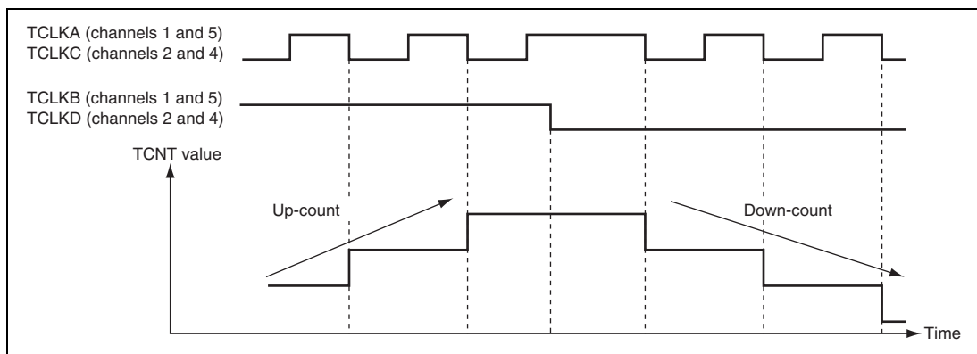
Figure 12.26 Example of Phase Counting Mode 2 Operation
