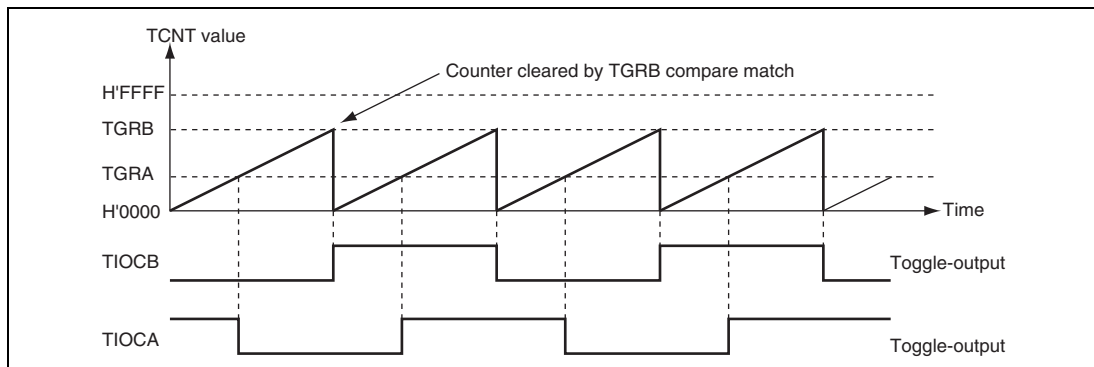
Figure 12.7 Example of Toggle Output Operation
