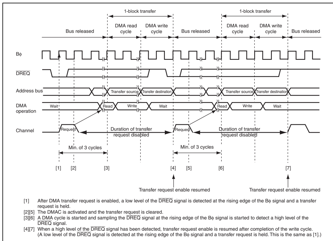
Figure 9.30 Example of Transfer in Block Transfer Mode Activated by \overline{\text{DREQ}} Falling Edge
