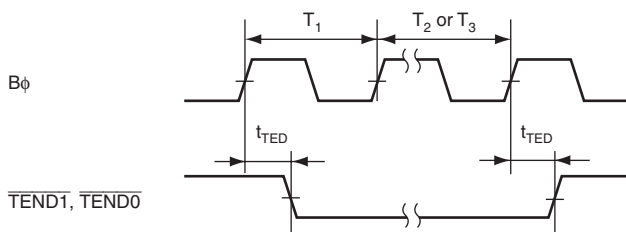
Figure 26.23 DMAC, \overline{TEND} Output Timing
