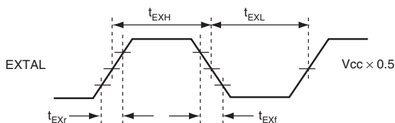
Figure 23.5 External Clock Input Timing
