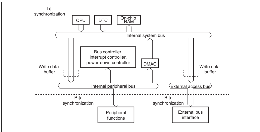
Figure 8.4 Internal Bus Configuration
