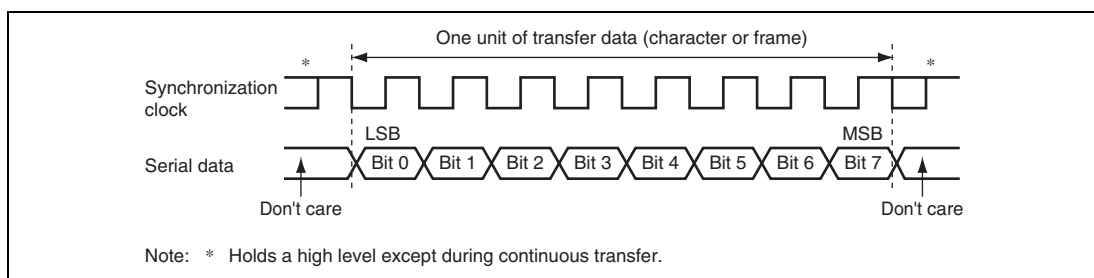
Figure 16.14 Data Format in Clocked Synchronous Communication (LSB-First)
