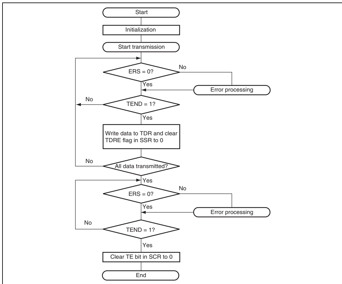
Figure 16.28 Sample Transmission Flowchart
