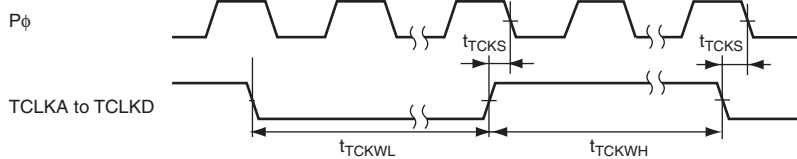
Figure 26.28 TPU Clock Input Timing
