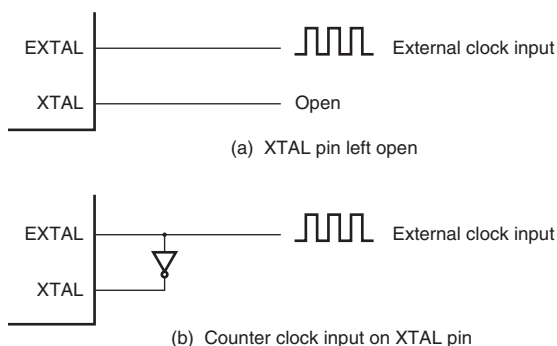
Figure 23.4 External Clock Input (Examples)
