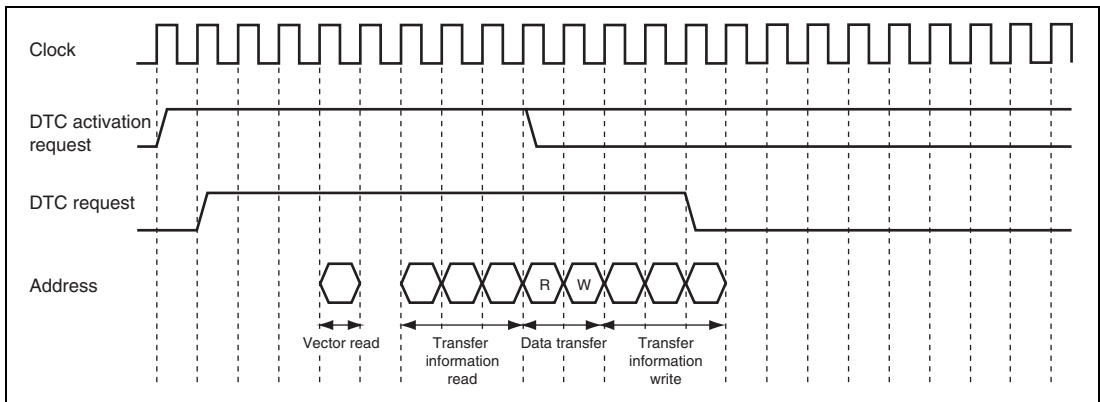
Figure 10.11 DTC Operation Timing (Example of Short Address Mode in Normal Transfer Mode or Repeat Transfer Mode)
