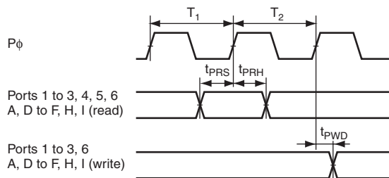
Figure 26.26 I/O Port Input/Output Timing
