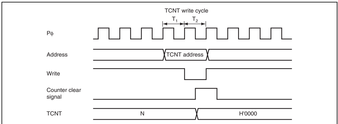
Figure 12.46 Conflict between TCNT Write and Clear Operations
