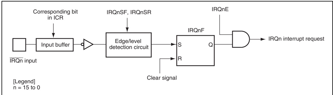
Figure 6.2 Block Diagram of Interrupts \text{IRQn}
