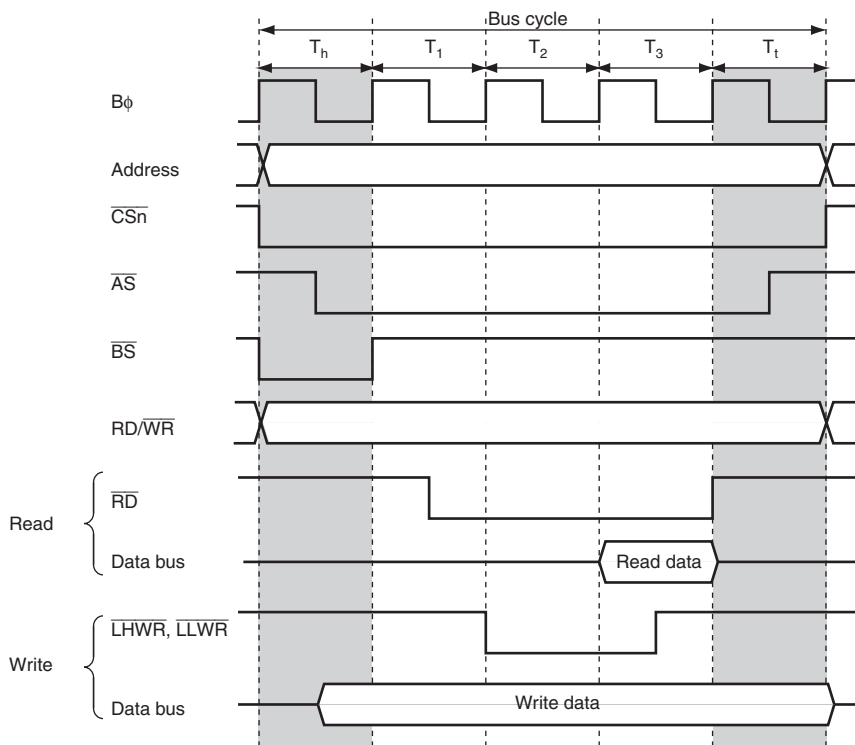
Figure 8.3 \overline{\text{CS}} and Address Assertion Period Extension (Example of Basic Bus Interface, 3-State Access Space, and RDNn = 0)
