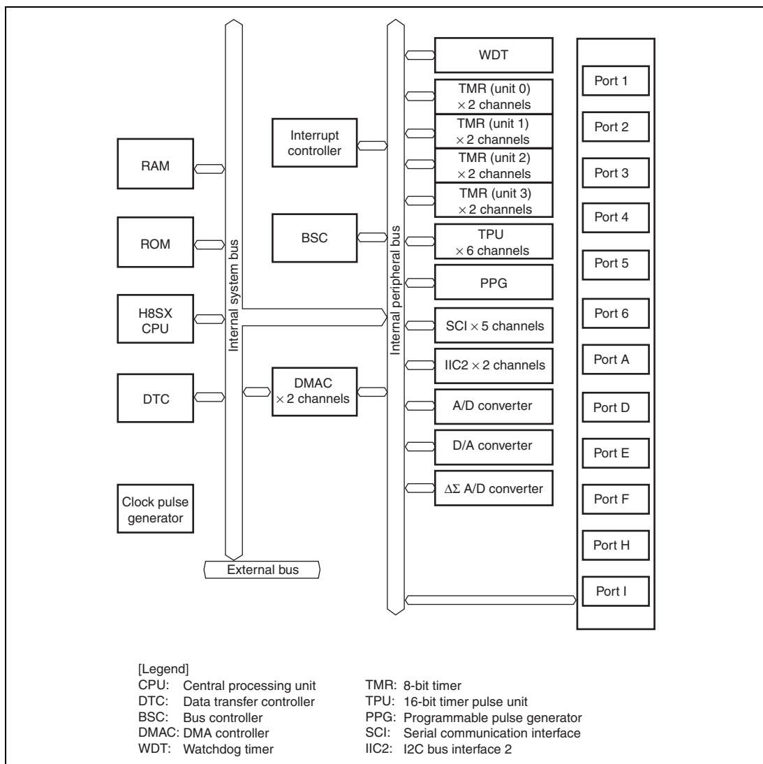
Figure 1.2 Block Diagram
