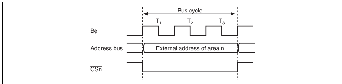
Figure 8.8 \overline{CSn} Signal Output Timing ( n = 0 to 7)
