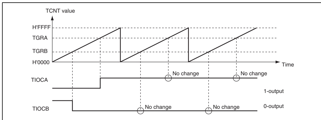
Figure 12.6 Example of 0-Output/1-Output Operation
