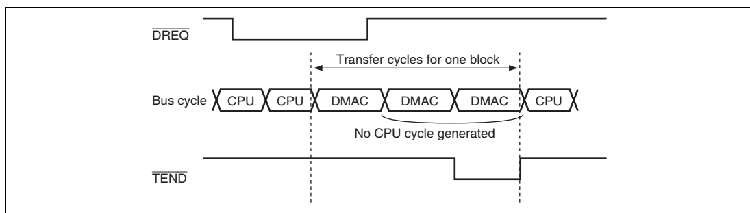
Figure 9.10 Operations in Block Transfer Mode
