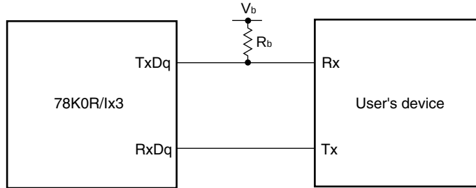
UART mode connection diagram (communication at different potential)
