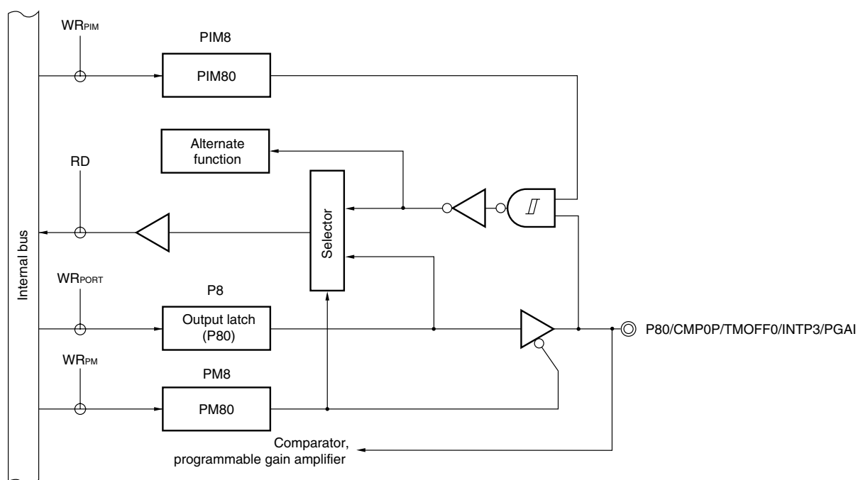
Figure 4-20. Block Diagram of P80
