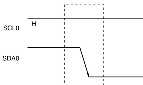
Figure 14-15. Start Conditions
