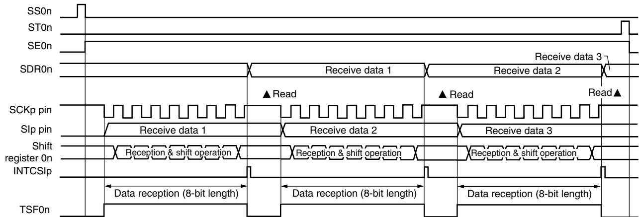
Figure 13-60. Timing Chart of Slave Reception (in Single-Reception Mode) (Type 1: DAP0n = 0, CKP0n = 0)
