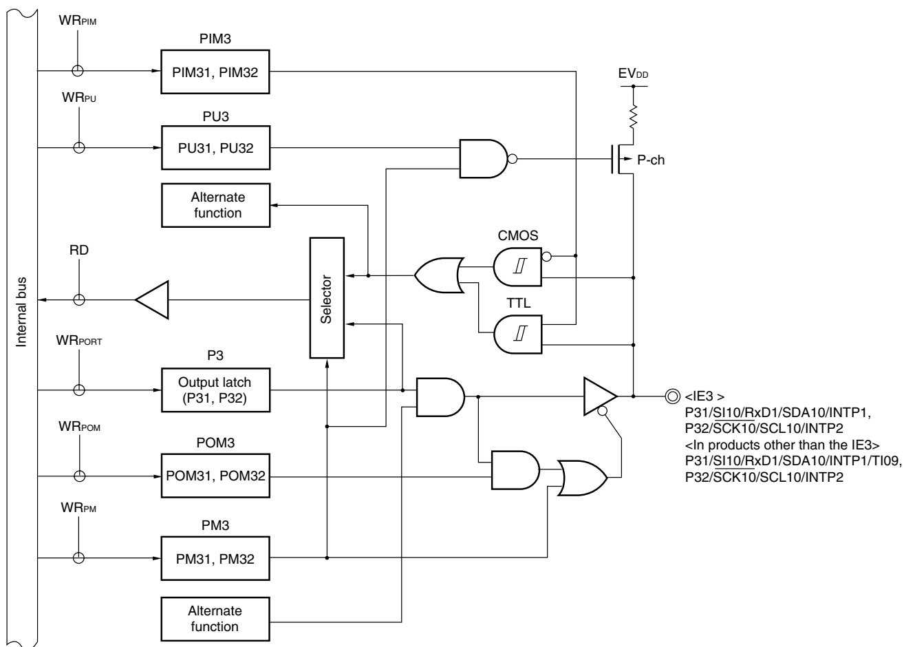
Figure 4-6. Block Diagram of P31 and P32
