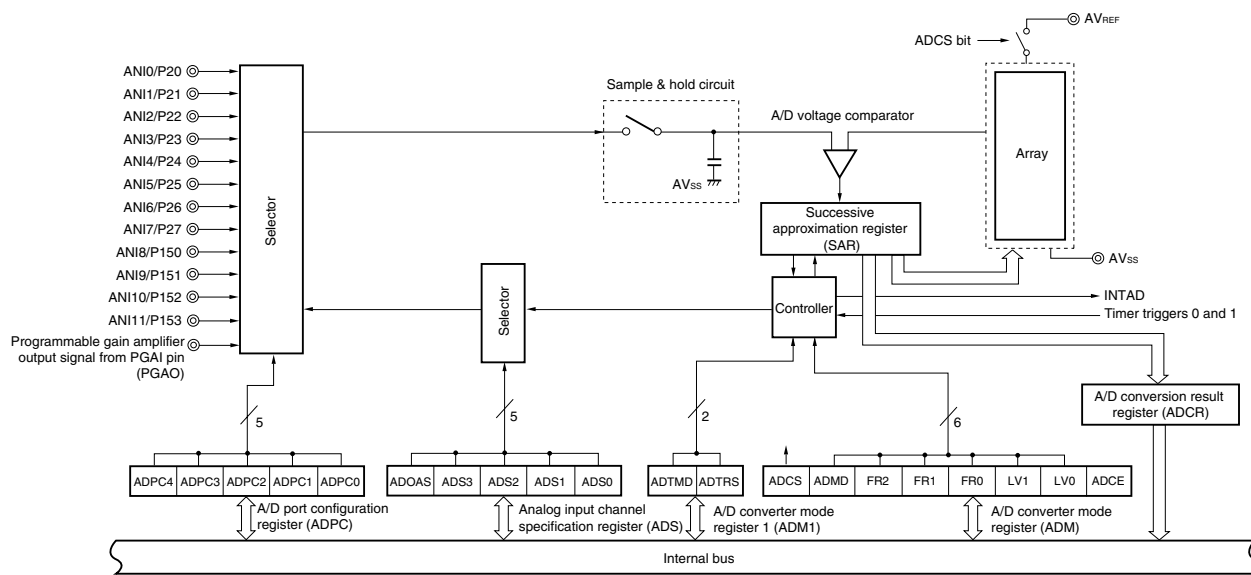
Figure 12-1. Block Diagram of A/D Converter
