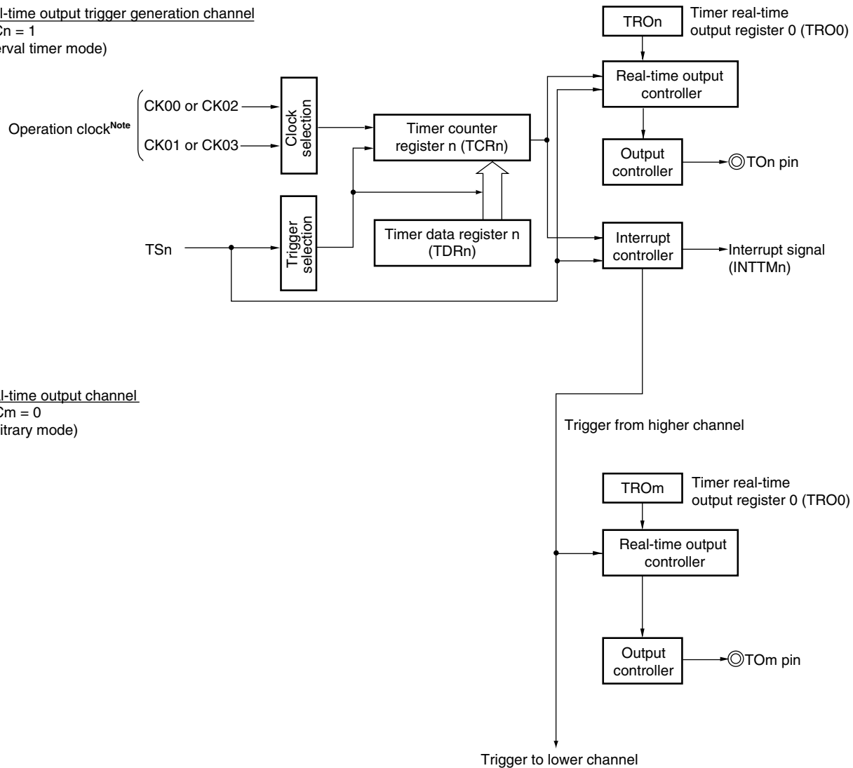
Figure 7-15. Block Diagram of Operation as Real-Time Output Function (Type 1)
