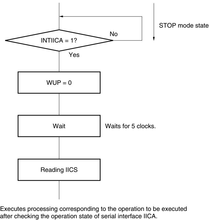
Figure 14-23. Flow When Setting WUP = 0 upon Address Match (Including Extension Code Reception)
