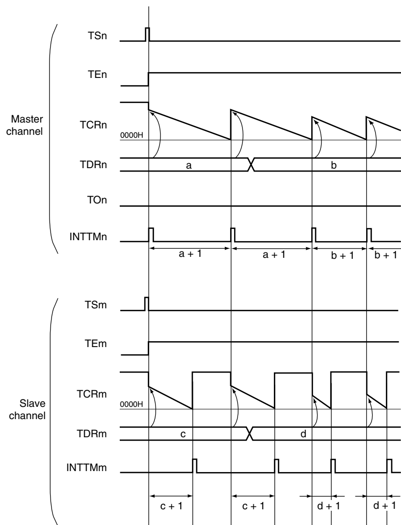
Figure 7-51. Example of Basic Timing of Operation as A/D Conversion Trigger Output Function (Type 1)
