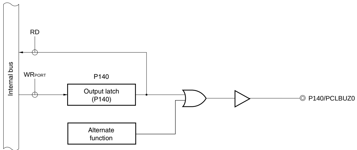
Figure 4-26. Block Diagram of P140
