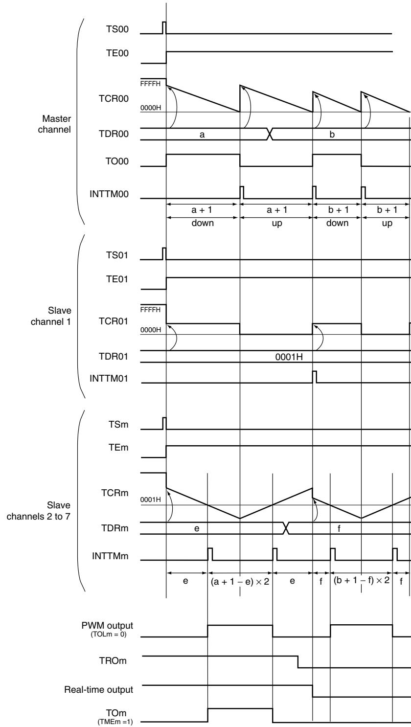
Figure 7-86. Example of Basic Timing of Operation as Non-complementary Modulation Output Function (Type 2) (Default setting : TO00 = 1, T0m = 0, MD000 = 0)
