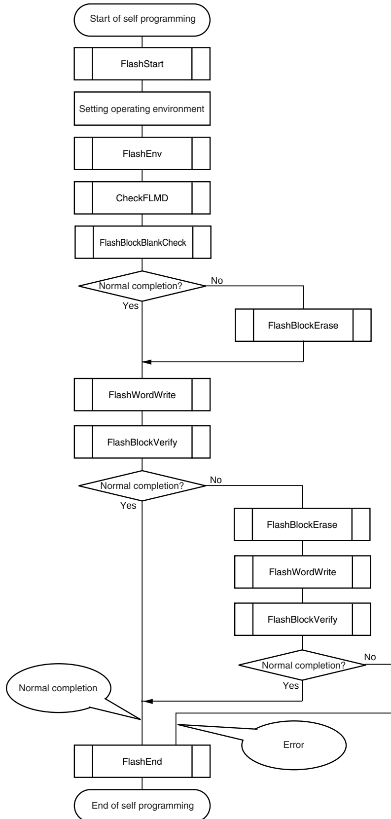
Figure 24-15. Flow of Self Programming (Rewriting Flash Memory)
