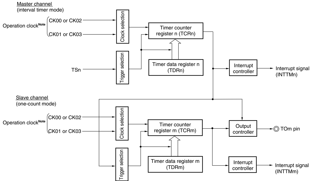
Figure 6-61. Block Diagram of Operation as PWM Function
