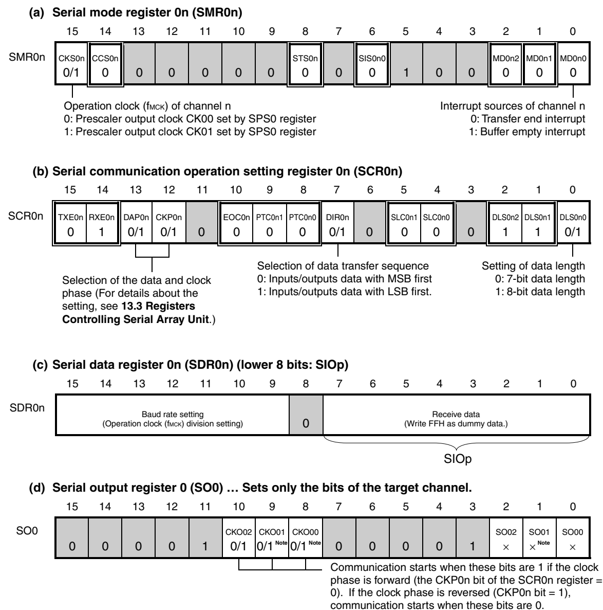
Figure 13-32. Example of Contents of Registers for Master Reception of 3-Wire Serial I/O (CSI00 Note , CSI01 Note , CSI10) (1/2)
