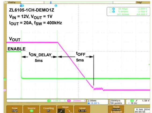
FIGURE 11. TYPICAL TURN-OFF RAMP, t_{FALL} = 5ms , t_{OFF\_DELAY} = 5ms
