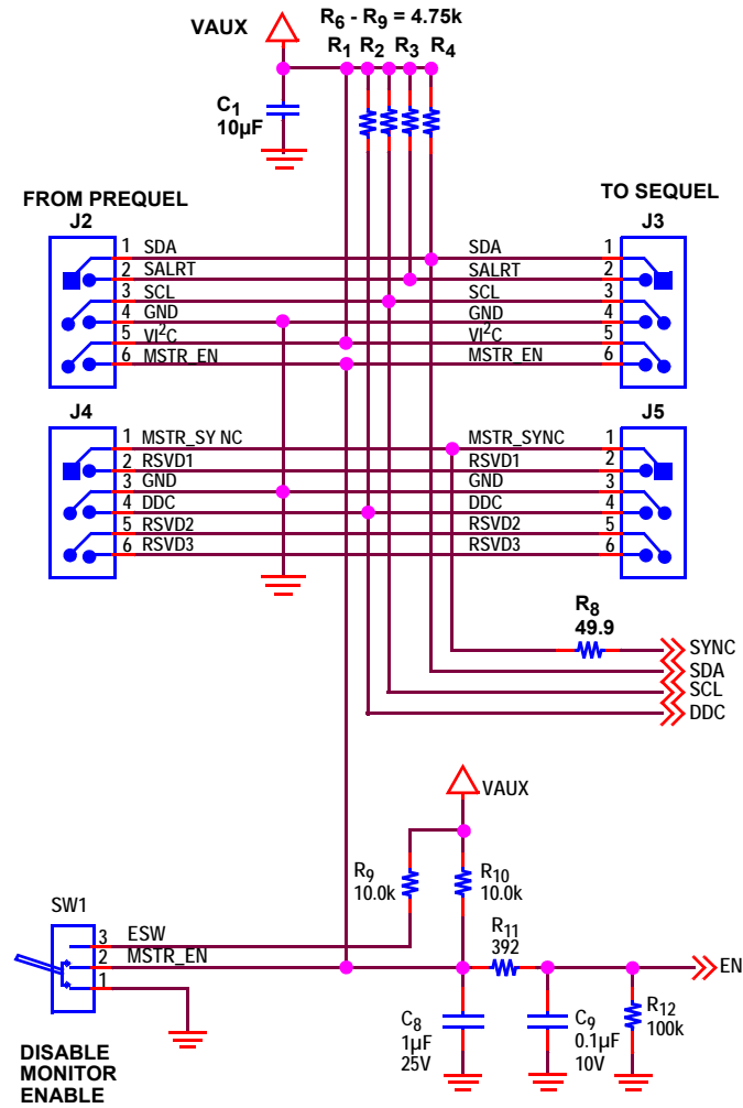
FIGURE 5. ZL6105-1CH-DEMO1Z INTERFACE
