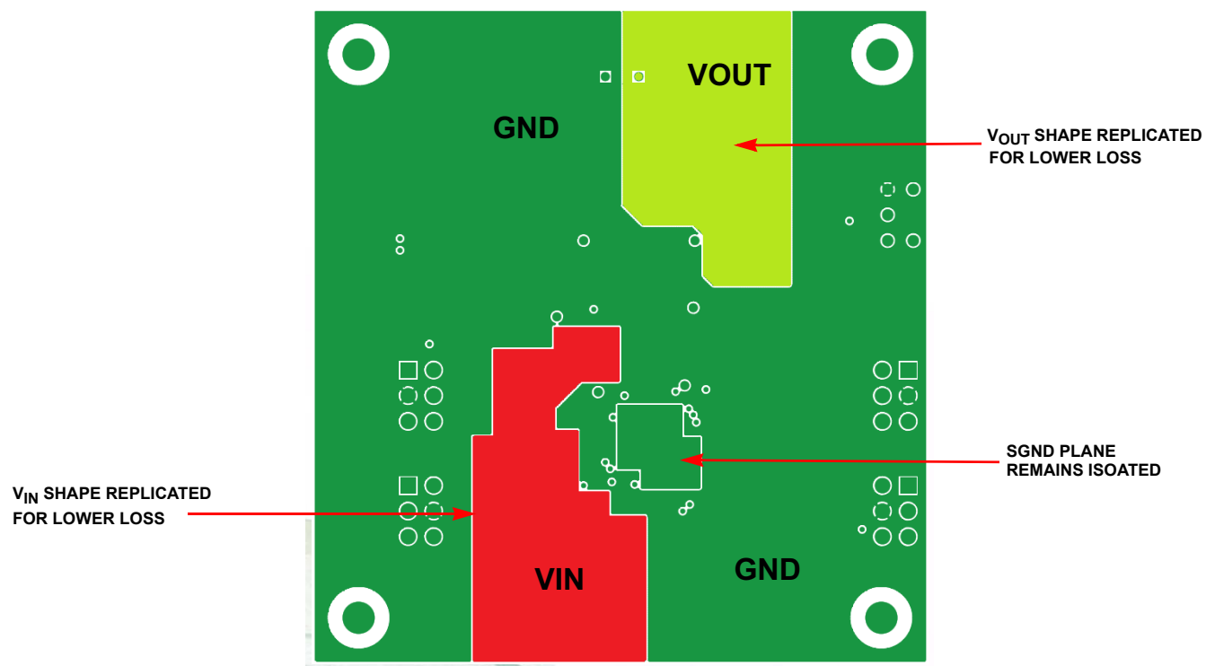
FIGURE 17. INNER LAYER 3
