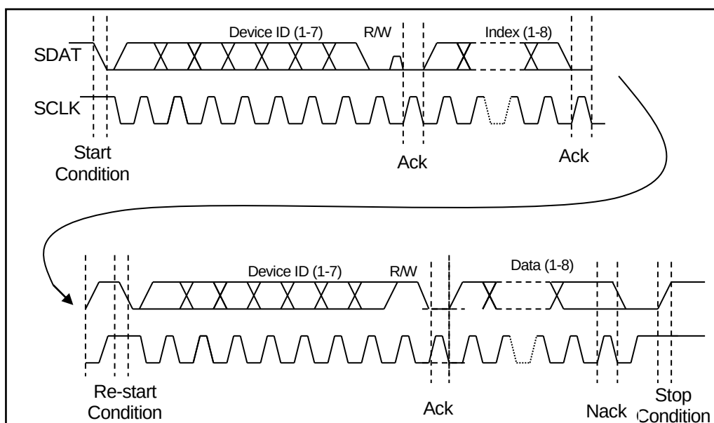
FIGURE 24. ONE COMPLETE REGISTER READ SEQUENCE VIA THE SERIAL BUS INTERFACE
