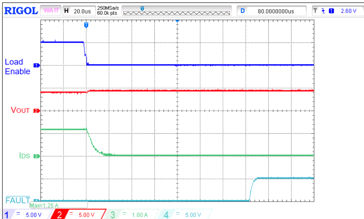
Figure 9. Typical FAULT de-assertion waveform for V_{IN} = 4.5 V, C_{LOAD} = 10 \mu F, I_{ACL} = 1 A, R_{SET} = 91 k \Omega , switch out 3.3 \Omega load
