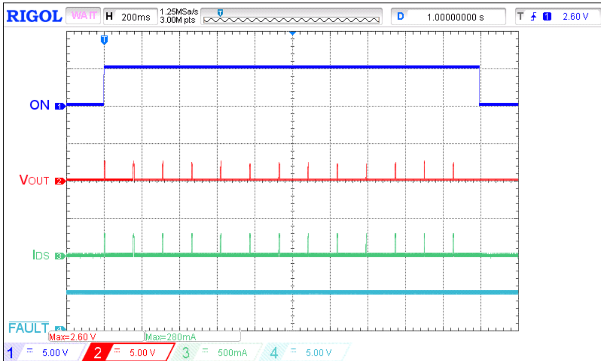
Figure 43. Typical SOA waveform during power up under heavy load for V_{IN} = 20 V, C_{LOAD} = 10 \mu F, R_{SET} = 30.1 k \Omega , R_{LOAD} = 8 \Omega
