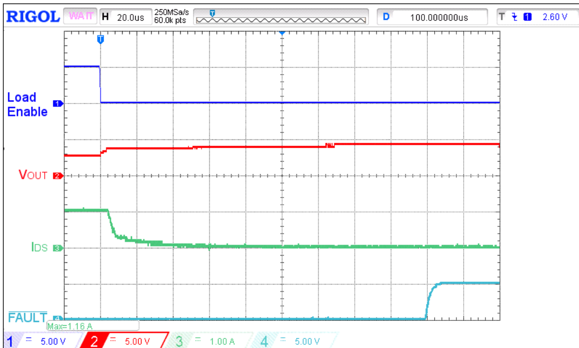
Figure 24. Typical FAULT de-assertion waveform for V_{IN} = 4.5 V, C_{LOAD} = 10 \mu F, I_{ACL} = 1 A, R_{SET} = 91 k \Omega , switch out 3.8 \Omega load
