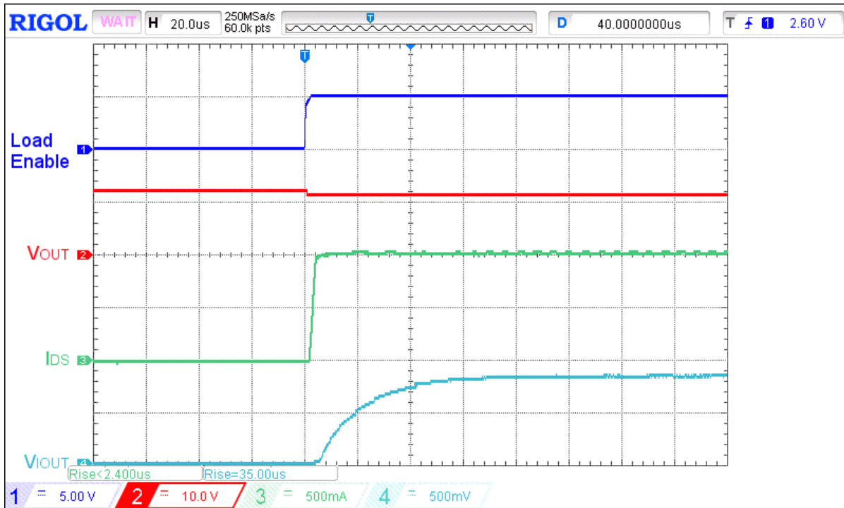
Figure 35. Typical I_{OUT} response time waveform for V_{IN} = 12 V, C_{LOAD} = 10 μF, R_{LOAD} = 12 Ω, C_{IOUT} = 0.18 nF, R_{IOUT} = 84.5 kΩ, load step 0 A to 1 A
