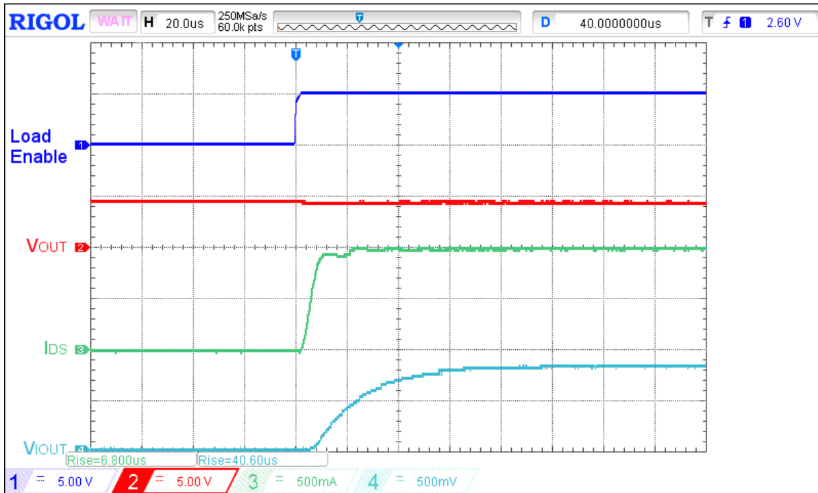
Figure 31. Typical I_{OUT} response time waveform for V_{IN} = 4.5 V, C_{LOAD} = 10 μF, R_{LOAD} = 4.5 Ω, C_{IOUT} = 0.18 nF, R_{IOUT} = 84.5 kΩ, load step 0 A to 1 A
