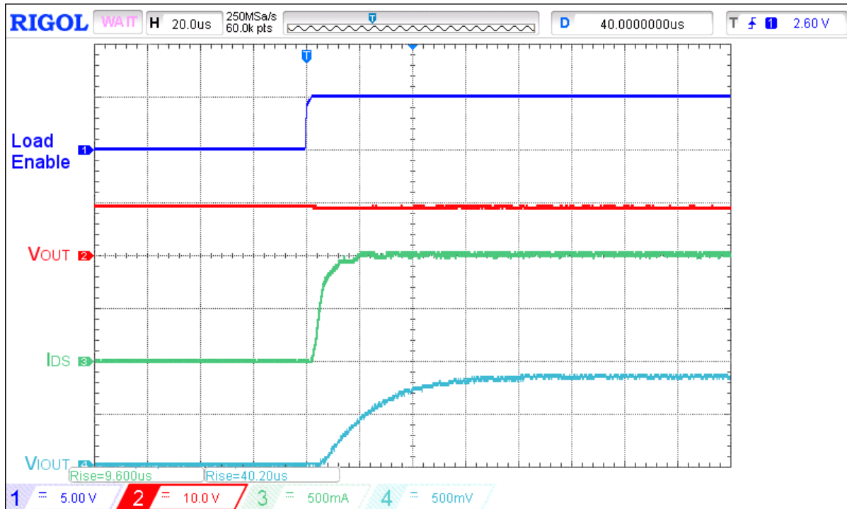
Figure 33. Typical I_{OUT} response time waveform for V_{IN} = 9 V, C_{LOAD} = 10 μF, R_{LOAD} = 9 Ω, C_{IOUT} = 0.18 nF, R_{IOUT} = 84.5 kΩ, load step 0 A to 1 A
