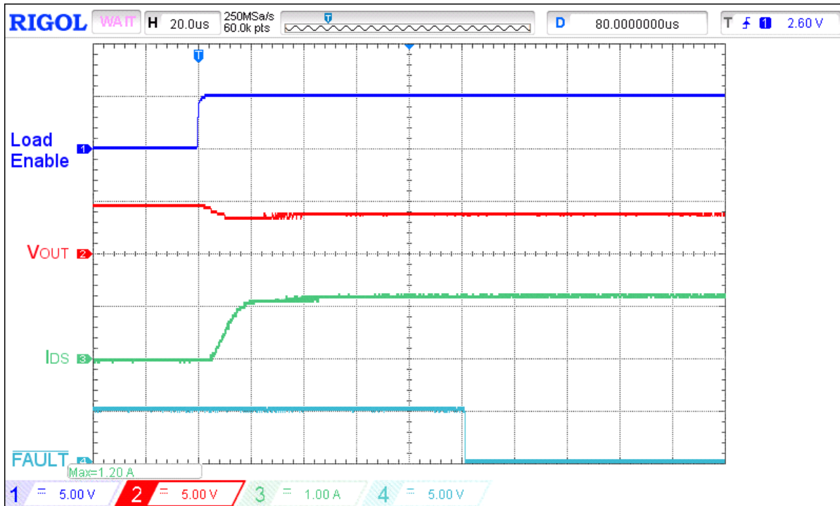
Figure 23. Typical FAULT assertion waveform for V_{IN} = 4.5 V, C_{LOAD} = 10 \mu F, I_{ACL} = 1 A, R_{SET} = 91 k \Omega , switch on 3.8 \Omega load
