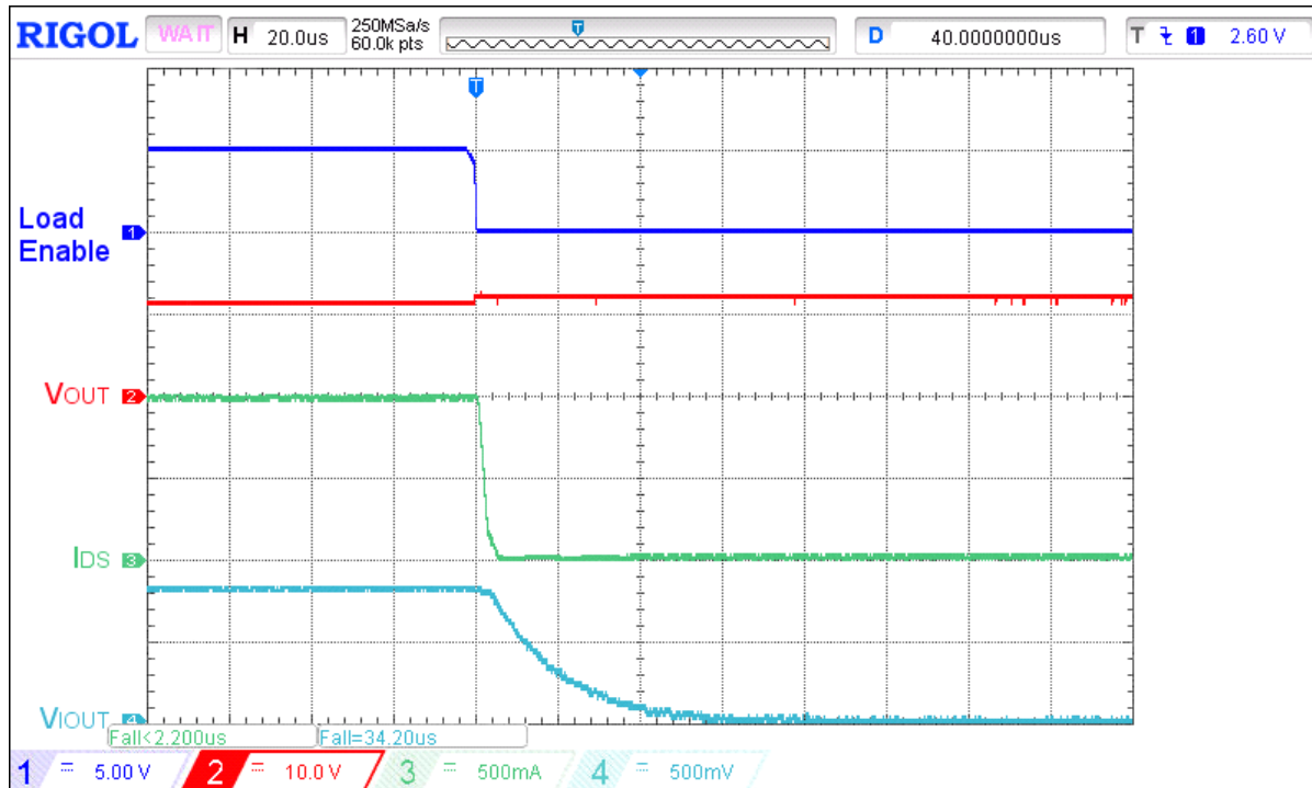
Figure 36. Typical I_{OUT} response time waveform for V_{IN} = 12 V, C_{LOAD} = 10 μF, R_{LOAD} = 12 Ω, C_{IOUT} = 0.18 nF, R_{IOUT} = 84.5 kΩ, load step 1 A to 0 A
