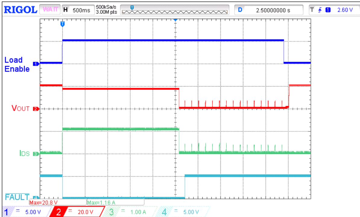
Figure 22. Thermally induced SOA shutdown for V_{IN} = 20\text{ V} , C_{LOAD} = 10\text{ }\mu\text{F} , I_{ACL} = 1\text{ A} , R_{SET} = 91\text{ k}\Omega
