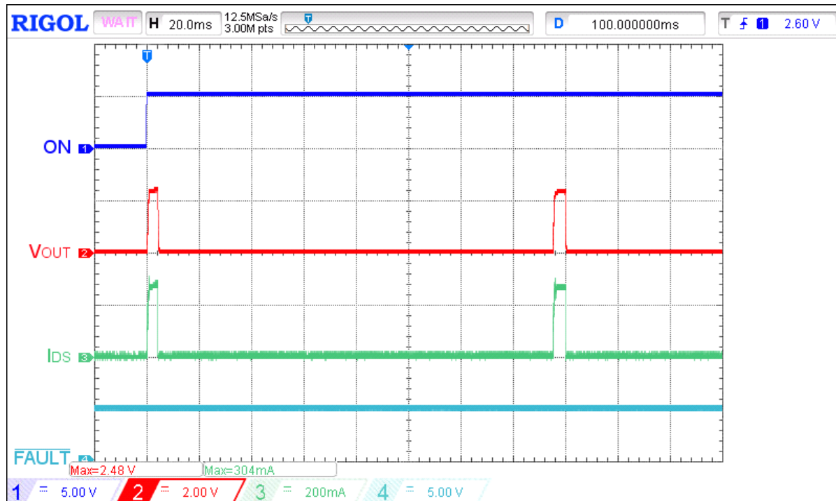
Figure 44. Extended typical SOA waveform during power up under heavy load for V_{IN} = 20 V, C_{LOAD} = 10 \mu F, R_{SET} = 30.1 k \Omega , R_{LOAD} = 8 \Omega
