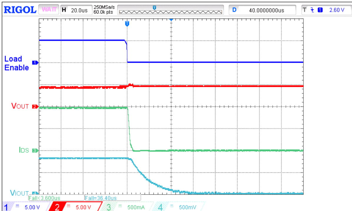
Figure 32. Typical I_{OUT} response time waveform for V_{IN} = 4.5 V, C_{LOAD} = 10 μF, R_{LOAD} = 4.5 Ω, C_{IOUT} = 0.18 nF, R_{IOUT} = 84.5 kΩ, load step 1 A to 0 A
