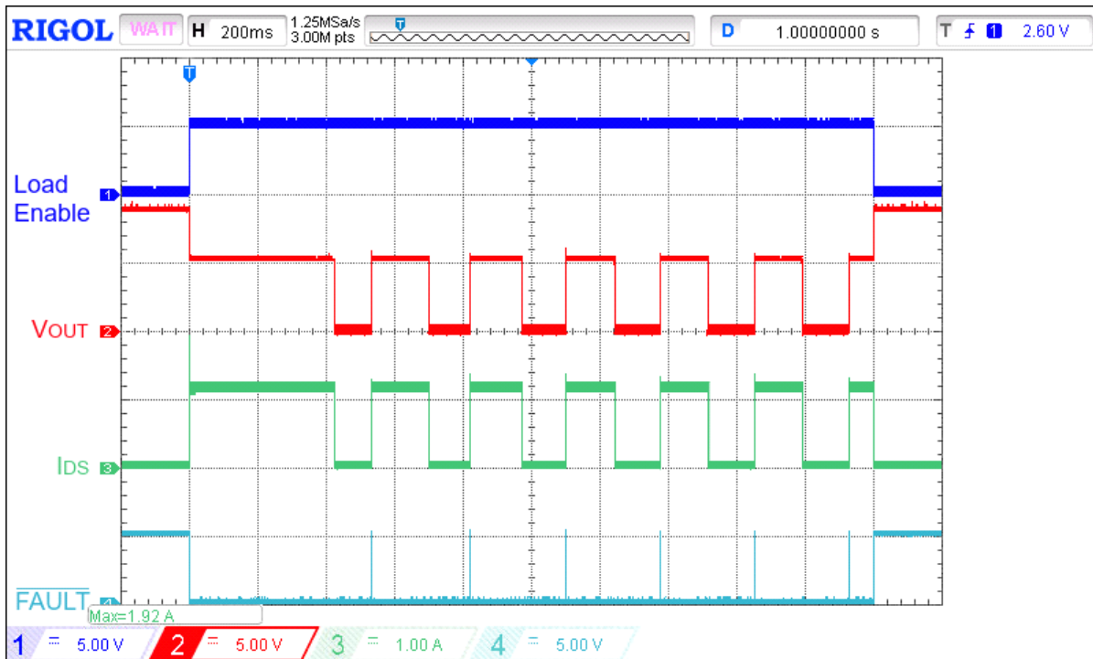
Figure 11. Typical ACL operation waveform for V_{IN} = 9 V, C_{LOAD} = 10 μF, I_{ACL} = 1 A, R_{SET} = 91 kΩ
