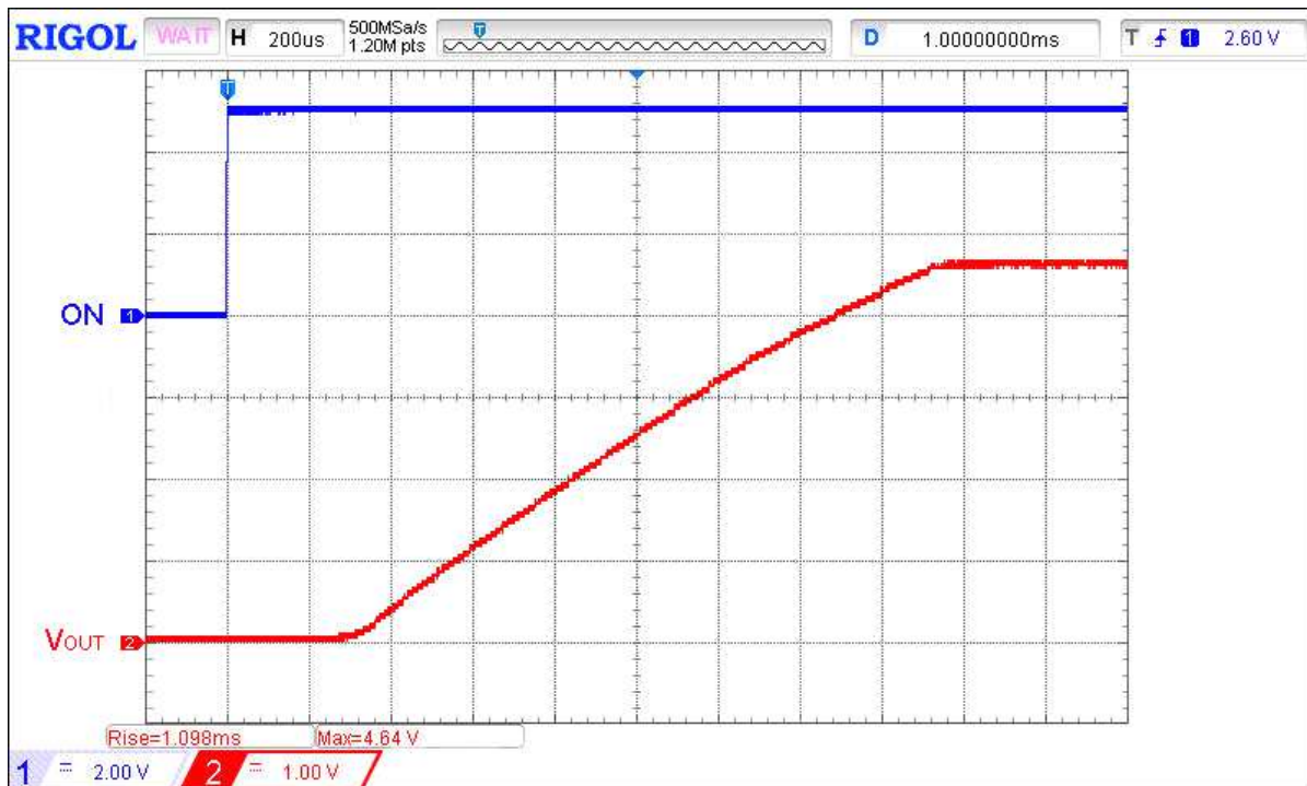
Typical Turn-on Waveforms
