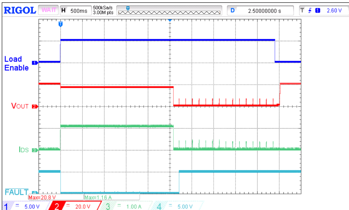
Figure 12. Thermally induced SOA shutdown for V_{IN} = 20 V, C_{LOAD} = 10 \mu F, I_{ACL} = 1 A, R_{SET} = 91 k \Omega
