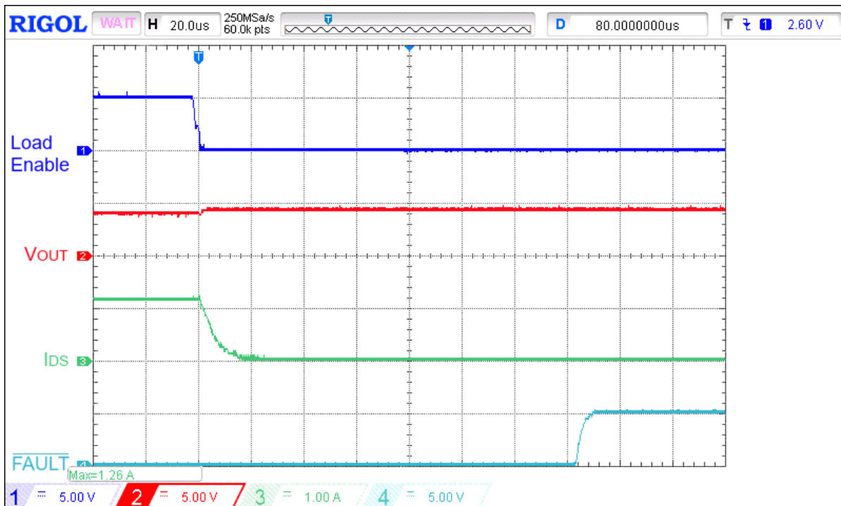
Figure 14. Typical FAULT de-assertion waveform for V_{IN} = 4.5 V, C_{LOAD} = 10 \mu F, I_{ACL} = 1 A, R_{SET} = 91 k \Omega , switch out 3.3 \Omega load
