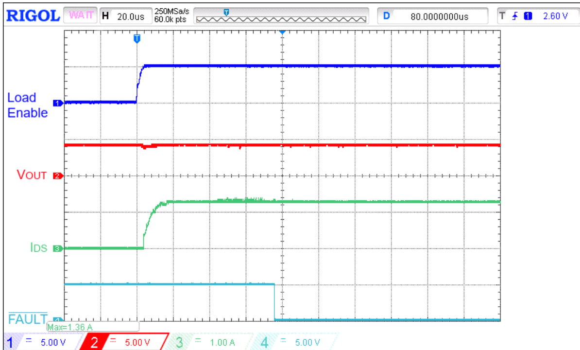
Figure 13. Typical FAULT assertion waveform for V_{IN} = 4.5 V, C_{LOAD} = 10 \mu F, I_{ACL} = 1 A, R_{SET} = 91 k \Omega , switch on 3.3 \Omega load
