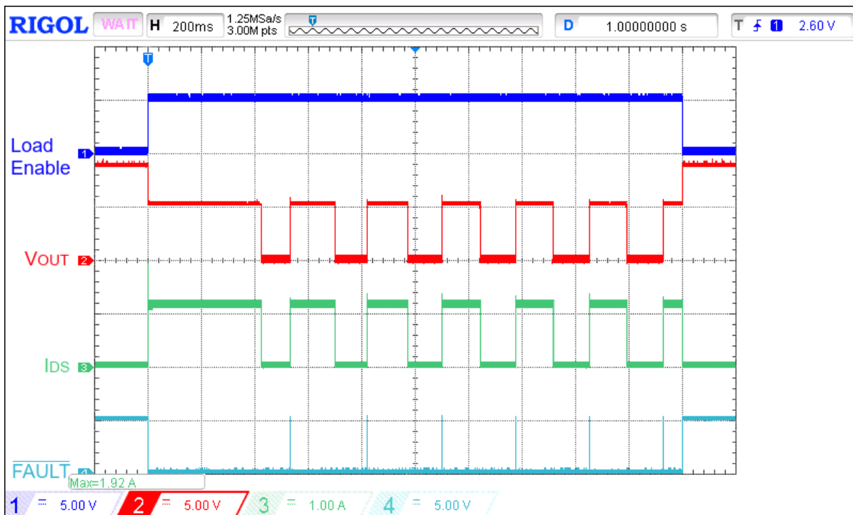
Figure 11. Typical ACL operation waveform for V_{IN} = 9 V, C_{LOAD} = 10 \mu F, I_{ACL} = 1 A, R_{SET} = 91 k \Omega
