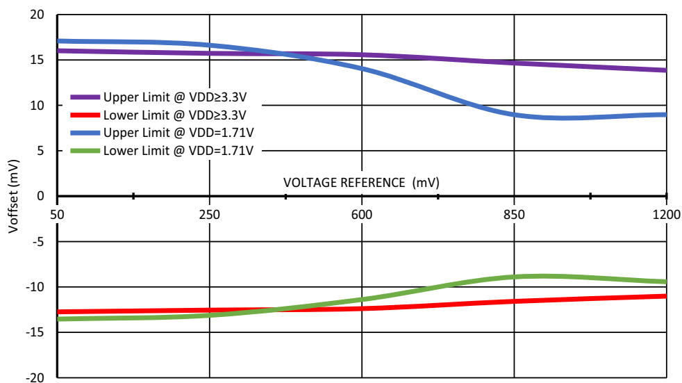
Figure 53. Buffer Input Voltage Offset vs. Voltage Reference at T = (-40.... +85)^{\circ}\text{C} , Buffer Bandwidth = 50 kHz, V_{\text{phys}} = 0 \text{ mV} , Gain = 1.
