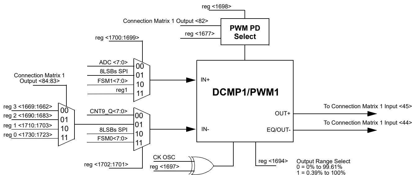
Figure 98. DCMP1/PWM1 Functional Diagram
