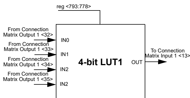
Figure 45. 4-bit LUT_1
