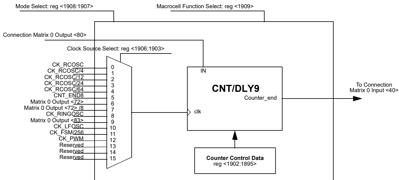
Figure 86. CNT/DLY9/PWM_RAMP
