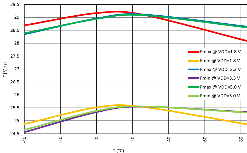
Figure 123. Ring Oscillator Frequency vs. Temperature, Ring OSC=27 MHz
