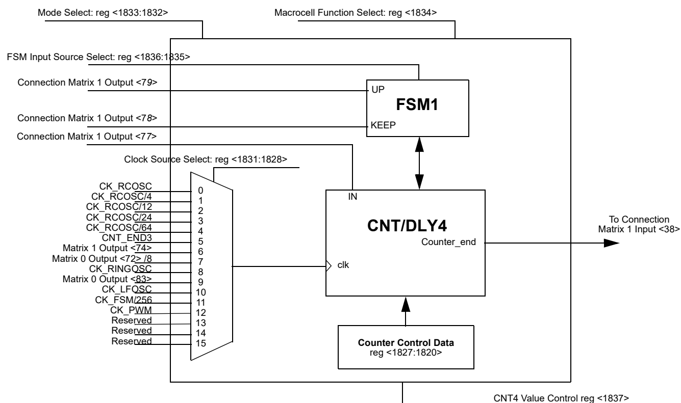
Figure 81. CNT/DLY4/FSM0
