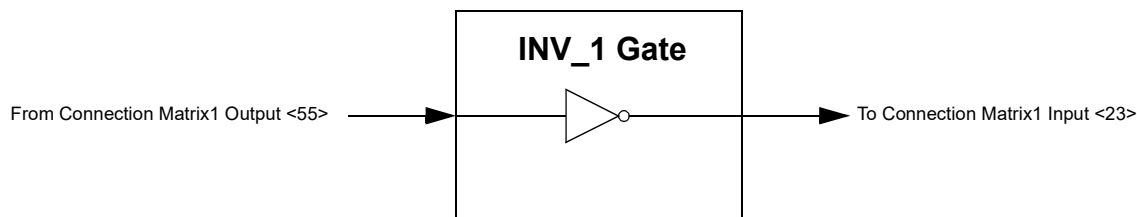
Figure 131. INV_1 Gate
