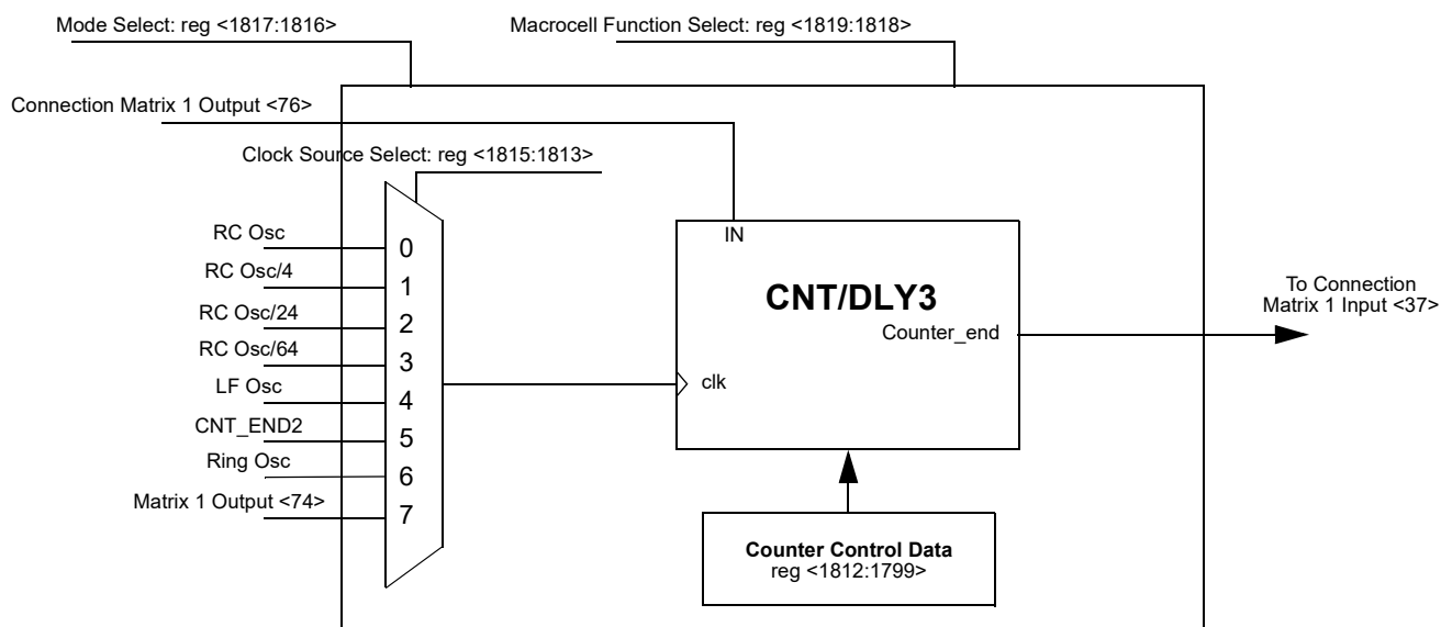
Figure 80. CNT/DLY3
