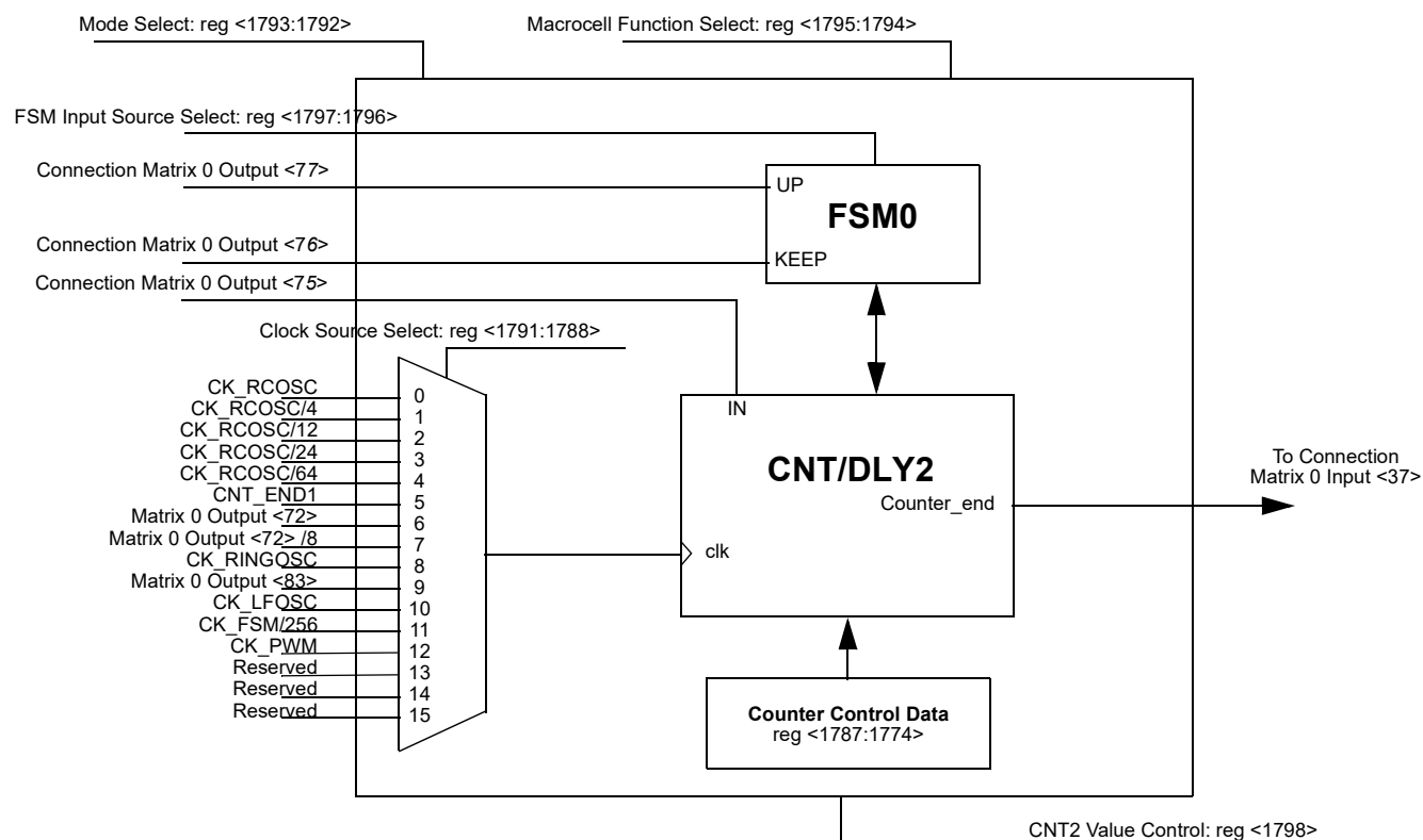
Figure 79. CNT/DLY2/FSM0
