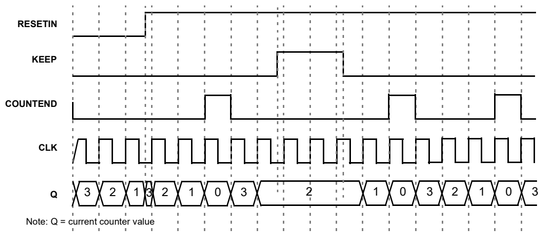
Figure 93. Timing (set rising edge mode, oscillator is forced on, UP=0) for count data = 3
