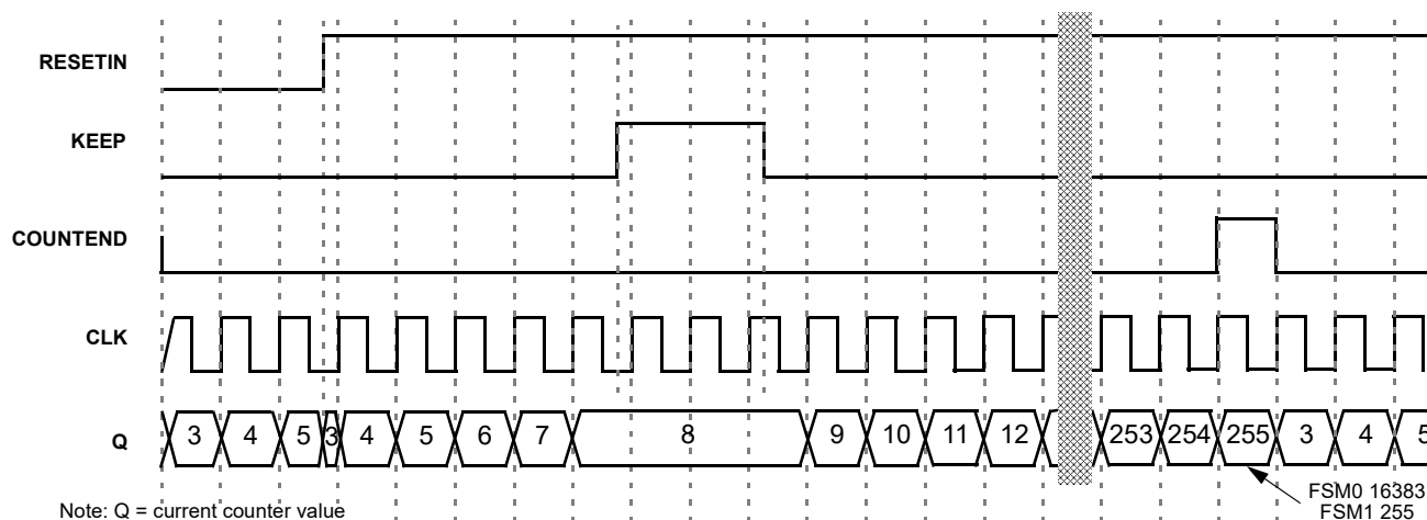
Figure 95. Timing (set rising edge mode, oscillator is forced on, UP=1) for count data = 3
