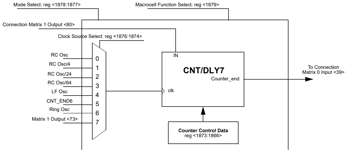
Figure 84. CNT/DLY7
