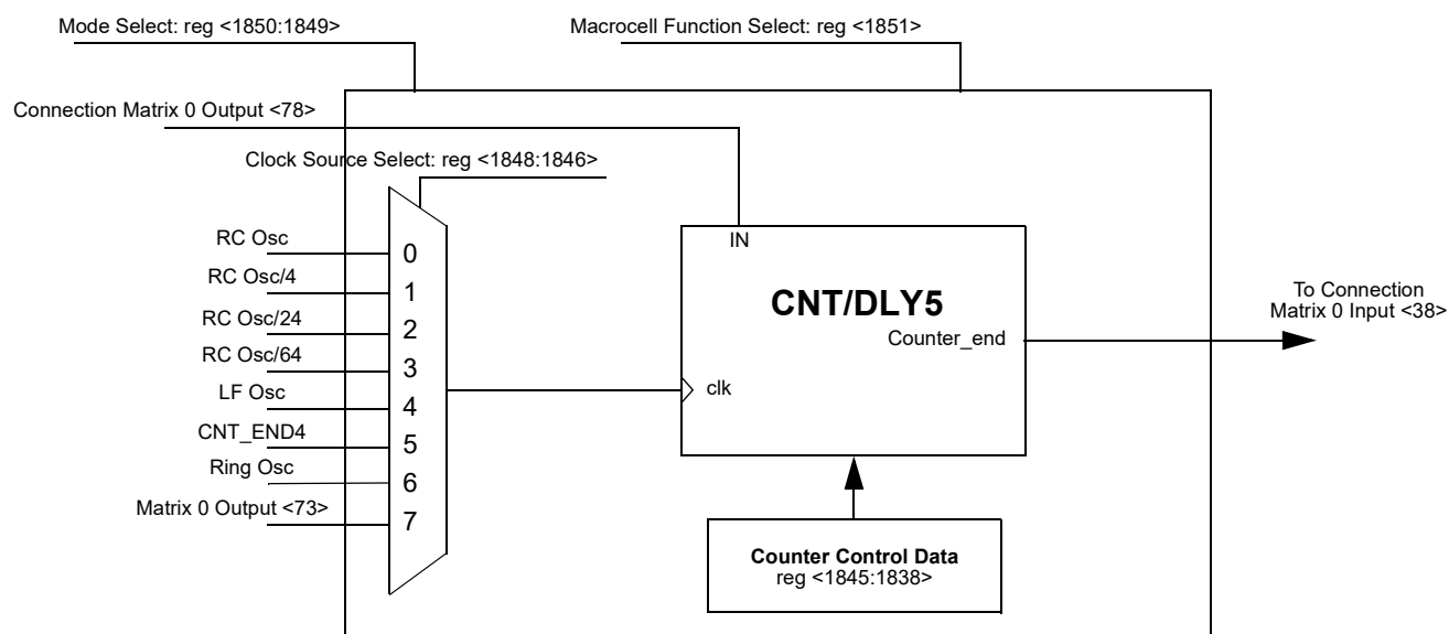
Figure 82. CNT/DLY5
