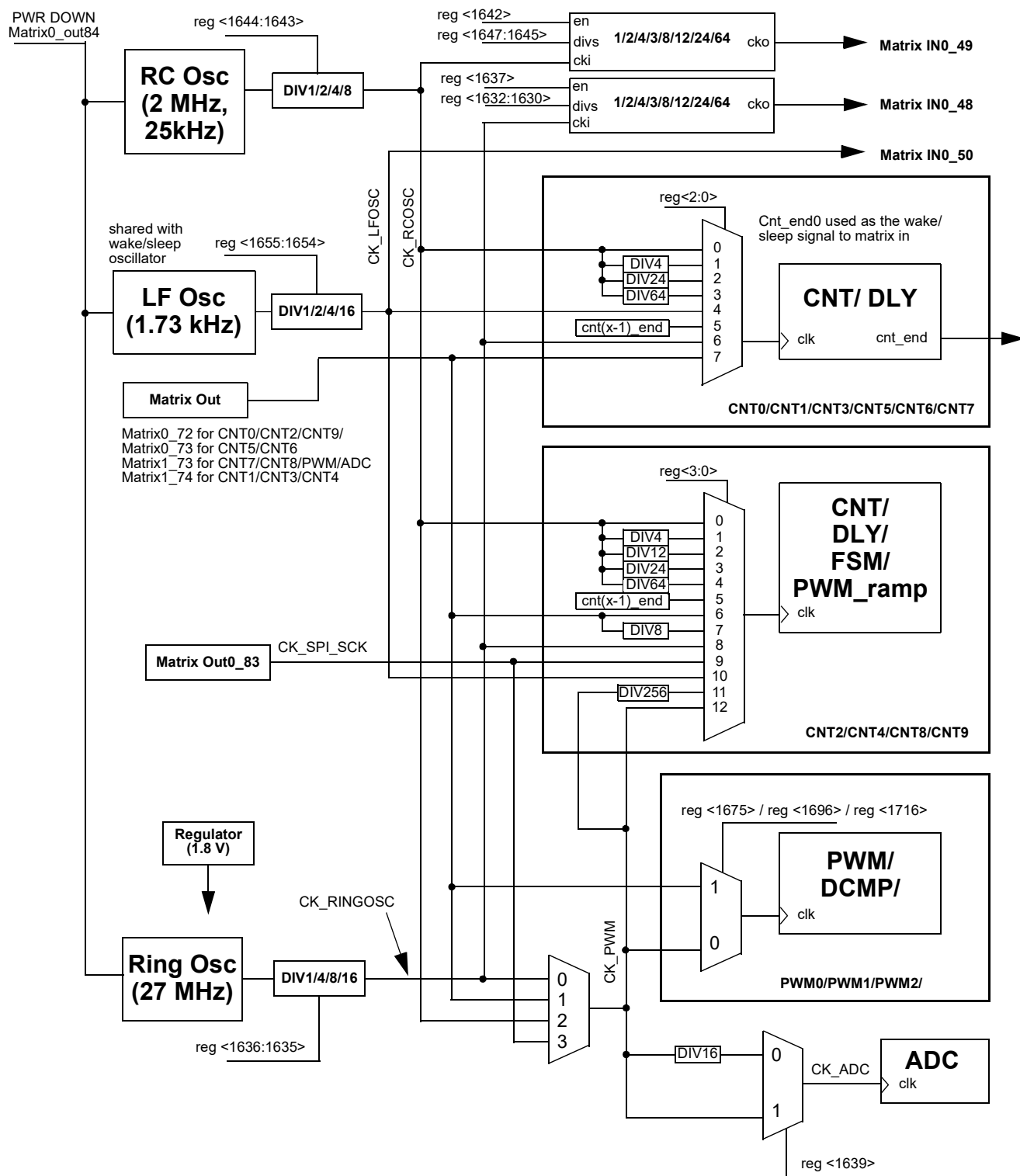
Figure 114. Oscillator Block Diagram
