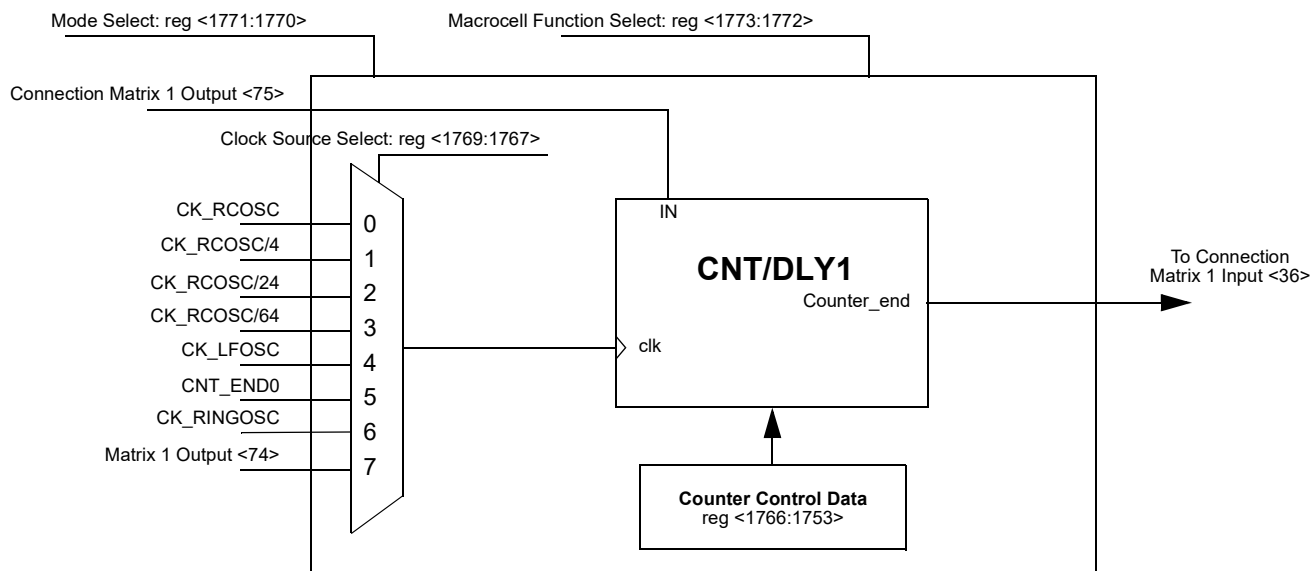
Figure 78. CNT/DLY1
