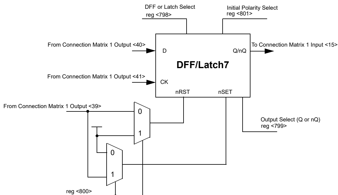
Figure 69. DFF/Latch7
