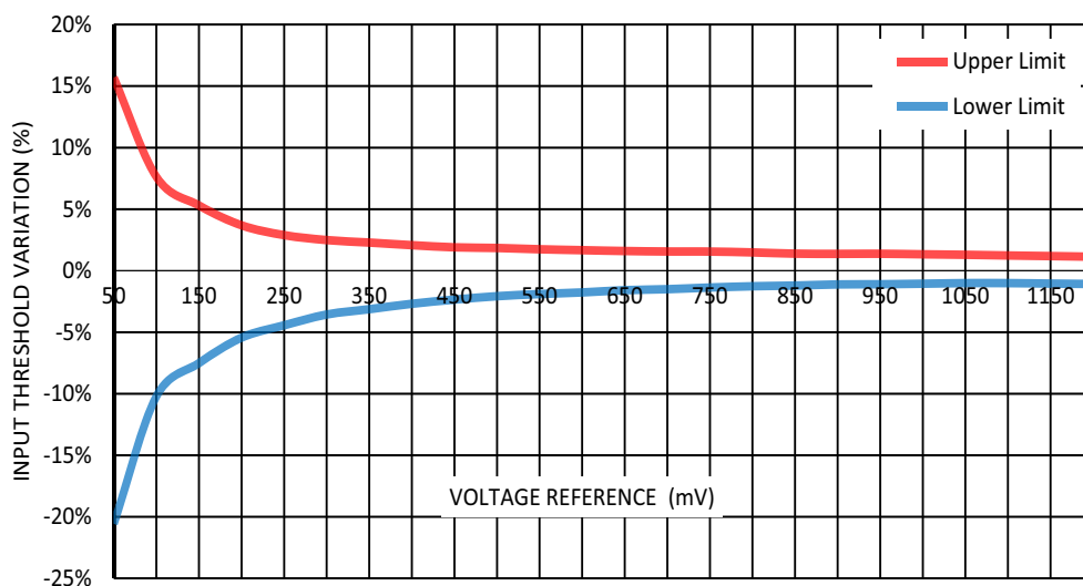
Figure 54. Input Threshold Variation (including V_{\text{ref}} variation, ACMP offset) vs. Voltage Reference at T = (-40.... +85)^{\circ}\text{C} , LMB Mode - Disable, V_{\text{phys}} = 0 \text{ mV} .
