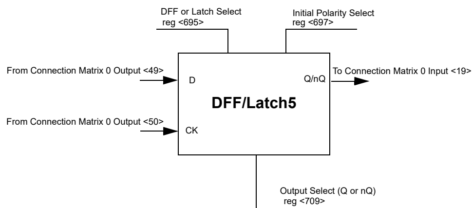
Figure 67. DFF/Latch5
