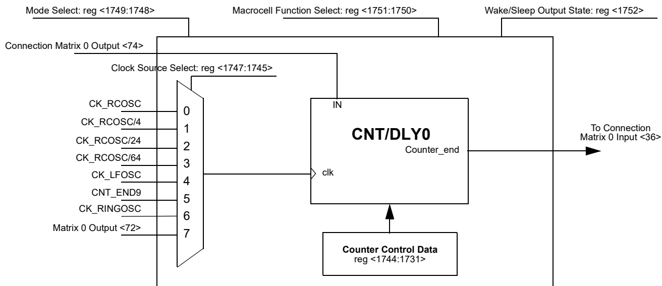
Figure 77. CNT/DLY0
