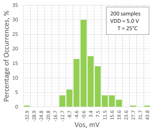
Figure 15. PGA Input Offset Distribution, Single-Ended Mode, G = 0.25
