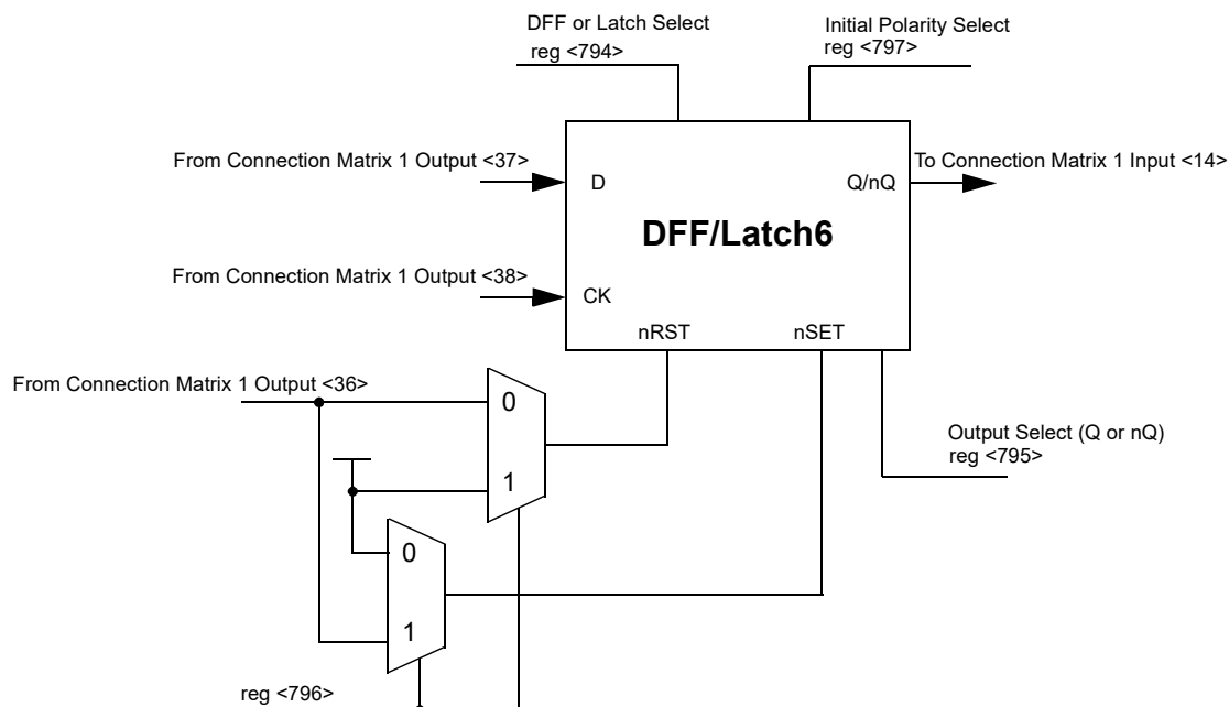
Figure 68. DFF/Latch6
