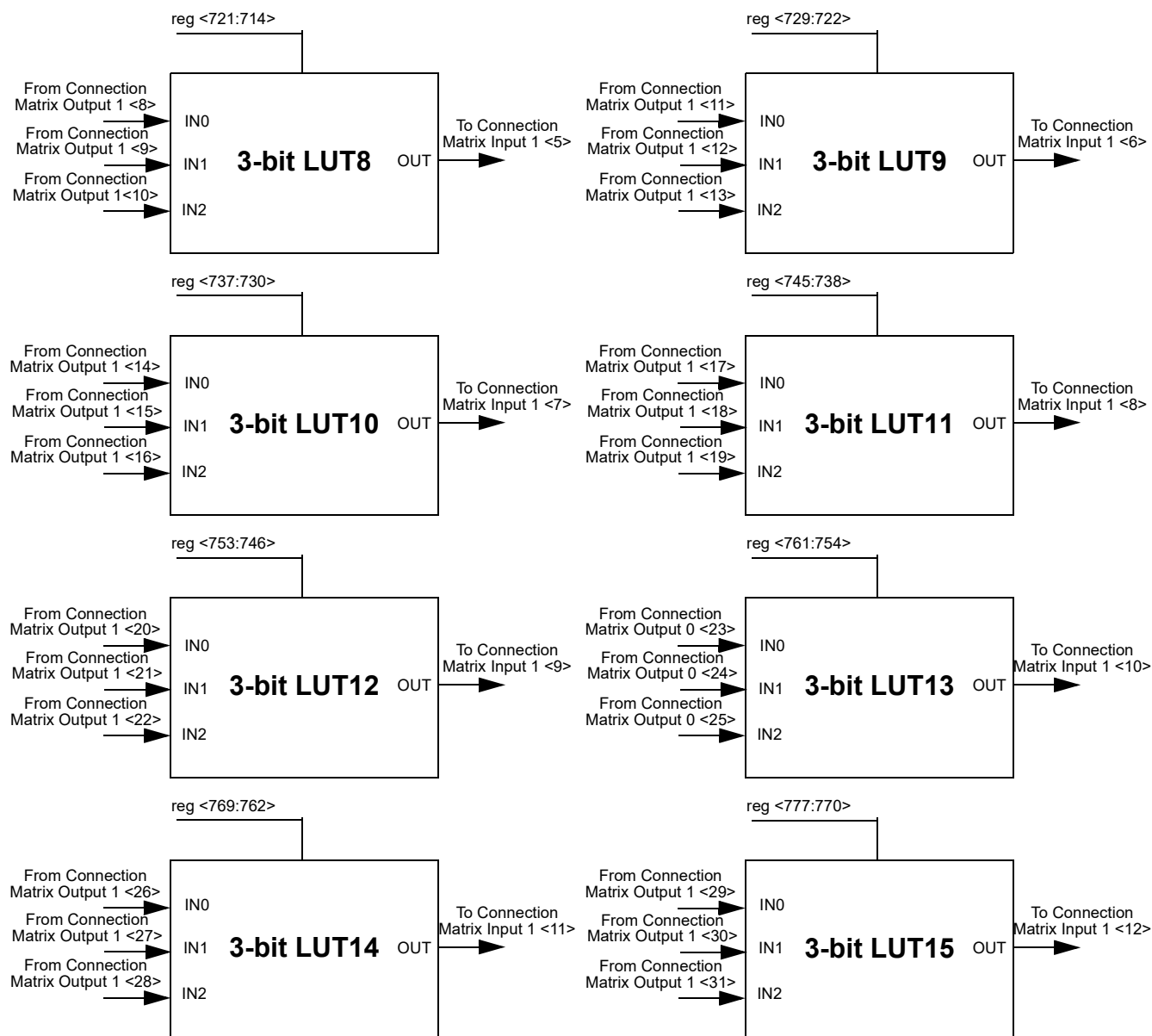
Figure 44. 3-bit LUTs
