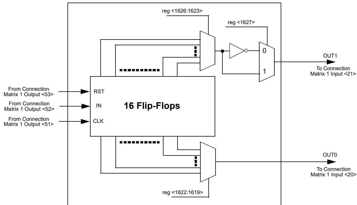
Figure 107. Pipe Delay 1
