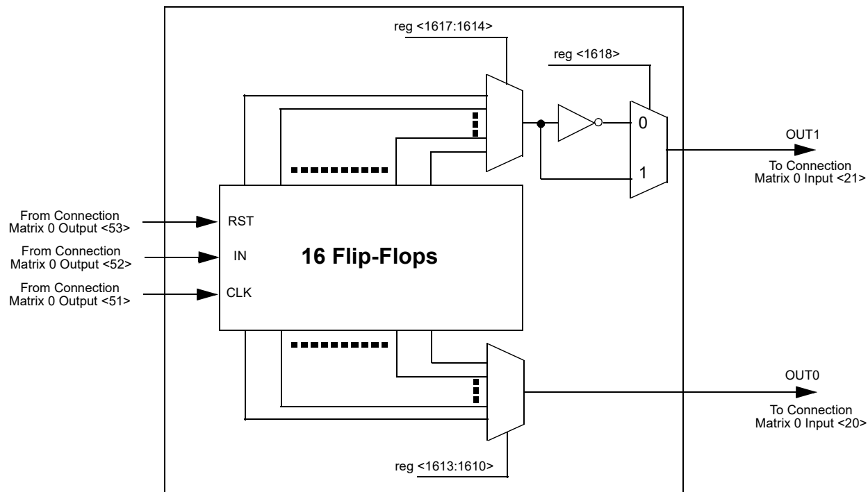
Figure 106. Pipe Delay 0
