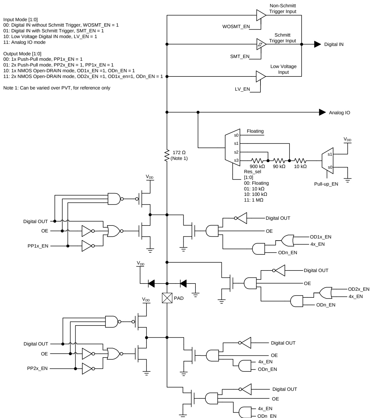
Figure 5. Matrix OE IO 4x Drive Structure Diagram
