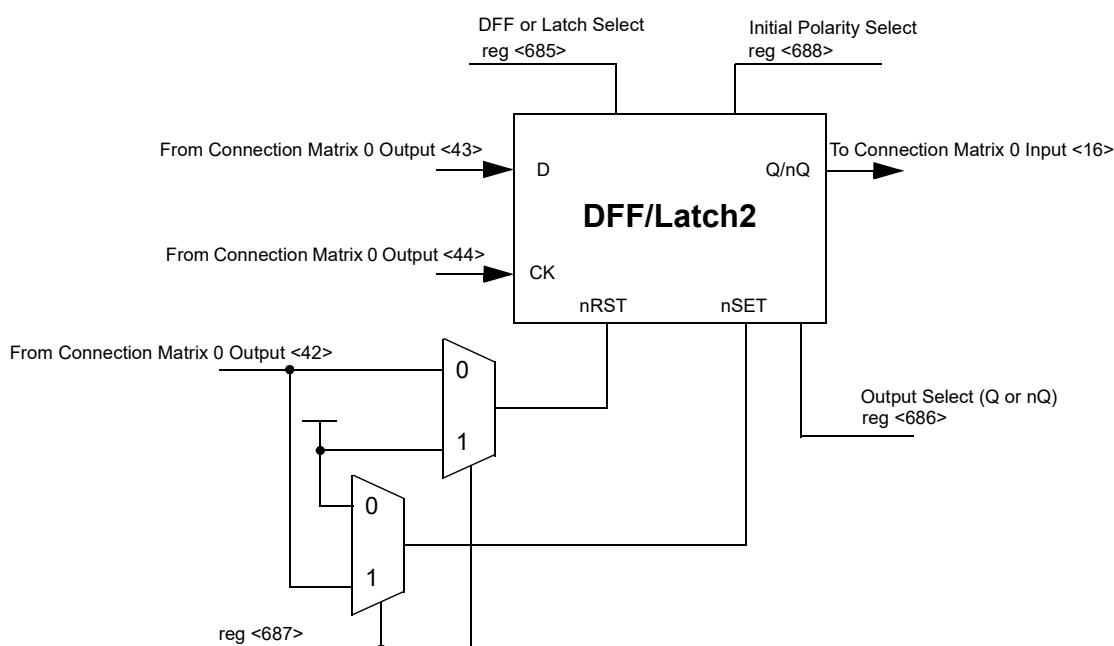
Figure 64. DFF/Latch2
