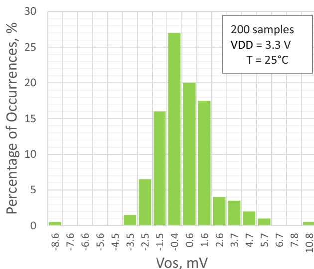
Figure 17. PGA Input Offset Distribution, Single-Ended Mode, G = 1
