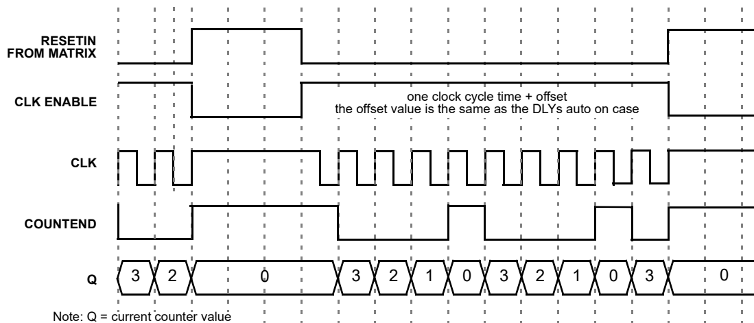
Figure 91. Timing (reset high level mode, oscillator is autopowered on (controlled by reset)) for count data = 3
