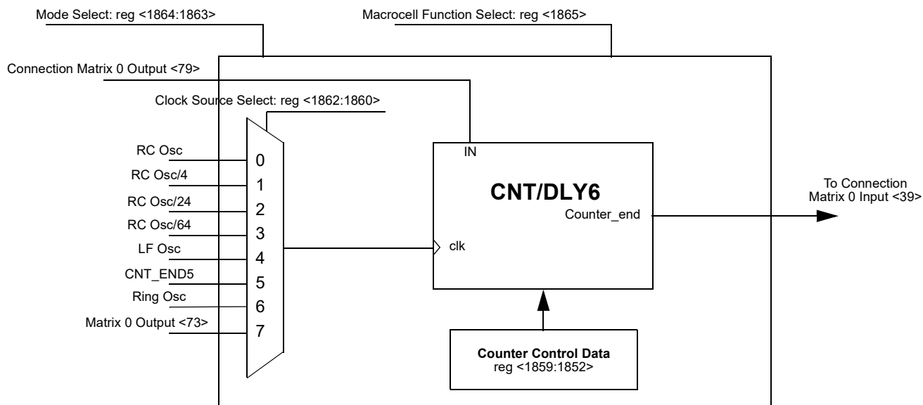
Figure 83. CNT/DLY6
