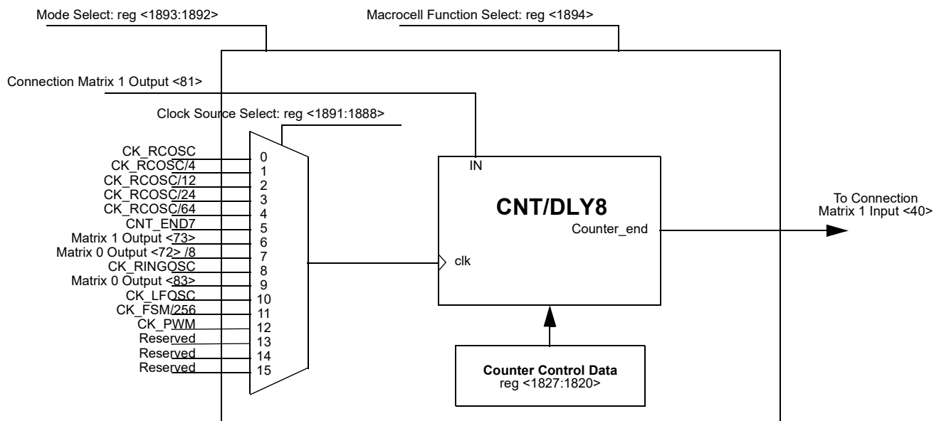
Figure 85. CNT/DLY8/PWM_RAMP
