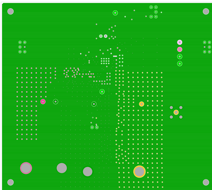
Figure 9. PCB - Layer 2
