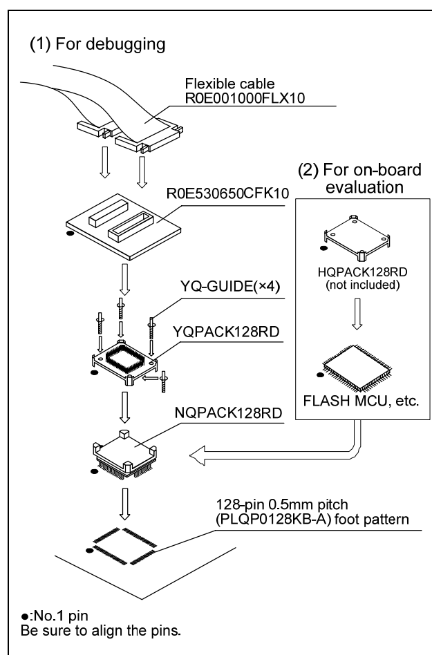
Figure 2 Usage of the R0E530650CFK10
