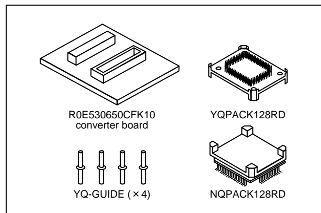
Figure 1 Package components of the R0E530650CFK10
