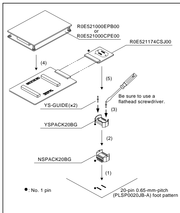
Figure 3 Connection procedure of the R0E521174CSJ00
