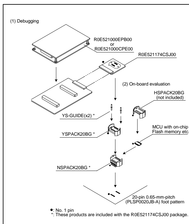
Figure 2 Usage of the R0E521174CSJ00
