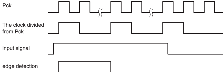
Figure 16.2 Edge Detection
