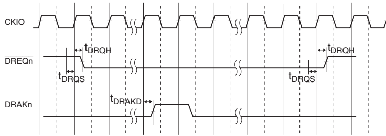
Figure 33.50 \overline{\text{DREQ}}/\text{DRAK} Timing
