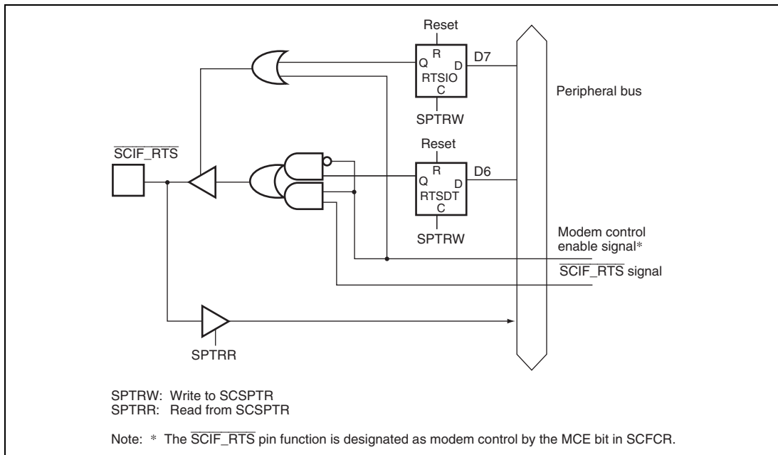
Figure 17.2 SCIF_RTSS Pin (Only in Channels 1 and 2)
