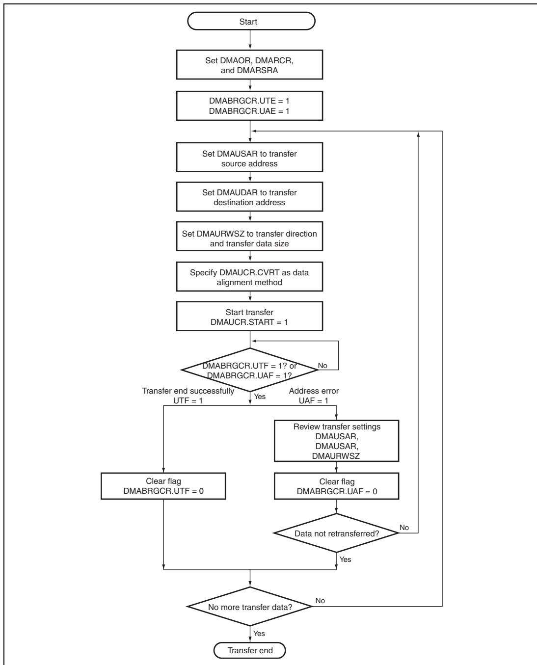
Figure 11.39 DMA Transfer Flow Shared Memory ↔ Synchronous DRAM
