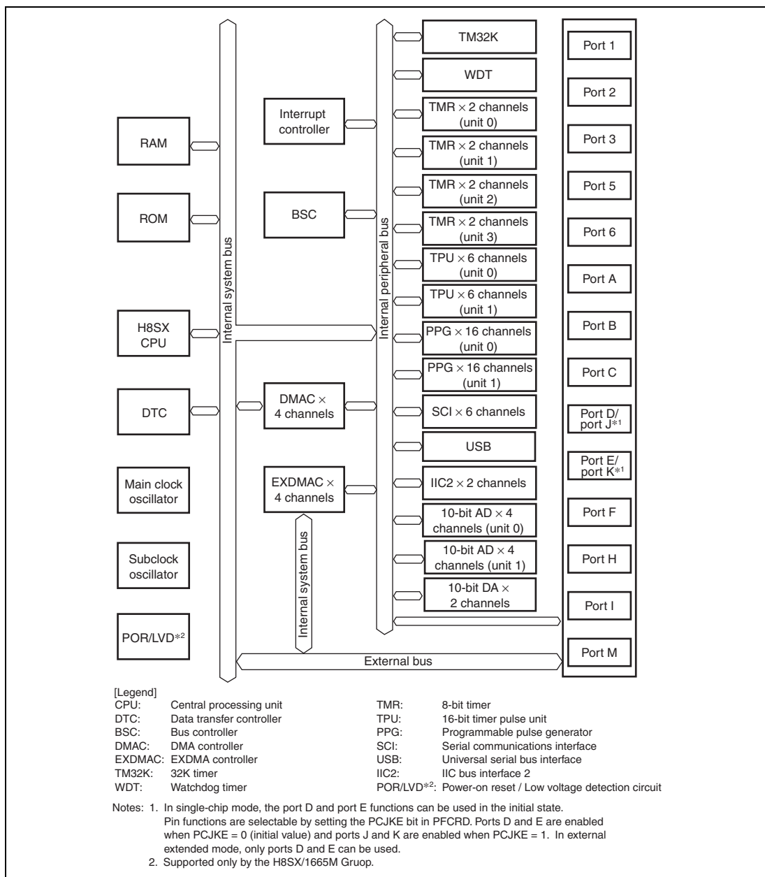
Figure 1.2 Block Diagram
