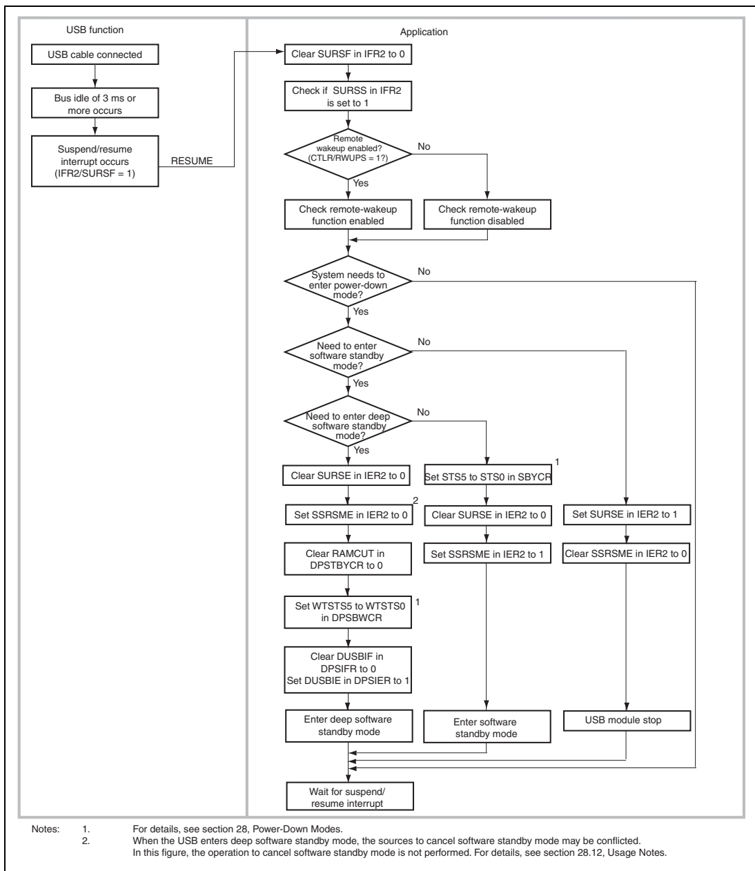
Figure 20.4 Suspend Operation
