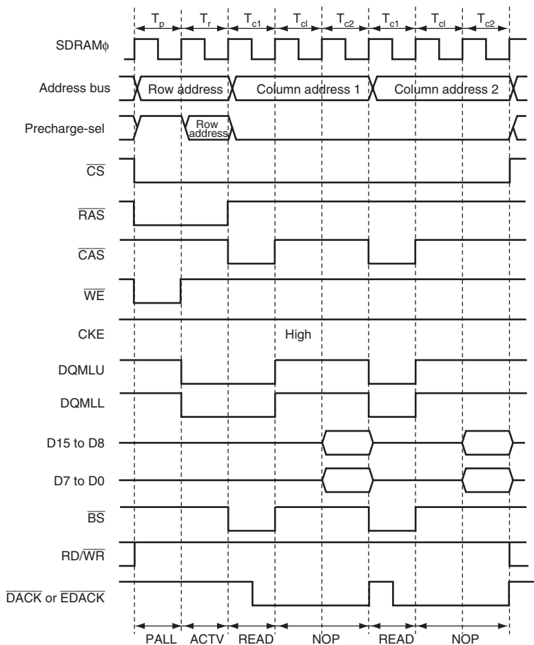
Figure 9.84 Output Timing Example of \overline{\text{DACK}} and \overline{\text{EDACK}} when DDS = 1 or EDDS = 1 (Read, CAS Latency = 2)
