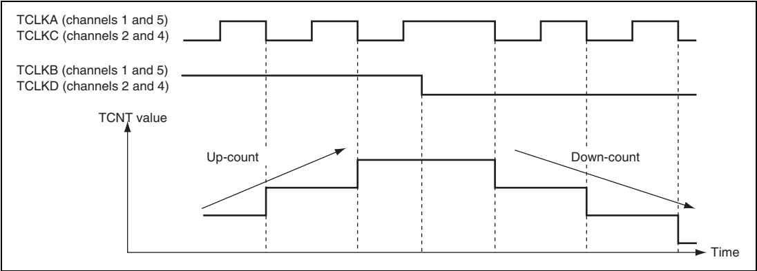
Figure 14.27 Example of Phase Counting Mode 2 Operation
