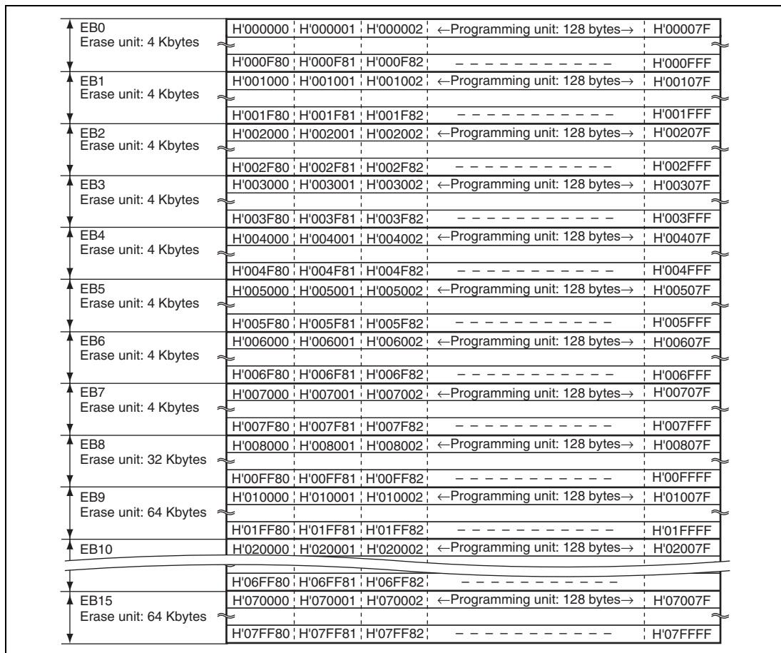
Figure 25.4 (2) User MAT Block Structure of H8SX/1665
