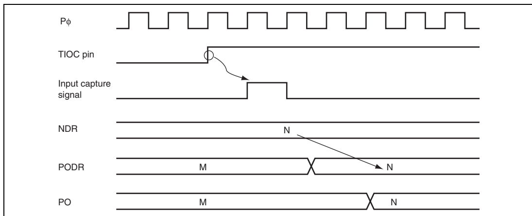
Figure 15.14 Pulse Output Triggered by Input Capture (Example)
