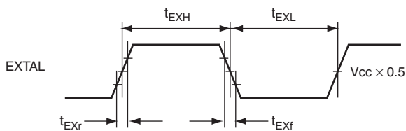
Figure 30.5 External Input Clock Timing
