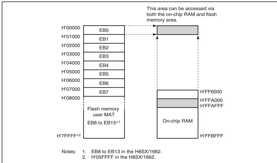
Figure 25.20 Address Map of Overlaid RAM Area (H8SX/1665)
