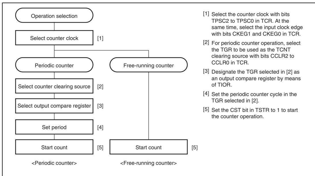
Figure 14.3 Example of Counter Operation Setting Procedure
