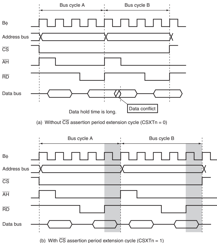
Figure 9.36 Consecutive Read Accesses to Same Area (Address/Data Multiplexed I/O Space)
