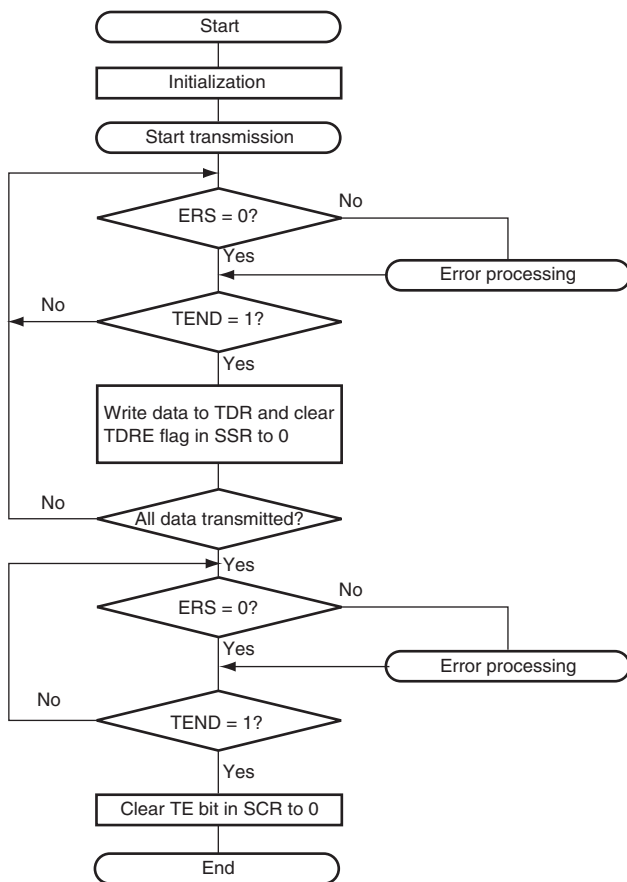
Figure 19.31 Sample Transmission Flowchart
