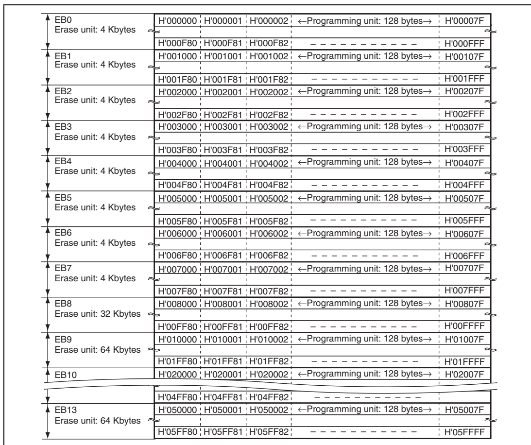
Figure 25.4 (1) User MAT Block Structure of H8SX/1662
