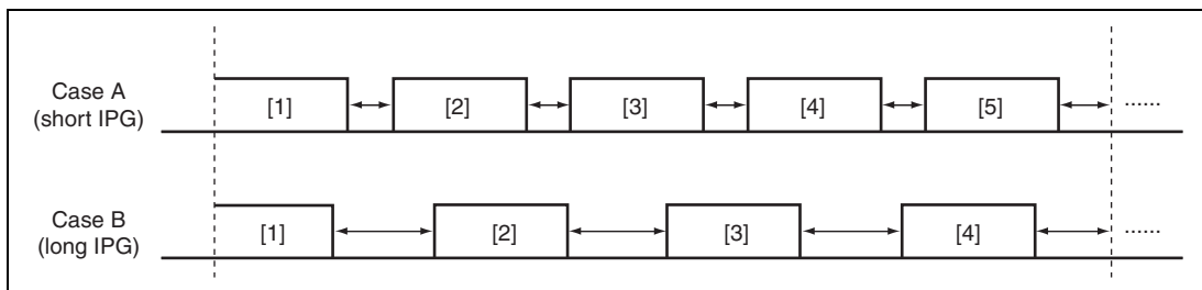
Figure 20.12 Changing IPG and Transmission Efficiency
