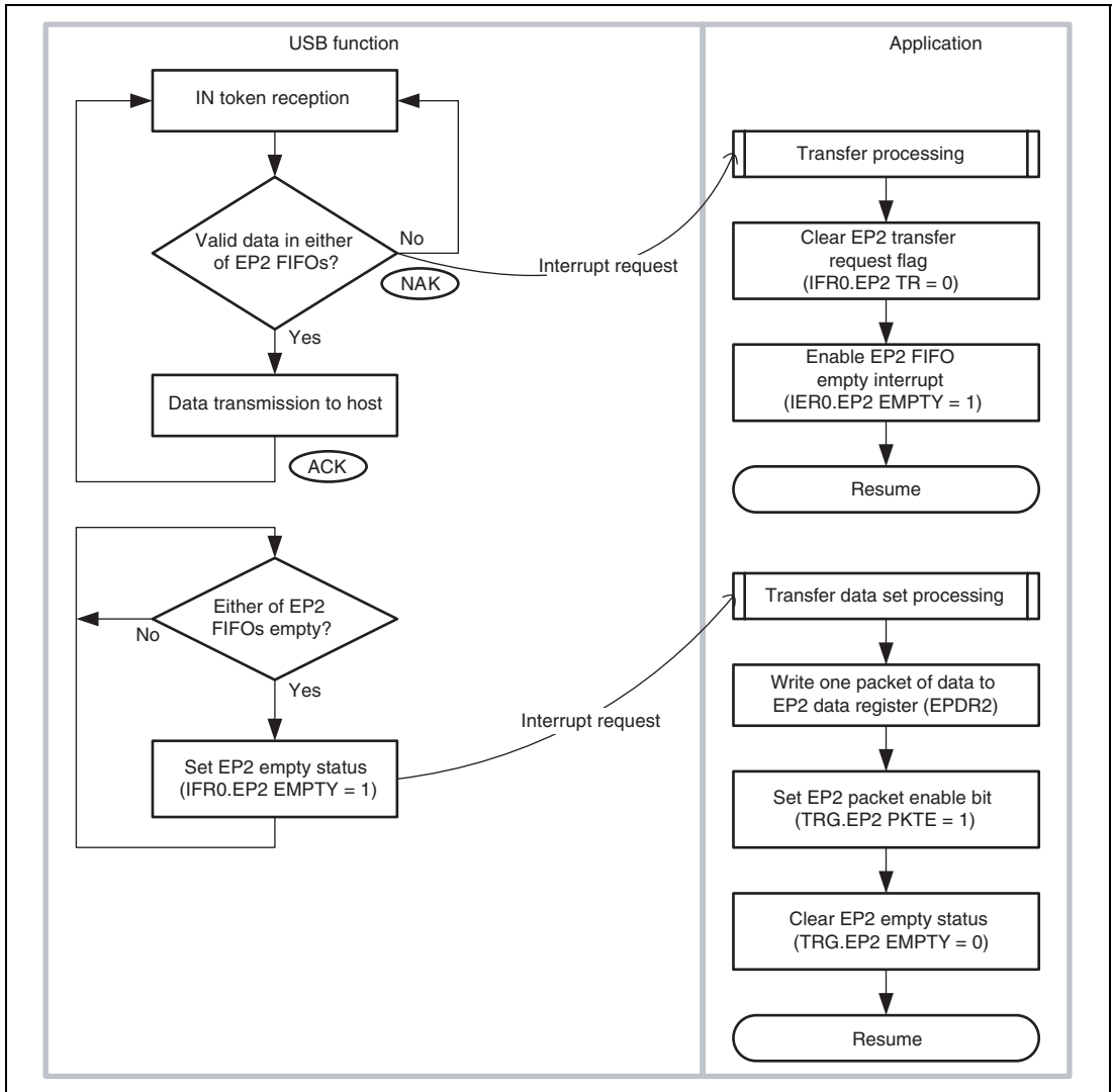
Figure 22.16 EP2 Bulk-In Transfer Operation
