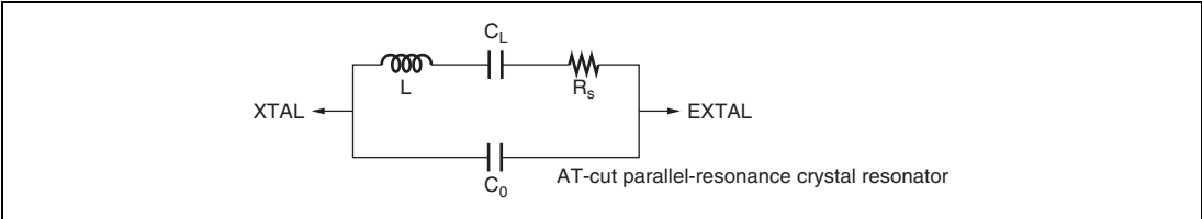
Figure 27.3 Equivalent Circuit of Crystal Resonator
