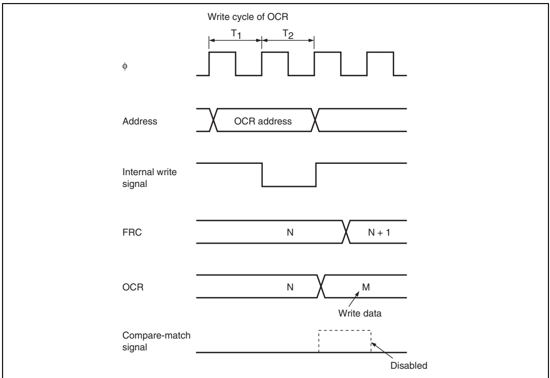
Figure 10.10 Conflict between OCR Write and Compare-Match (When Automatic Addition Function is Not Used)
