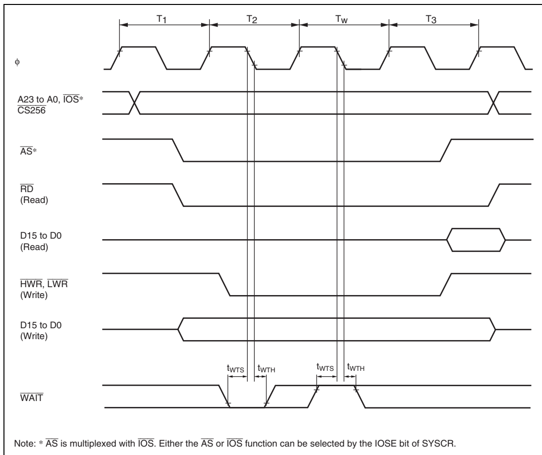
Figure 31.14 Basic Bus Timing/3-State Access with One Wait State
