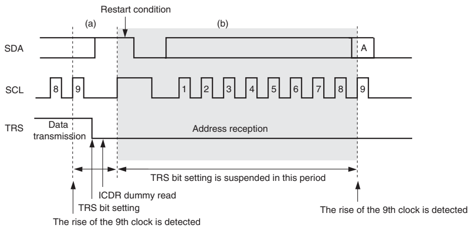
Figure 18.34 TRS Bit Set Timing in Slave Mode
