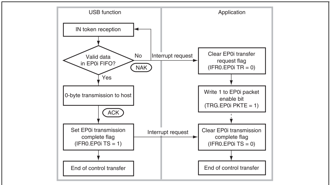
Figure 22.14 Status Stage (Control-Out) Operation
