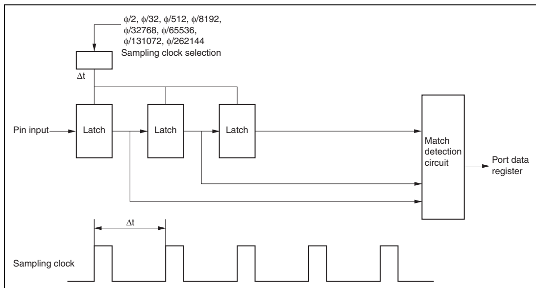
Figure 8.11 Noise Canceler Circuit
