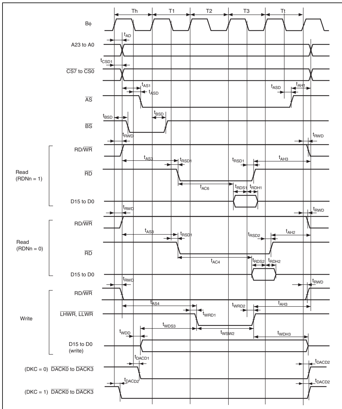
Figure 27.12 Basic Bus Timing: Three-State Access ( \overline{CS} Assertion Period Extended)
