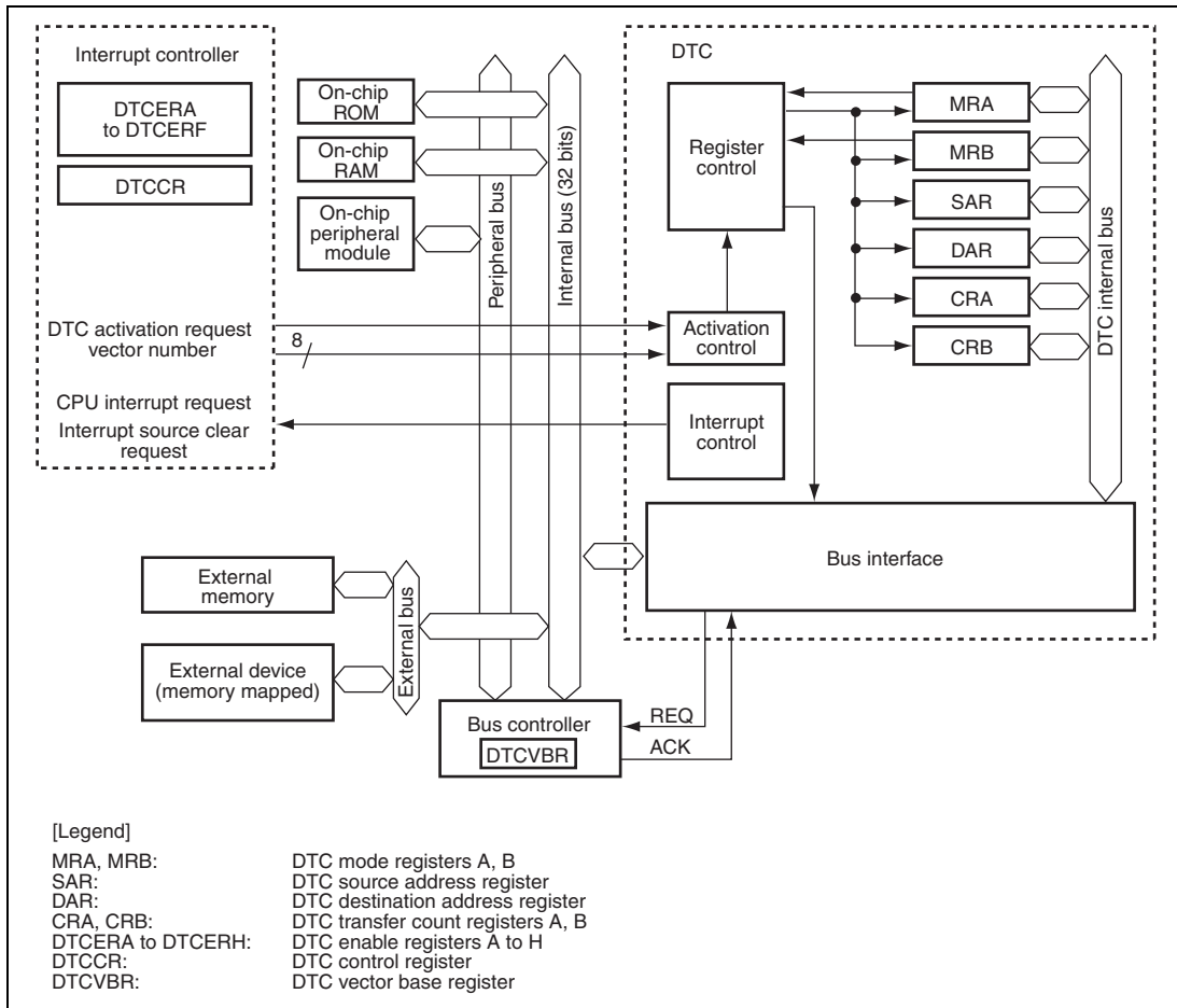
Figure 11.1 Block Diagram of DTC
