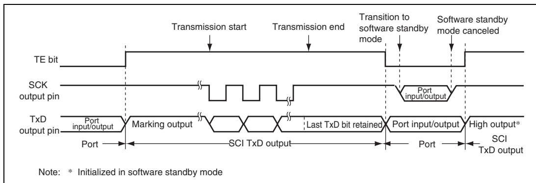
Figure 17.41 Port Pin States during Software Standby Mode Transition (Internal Clock, Clock Synchronous Transmission)
