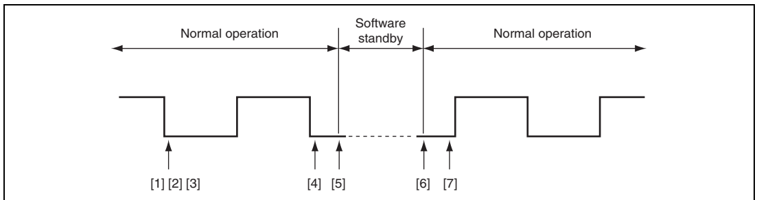
Figure 17.35 Clock Stop and Restart Procedure
