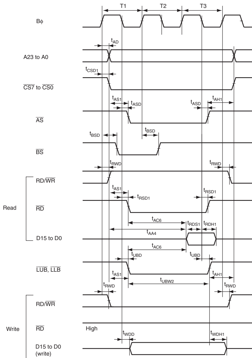
Figure 27.14 Byte Control SRAM: Three-State Read/Write Access
