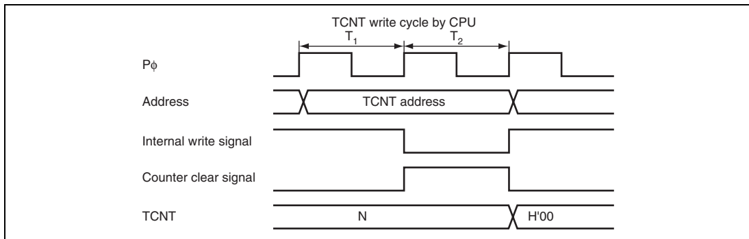
Figure 15.15 Conflict between TCNT Write and Clear
