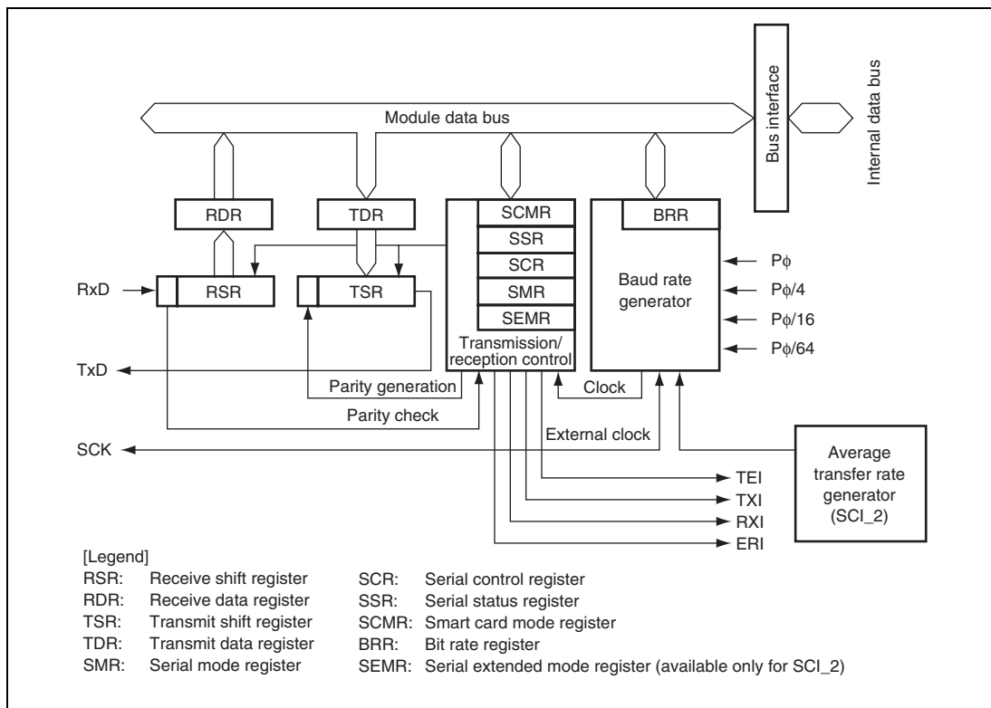
Figure 17.1 Block Diagram of SCI_0, 1, 2, 3, and 4
