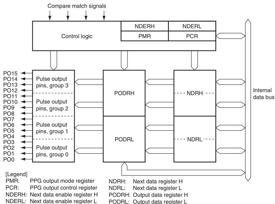
Figure 14.1 Block Diagram of PPG (Unit 0)
