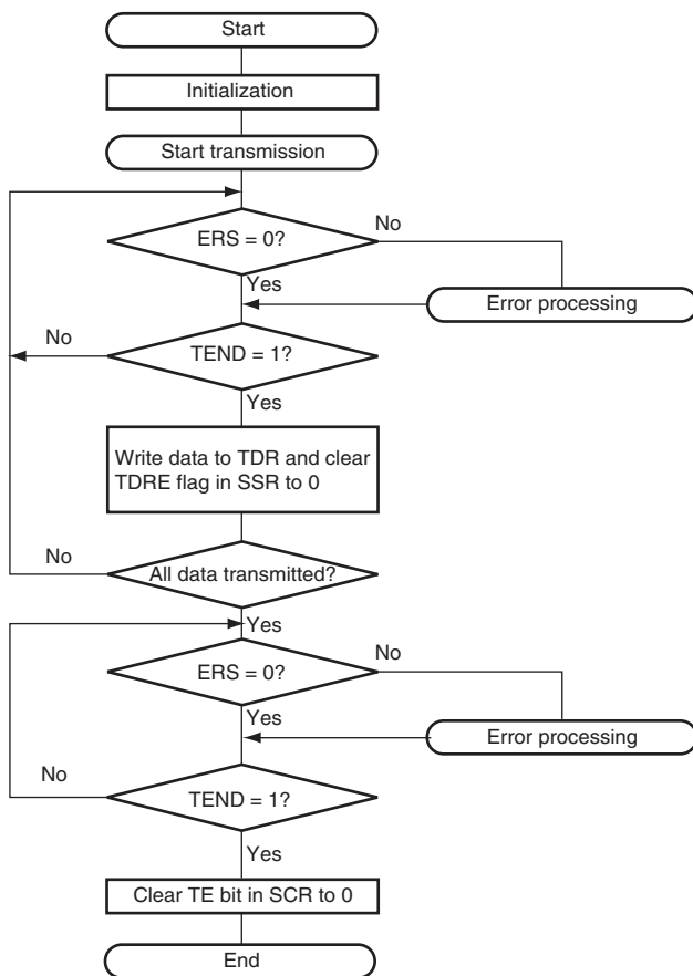
Figure 17.31 Sample Transmission Flowchart
