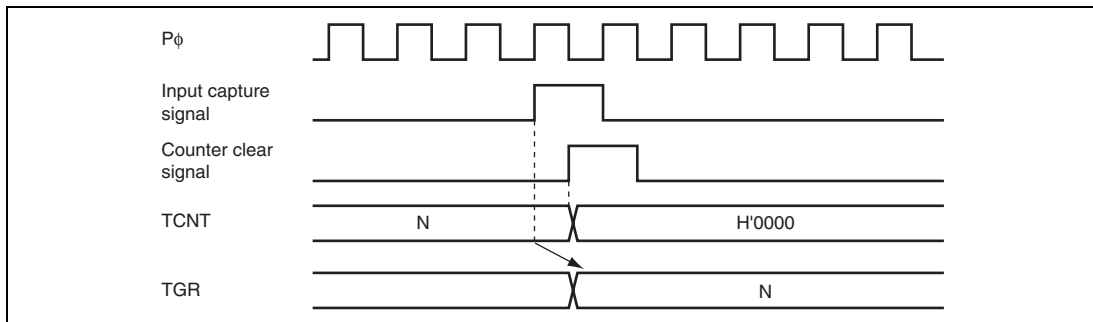
Figure 13.36 Counter Clear Timing (Input Capture)
