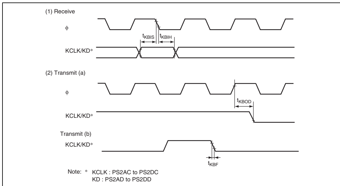
Figure 26.22 PS2 Timing
