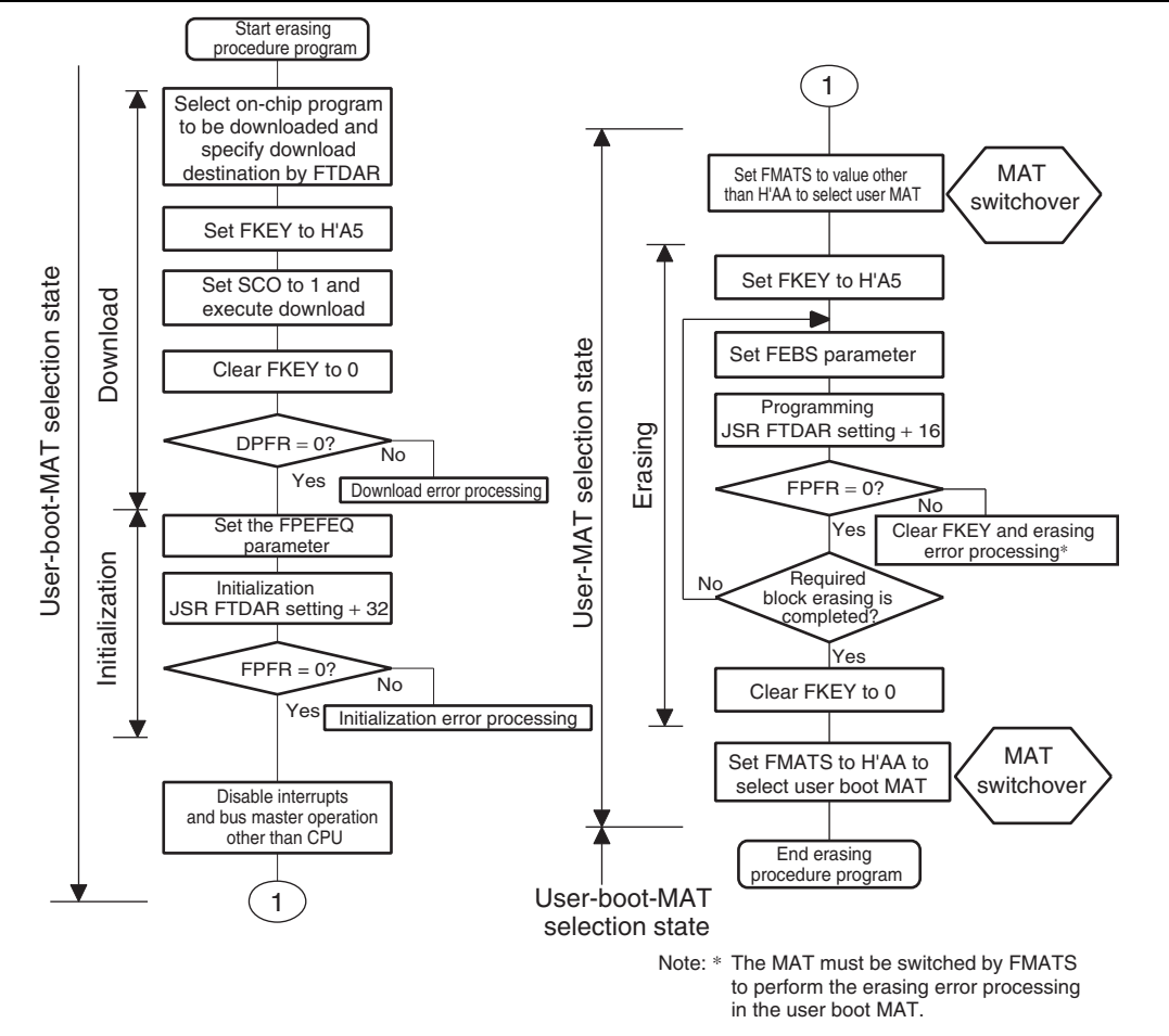
Figure 22.15 Procedure for Erasing User MAT in User Boot Mode
