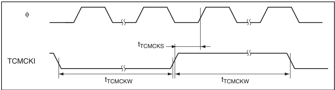
Figure 26.16 TCM Clock Input Timing
