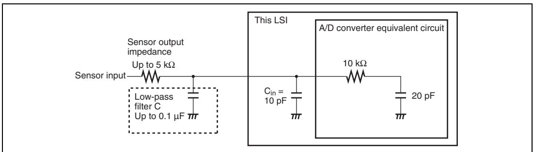
Figure 20.5 Example of Analog Input Circuit
