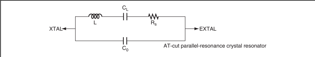
Figure 23.3 Equivalent Circuit of Crystal Resonator
