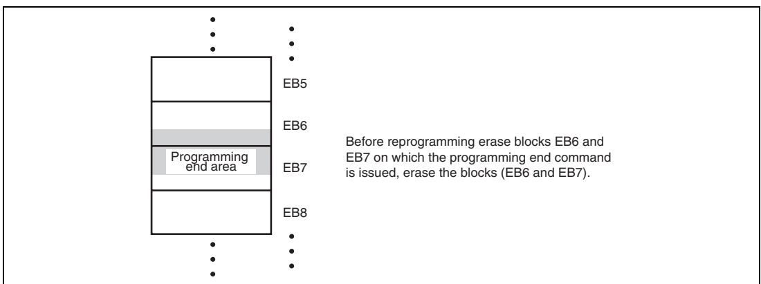
Figure 22.9 Example of Erase Block Including Programmed Area
