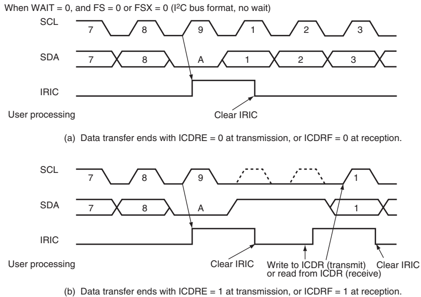
Figure 17.18 IRIC Setting Timing and SCL Control (1)
