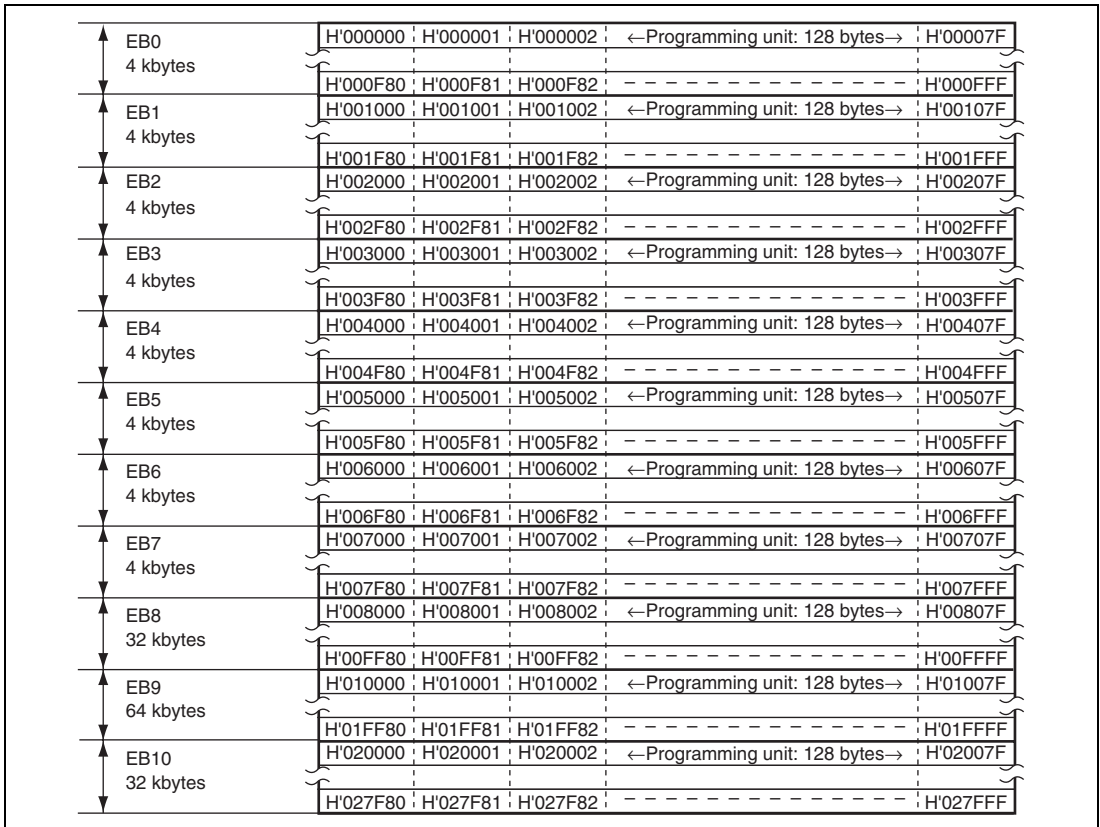
Figure 22.4 Block Structure of the User MAT
