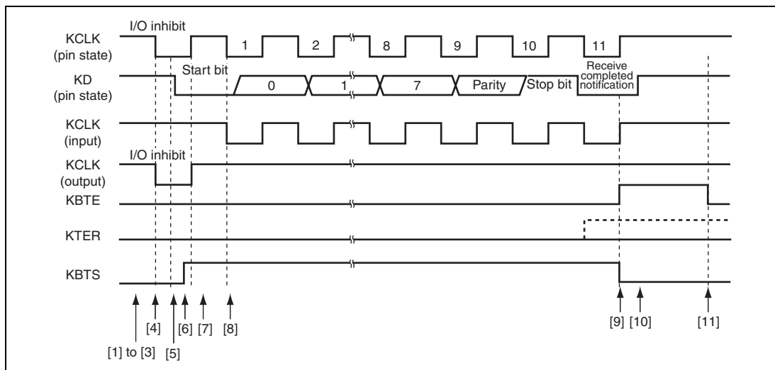
Figure 18.6 Transmit Timing
