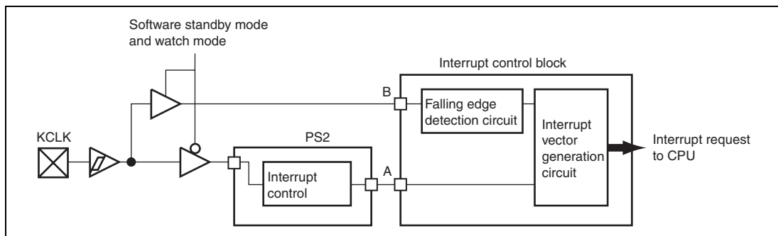
Figure 18.16 First KCLK Interrupt Path
