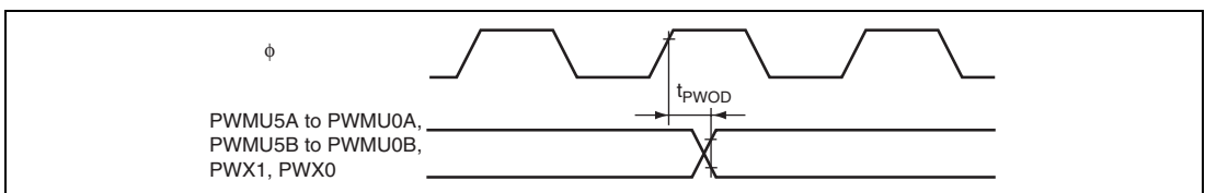
Figure 26.19 PWMU, PWMX Output Timing
