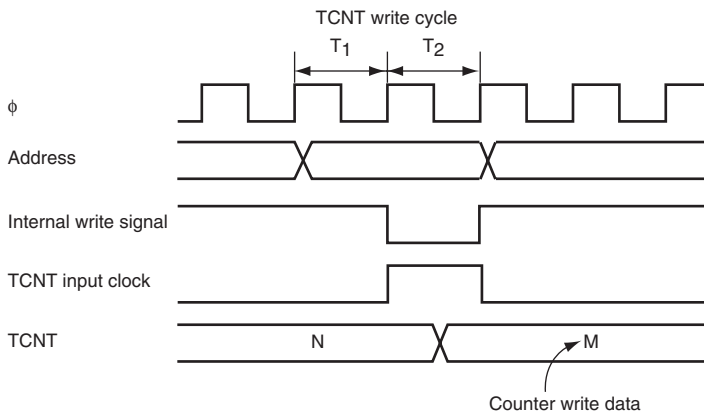
Figure 14.6 Conflict between TCNT Write and Increment
