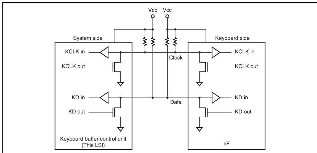
Figure 18.2 PS2 Connection
