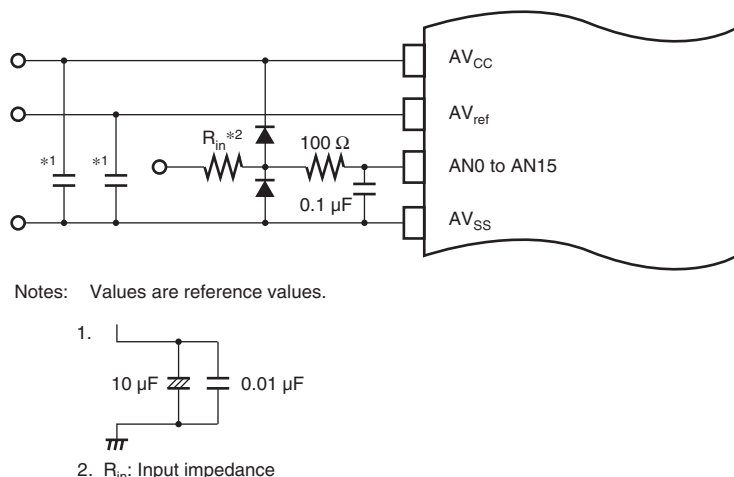
Figure 20.6 Example of Analog Input Protection Circuit
