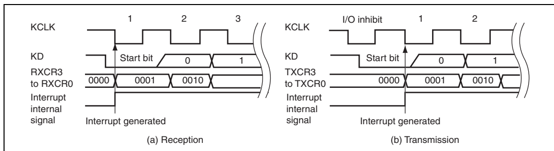
Figure 18.15 Timing of First KCLK Interrupt
