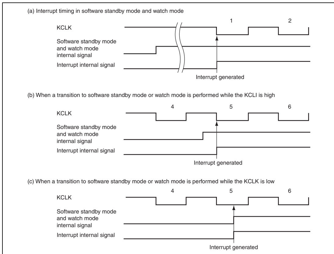
Figure 18.17 Interrupt Timing in Software Standby Mode and Watch Mode
