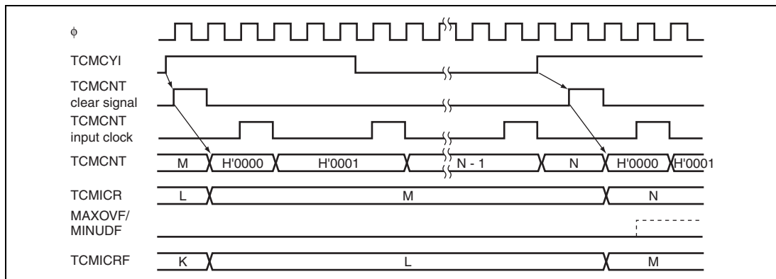
Figure 11.8 Example of Timing in Cycle Measurement
