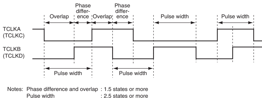
Figure 10.43 Phase Difference, Overlap, and Pulse Width in Phase Counting Mode
