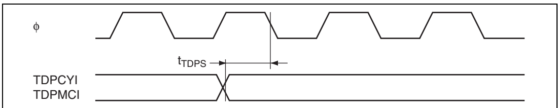
Figure 26.17 TDP Input Setup Time
