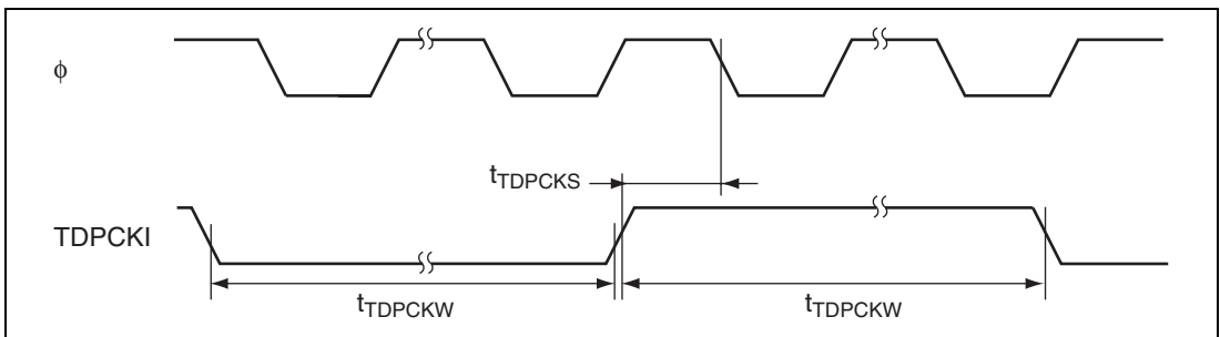
Figure 26.18 TDP Clock Input Timing
