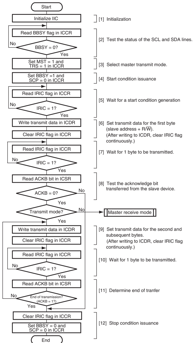
Figure 17.7 Sample Flowchart for Operations in Master Transmit Mode
