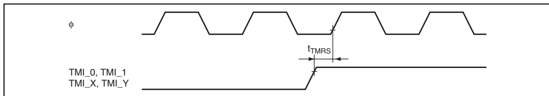
Figure 26.14 8-Bit Timer Reset Input Timing
