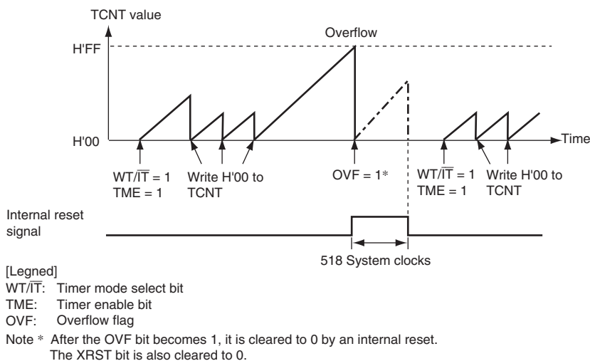
Figure 14.2 Watchdog Timer Mode ( \text{RST}/\overline{\text{NMI}} = 1 ) Operation
