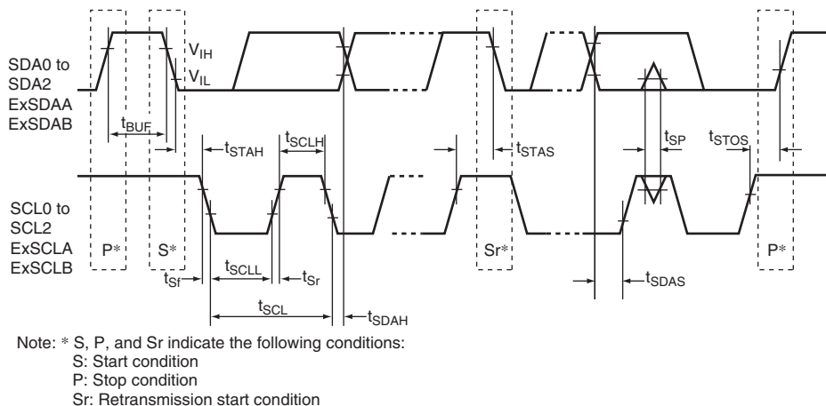
Figure 26.23 I 2 C Bus Interface Input/Output Timing
