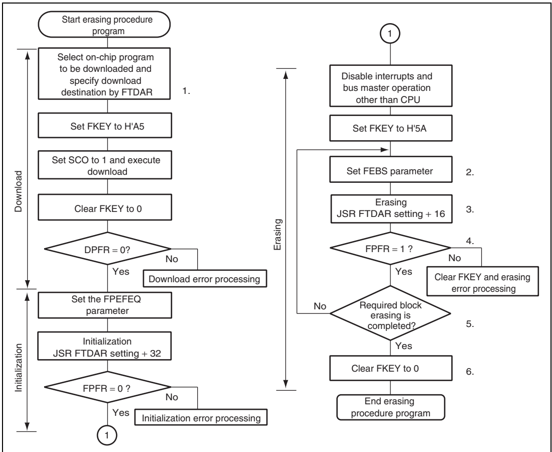
Figure 22.13 Erasing Procedure in User Program Mode
