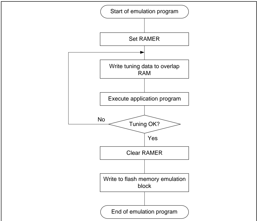
Figure 19.16 Flowchart of Flash Memory Emulation in RAM
