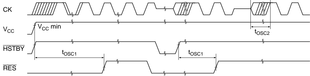
Figure 22.4 Oscillation Settling Time
