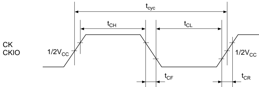
Figure 22.2 System Clock Timing
