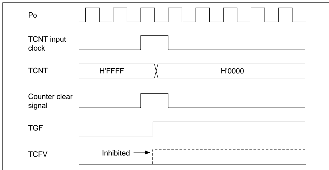
Figure 10.55 Contention between Overflow and Counter Clearing
