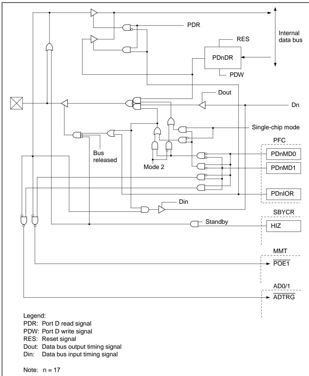
Figure C.24 PD17/D17/ \overline{\text{POE1}} /ADTRG Block Diagram
