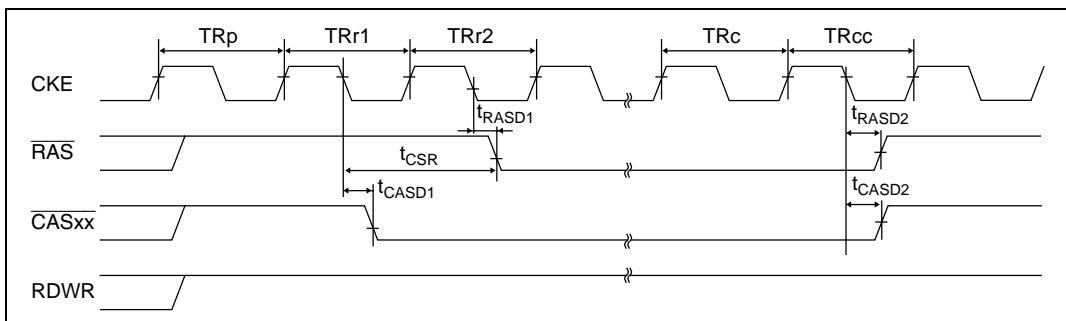
Figure 22.18 Self-Refresh
