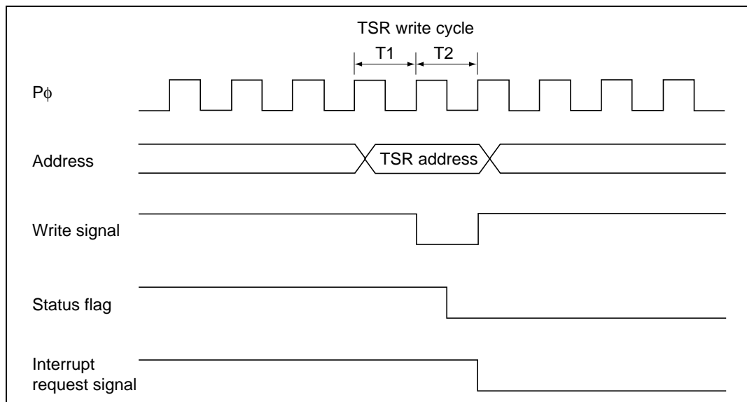
Figure 11.13 Timing of Status Flag Clearing by CPU
