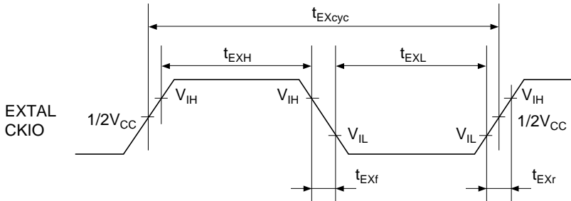
Figure 22.3 EXTAL Clock Input Timing
