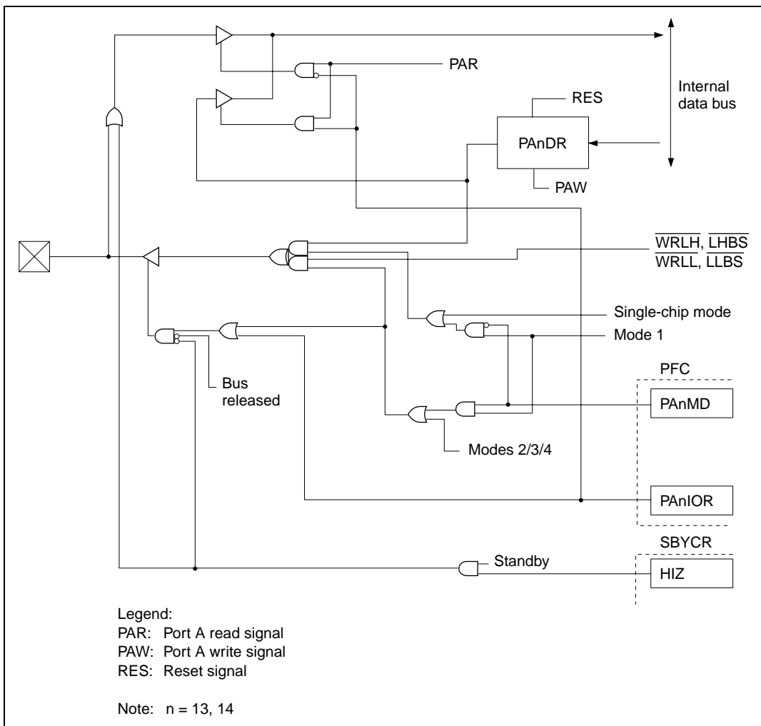
Figure C.3 PA13/ \overline{\text{WRLH}}/\text{LHBS} , PA14/ \overline{\text{WRLH}}/\text{LHBS} Block Diagram
