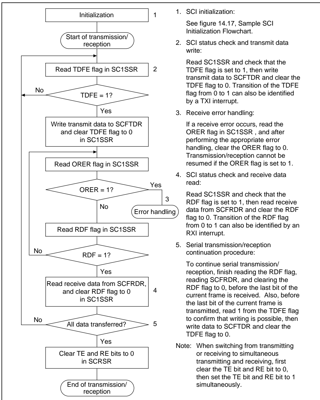
Figure 14.23 Sample Flowchart for Serial Transmission and Reception
