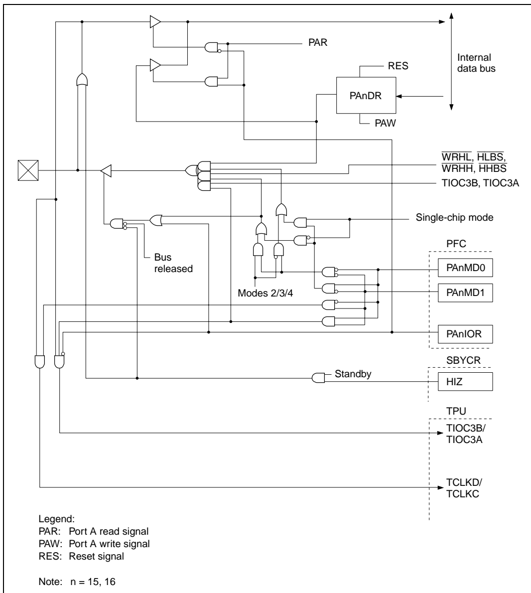
Figure C.4 PA15/ \overline{\text{WRHL}} / \overline{\text{HLBS}} /TCLKD/TIOC3B, PA16/ \overline{\text{WRHH}} / \overline{\text{HHBS}} /TCLKC/TIOC3A Block Diagram
