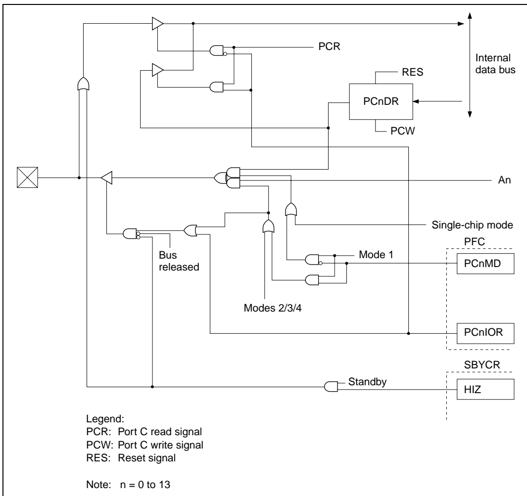
Figure C.13 PCn/An Block Diagram (for Mask ROM version)
