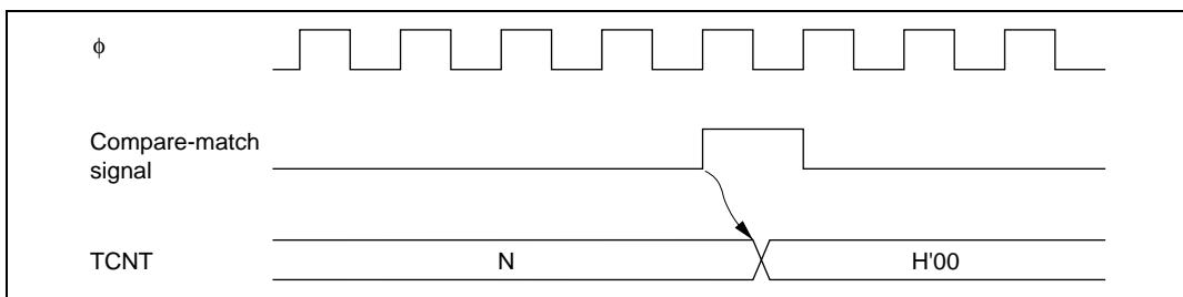
Figure 12.6 Timing of Compare-Match Clear
