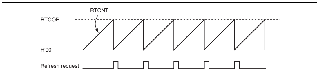
Figure 6.52 RTCNT Operation
