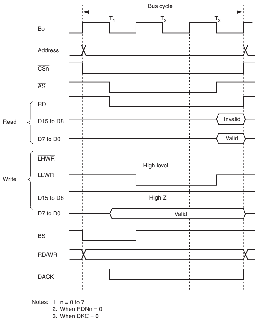
Figure 6.19 16-Bit 3-State Access Space Bus Timing (Word Access for Odd Address)
