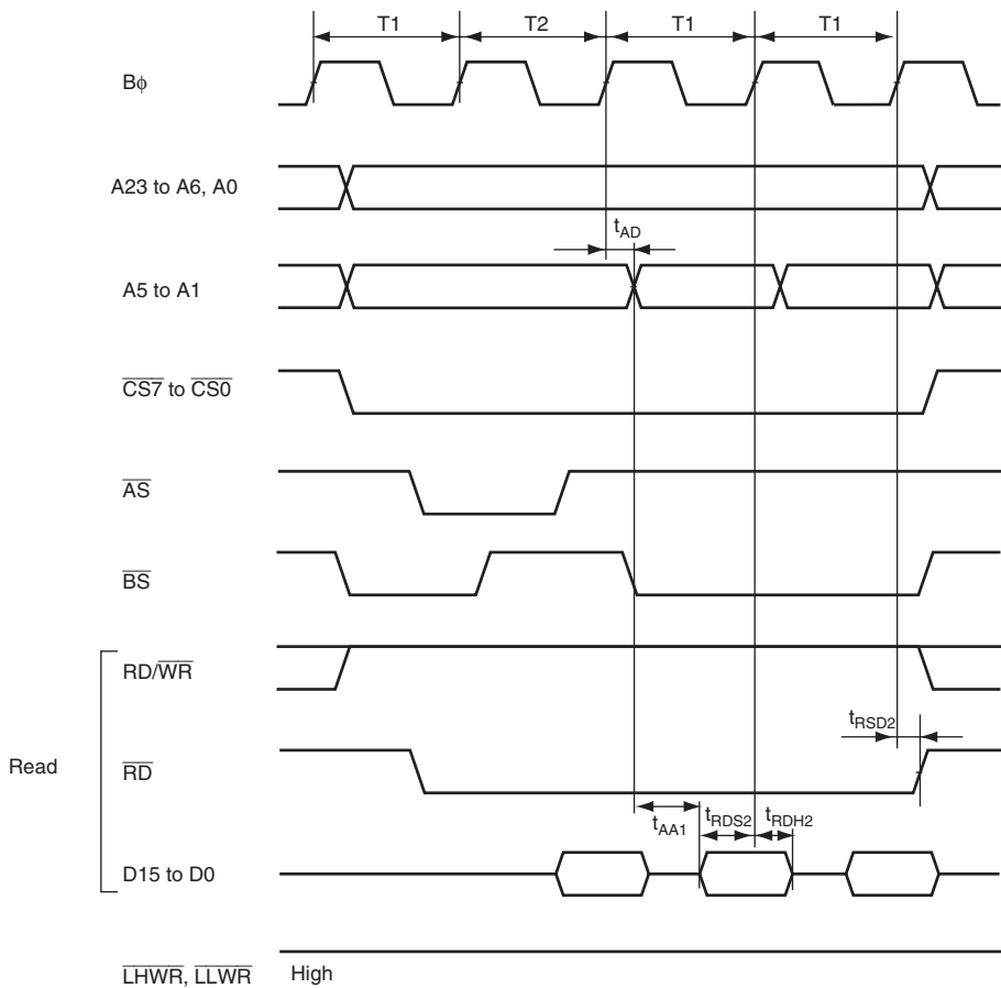
Figure 25.15 Burst ROM Access Timing: One-State Burst Access
