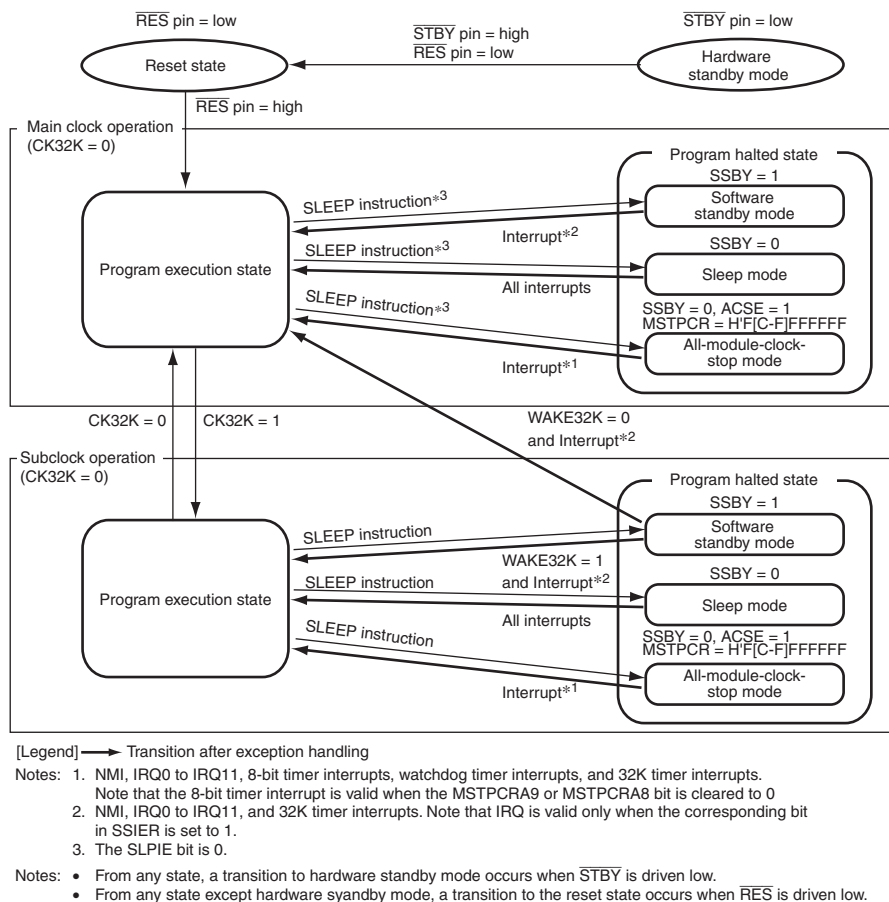
Figure 23.1 Mode Transitions
