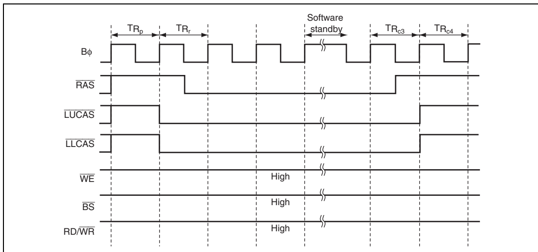
Figure 6.56 Self-Refresh Timing
