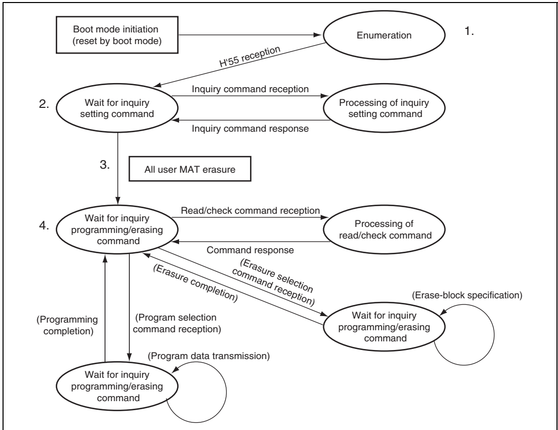
Figure 21.10 USB Boot Mode State Transition Diagram
