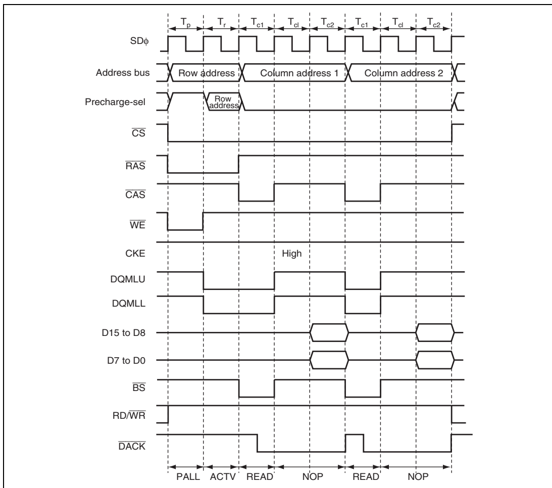
Figure 6.83 Output Timing Example of \overline{DACK} when DDS = 1 (Read, CAS Latency = 2)
