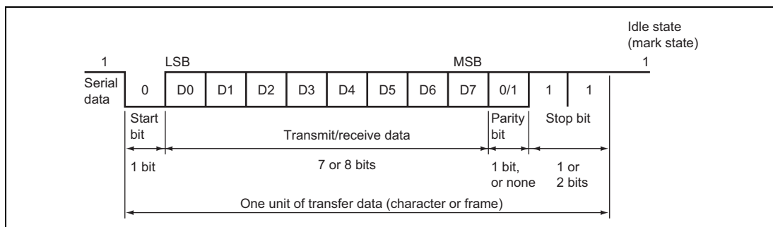
Figure 15.5 Data Format in Asynchronous Communication (Example with 8-Bit Data, Parity, Two Stop Bits)
