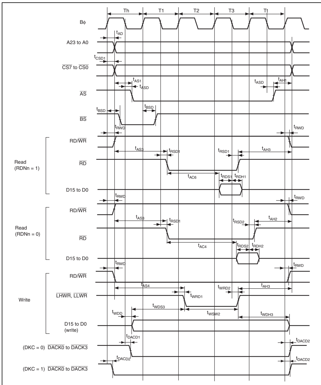
Figure 25.12 Basic Bus Timing: Three-State Access ( \overline{CS} Assertion Period Extended)
