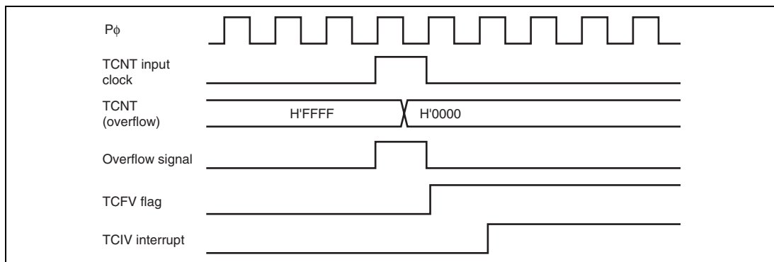
Figure 10.40 TCIV Interrupt Setting Timing
