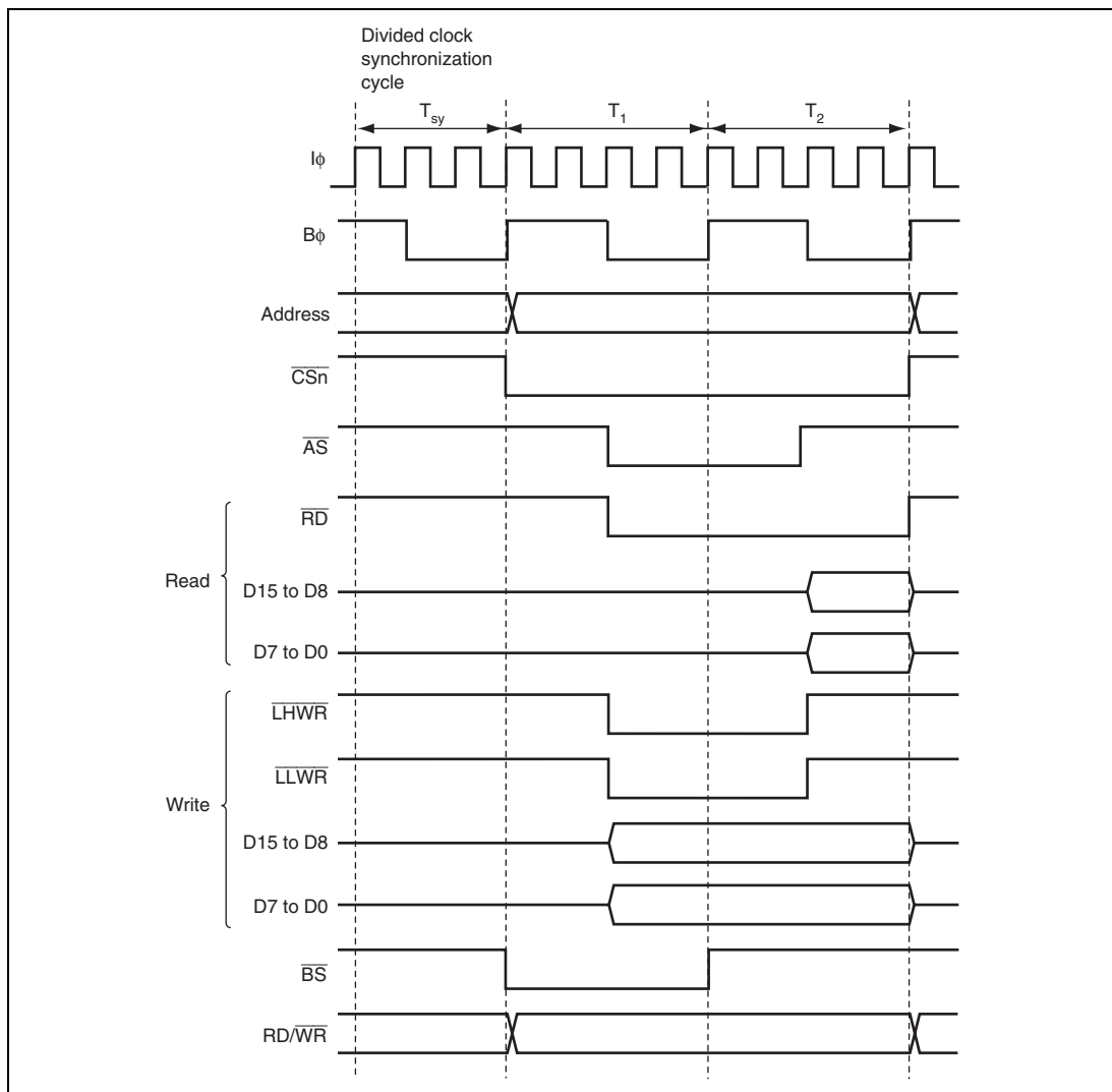
Figure 6.6 System Clock: External Bus Clock = 4:1, External 2-State Access
