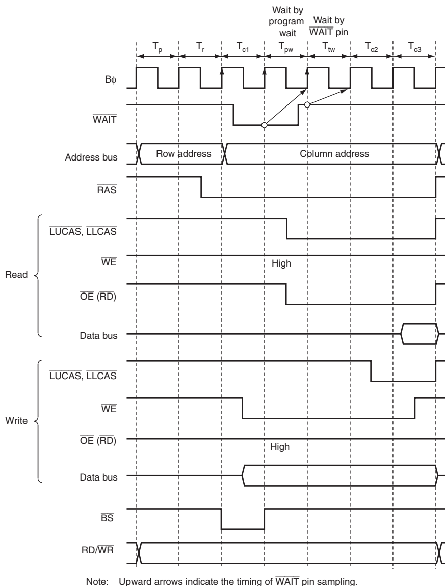
Figure 6.44 Example of Wait Cycle Insertion Timing for 3-Cycle Column Address Output
