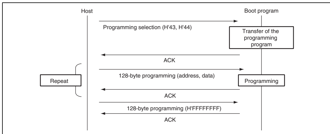
Figure 21.24 Programming Sequence
