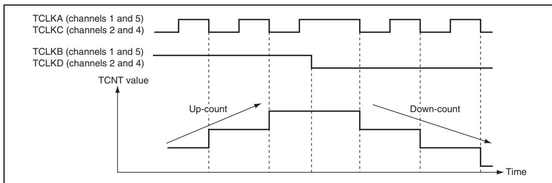
Figure 10.26 Example of Phase Counting Mode 2 Operation
