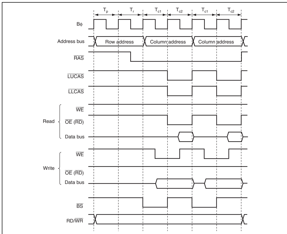
Figure 6.48 Operation Timing of Fast-Page Mode (RAST = 0, CAST = 0)
