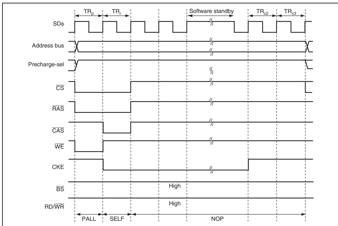
Figure 6.79 Self-Refresh Timing
