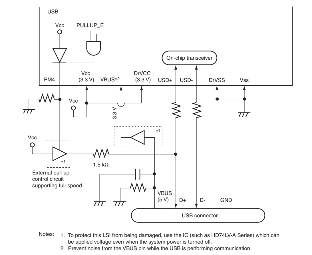
Figure 16.23 Example of Circuitry in Self Power Mode
