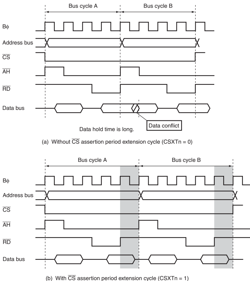
Figure 6.36 Consecutive Read Accesses to Same Area (Address/Data Multiplexed I/O Space)
