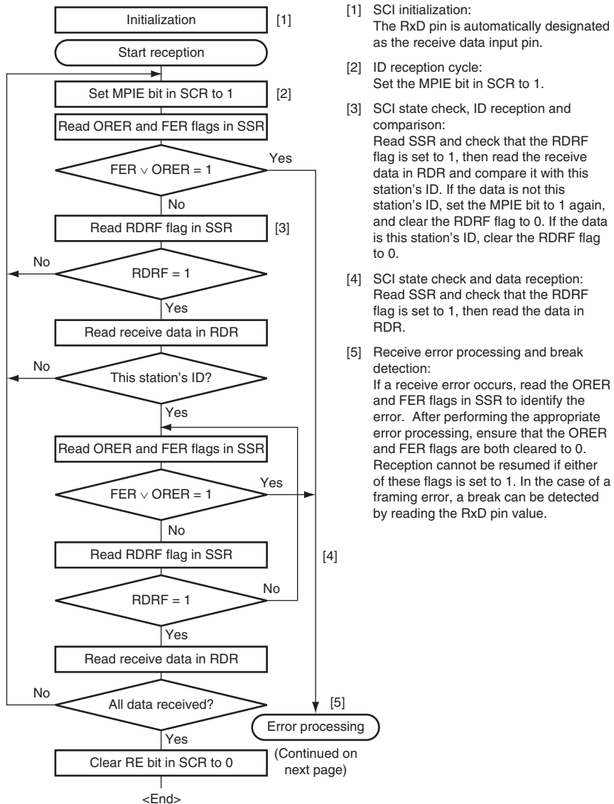
Figure 15.16 Sample Multiprocessor Serial Reception Flowchart (1)
