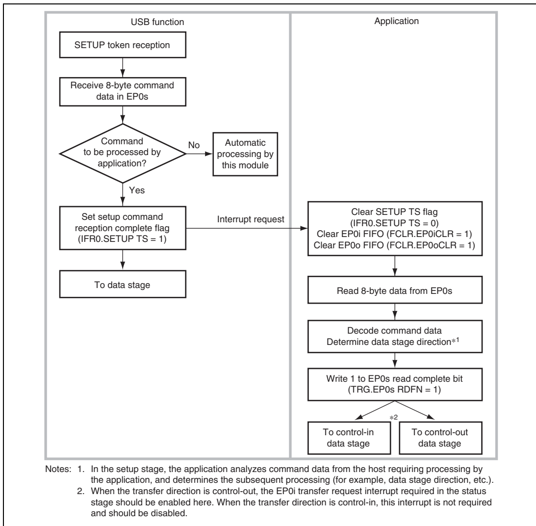
Figure 16.10 Setup Stage Operation
