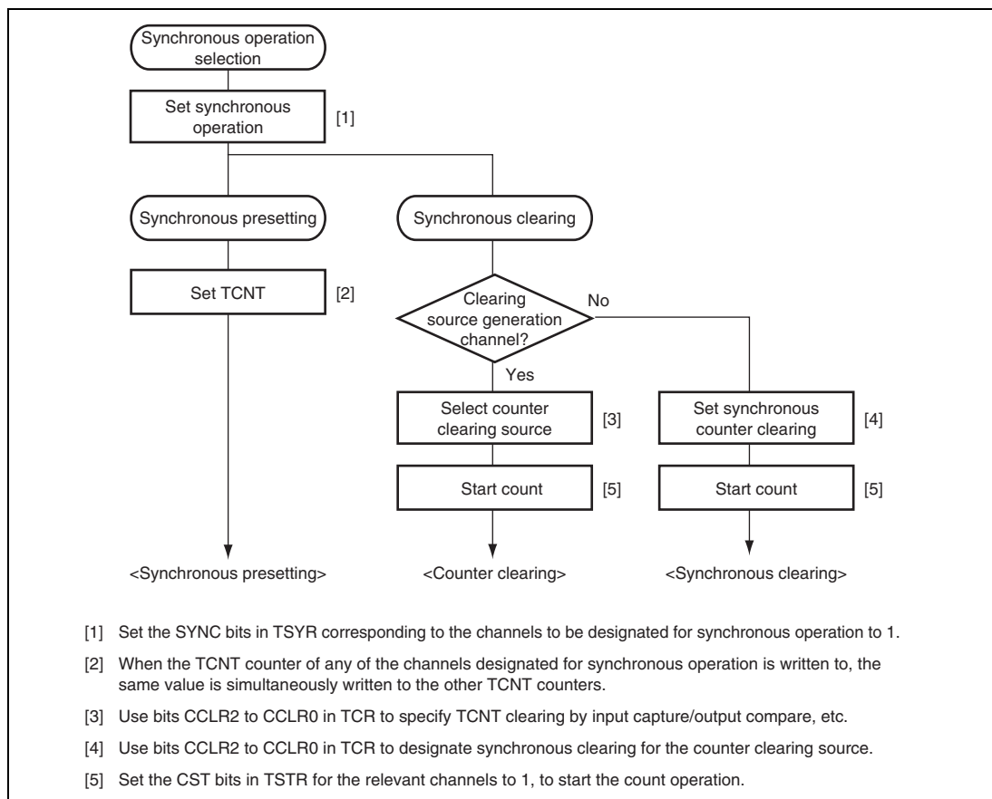
Figure 10.10 Example of Synchronous Operation Setting Procedure
