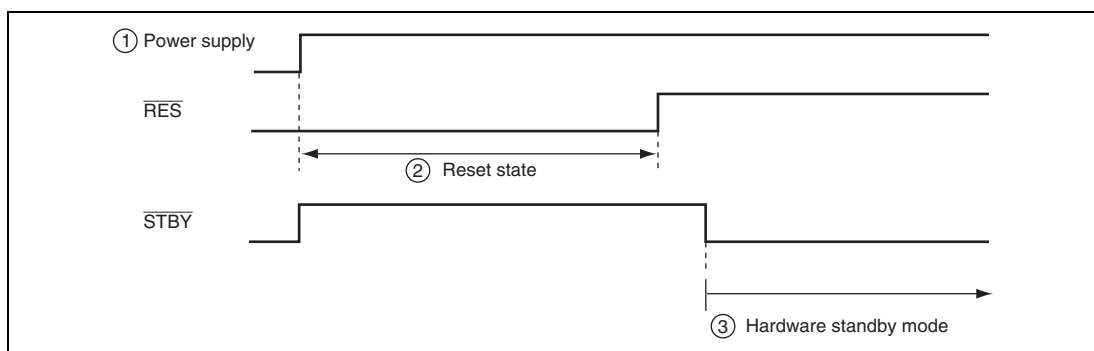
Figure 23.4 Timing Sequence at Power-On
