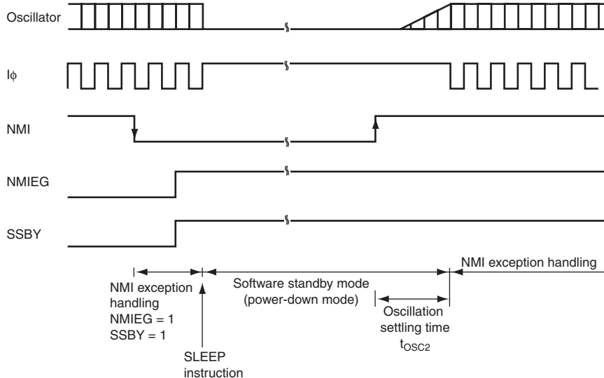
Figure 25.3 Oscillation Settling Timing after Software Standby Mode
