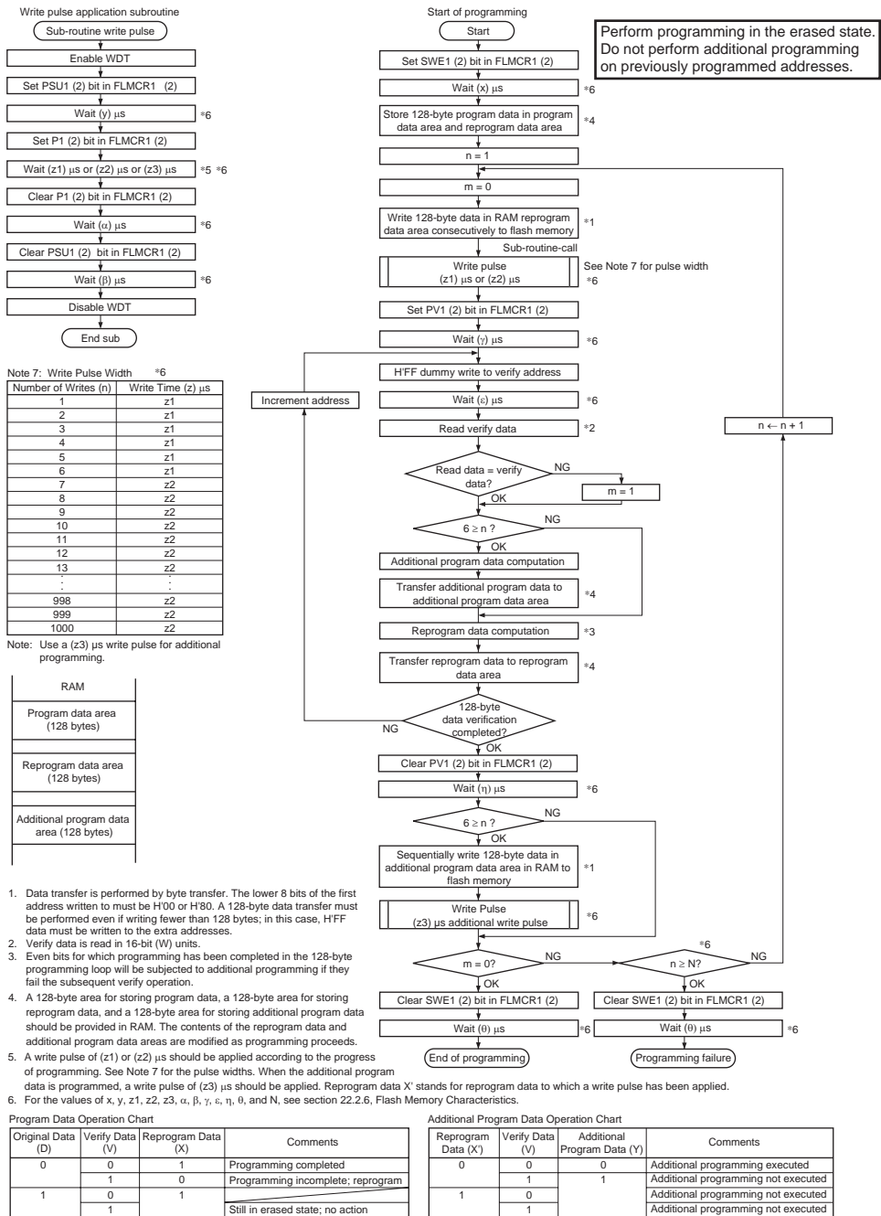
Figure 19.71 Program/Program-Verify Flowchart
