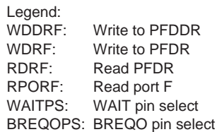
Figure C.12 (c) Port F Block Diagram (Pin PF 2 )
