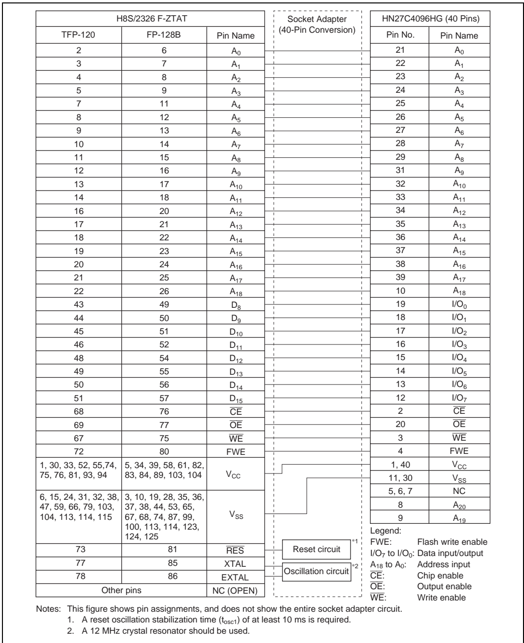
Figure 19.77 H8S/2326 F-ZTAT Socket Adapter Pin Assignments
