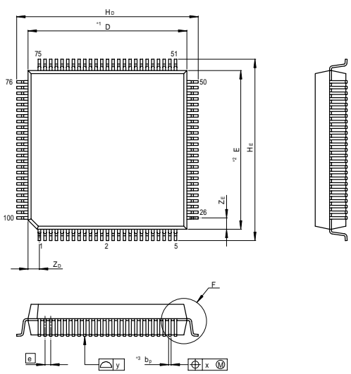
Figure F.2 FP-100B Package Dimensions
